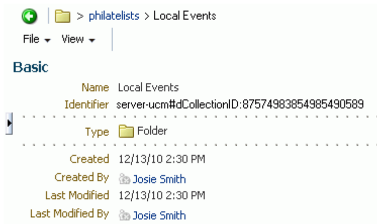
Figure 40–60 Folder Properties
