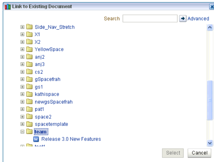
Figure 62–12 Existing Documents
