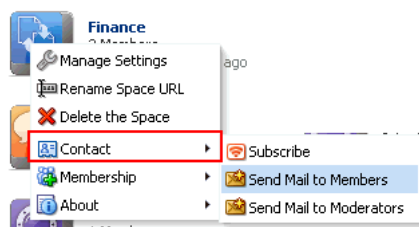
Figure 51-10 Actions Menu
