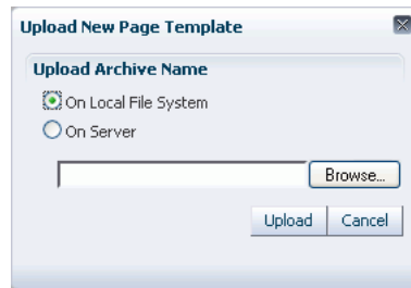
Figure 9–31 Upload Dialog
