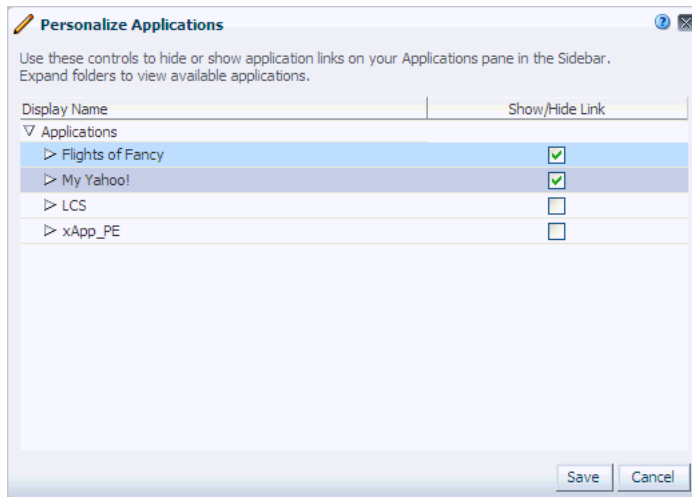
Figure 6–17 Personalize Applications
