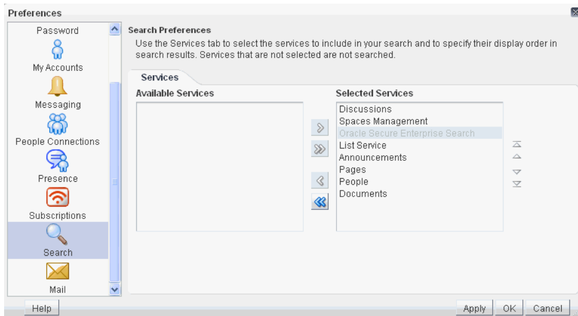
Figure 55–2 Search Preferences
