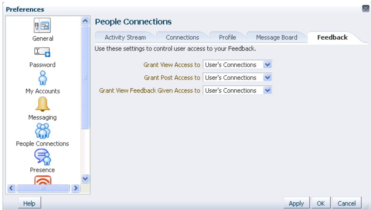
Figure 32–6 Feedback Preferences
