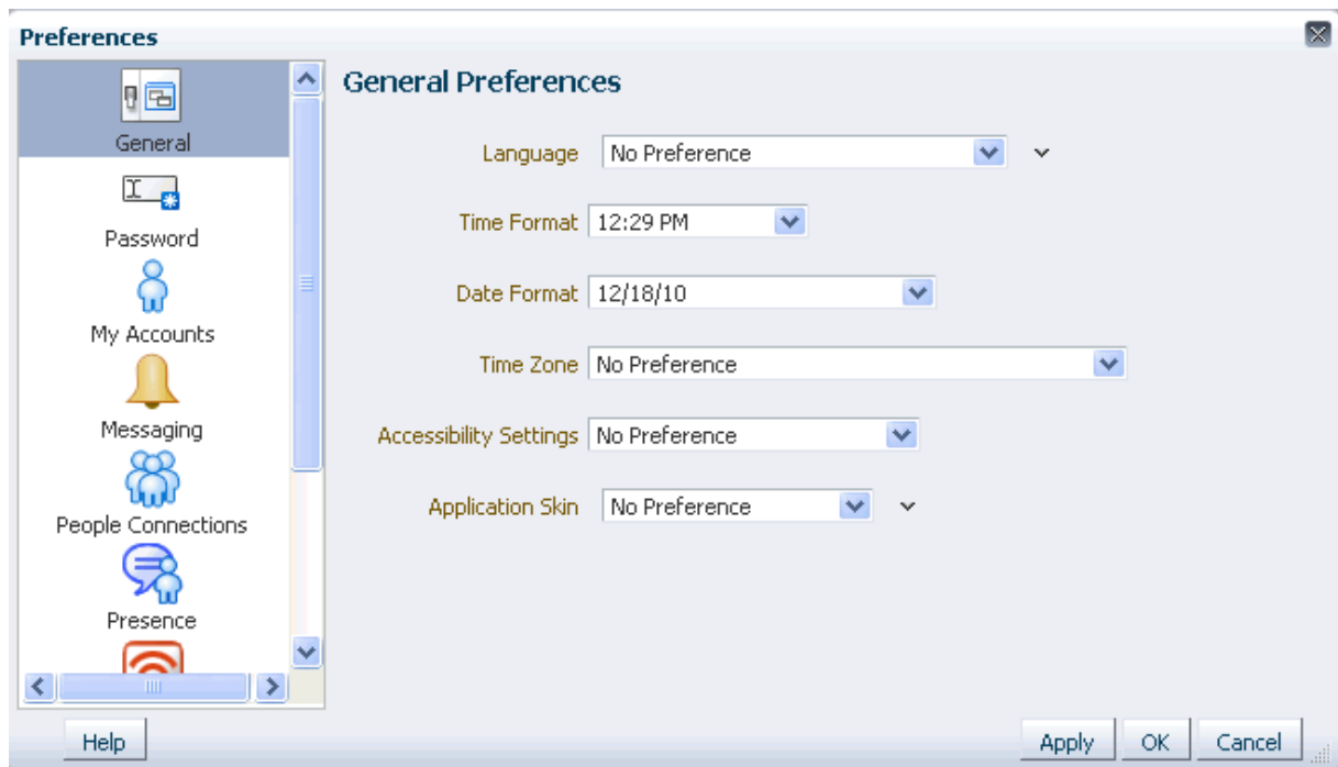
Figure 34-2 Preferences Dialog
