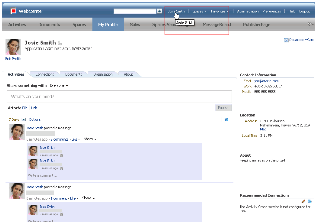
Figure 29–1 Profile Page
