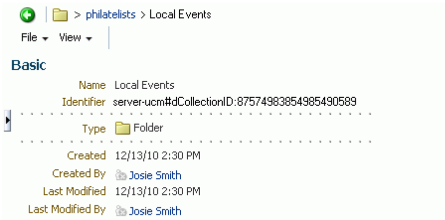
Figure 42–1 Folder Properties
