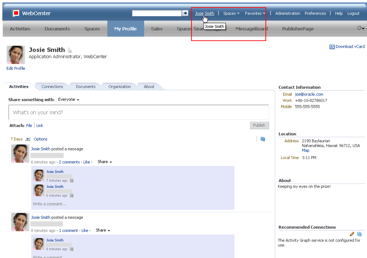
Figure 28–21 Profile Page
