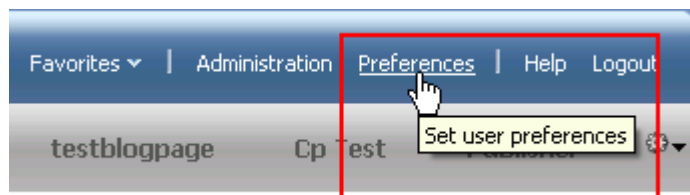
Figure 34-1 Preferences Link
