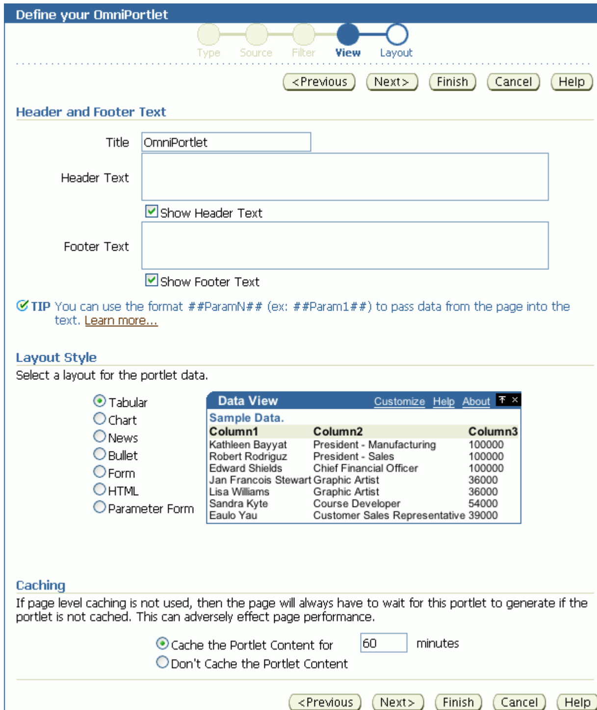
Figure 26–11 View Tab
