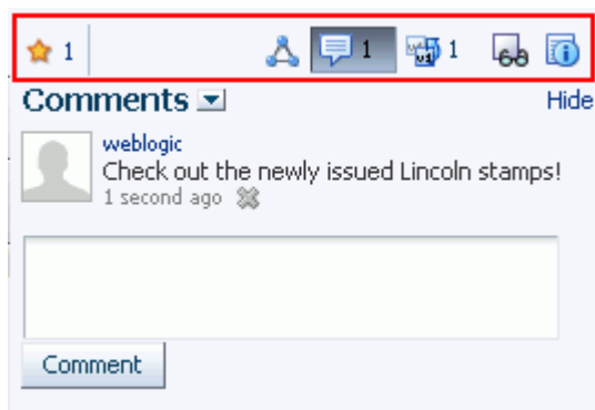
Figure 40–25 Sidebar Icons
