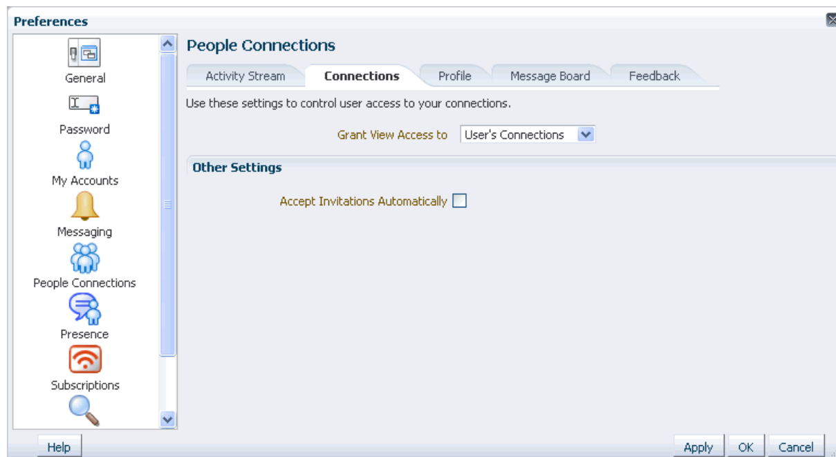
Figure 30–5 Connections Preferences
