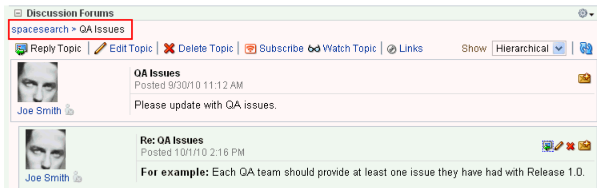
Figure 59–28 Forum Breadcrumbs
