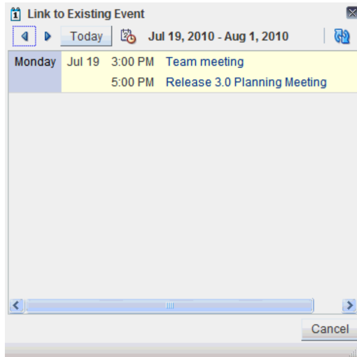
Figure 62–14 Existing Events
