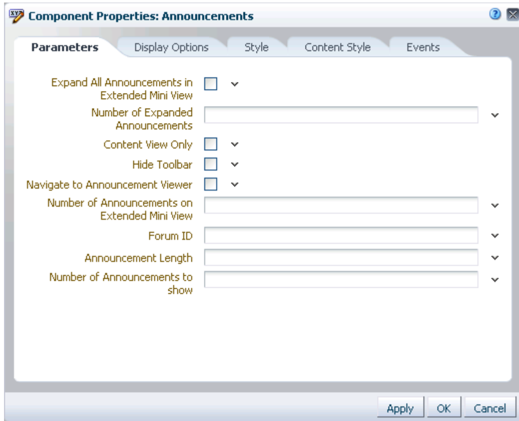
Figure 16-44 Component Parameters
