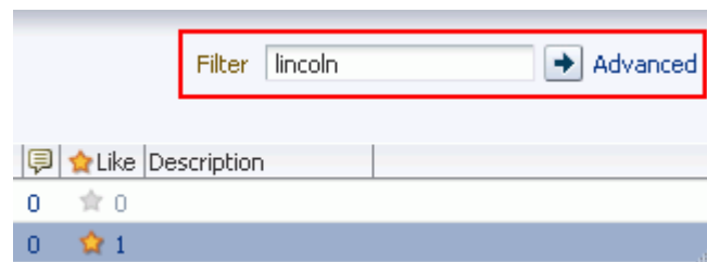
Figure 40–74 Filter Field
