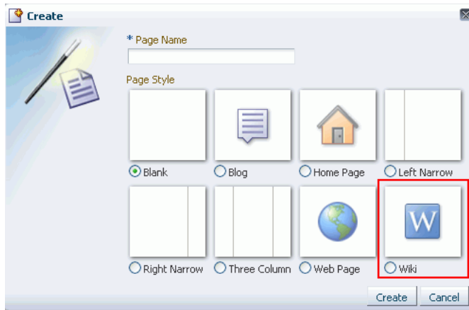
Figure 46–4 Create Dialog
