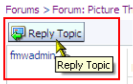
Figure 59–24 Reply Topic
