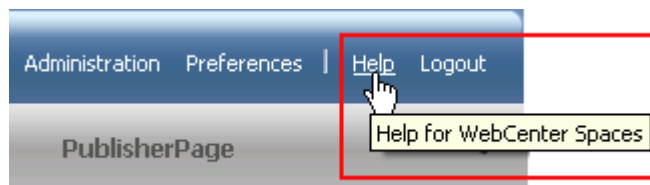
Figure 28–22 Help Link
