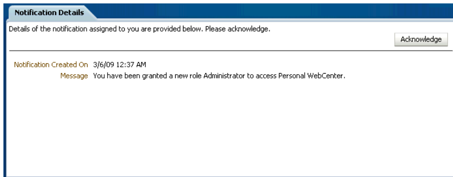
Figure 69–2 Worklist Notification
