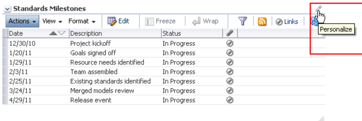
Figure 63–52 Personalize Icon
