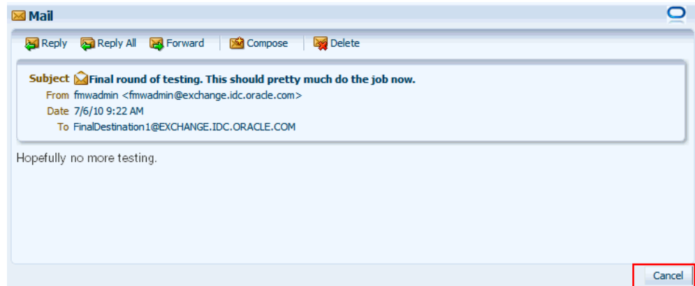
Figure 64–29 Cancel Message
