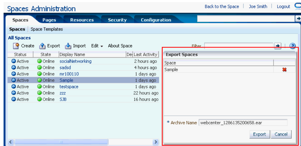
Figure 52–10 Exporting Spaces
