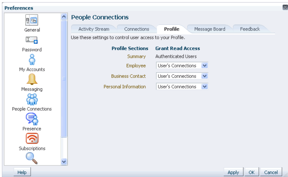
Figure 29-7 Profile Preferences
