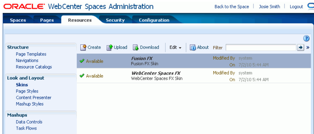
Figure 13–1 Built-in Skins
