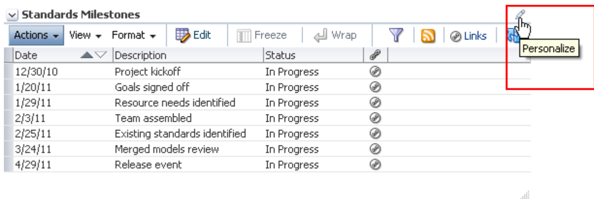
Figure 63–61 Personalize Icon
