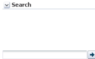
Figure 12–35 Search Component
