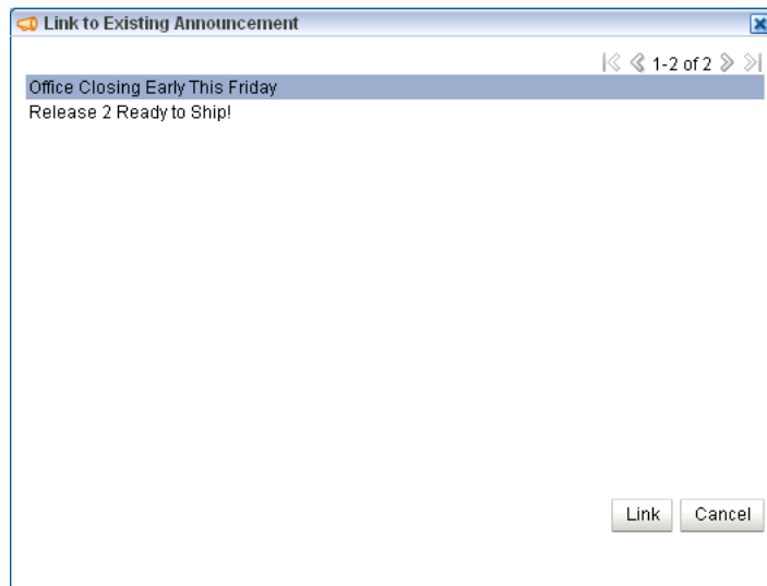
Figure 62–8 Existing Announcements
