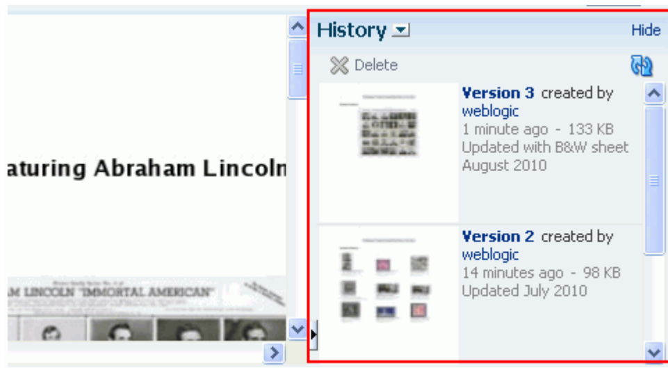
Figure 40-57 History Pane
