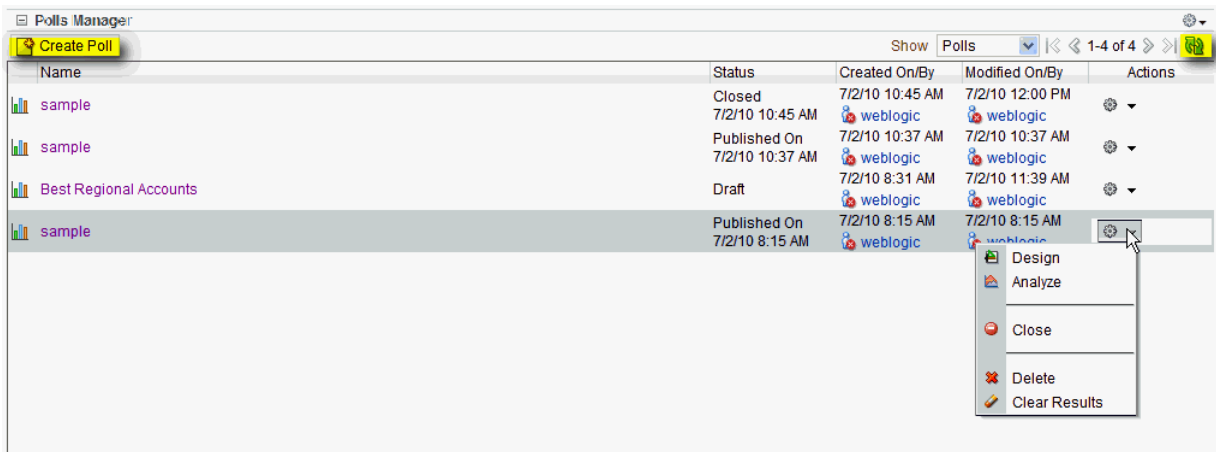
Figure 66–5 Polls Manager
