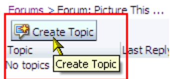
Figure 59–20 Create Topic
