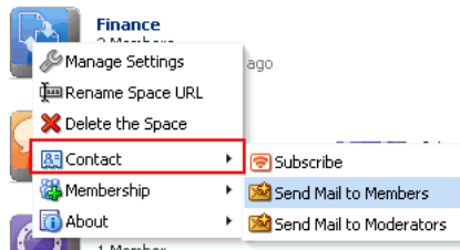
Figure 51-11 Actions Menu
