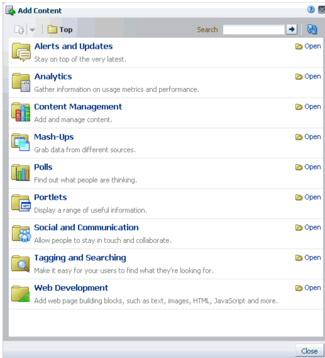
Figure 16–10 Resource Catalog
