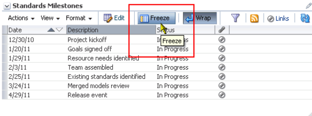
Figure 63–47 Freeze Icon
