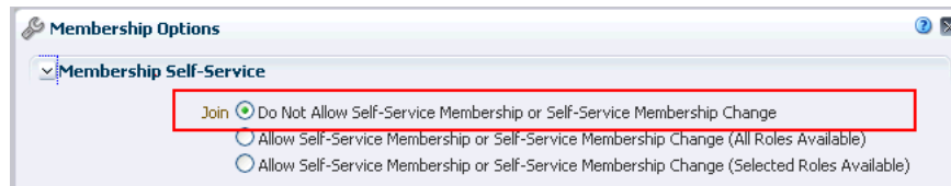
Figure 51-1 Disabling Self-Service
