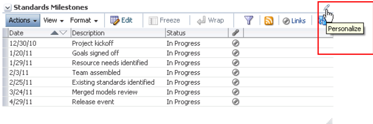
Figure 63–58 Personalize Icon
