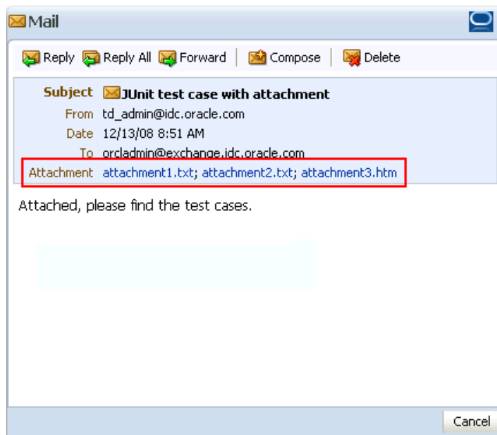
Figure 64–14 Mail Attachments
