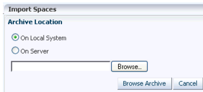
Figure 52–13 Importing Spaces
