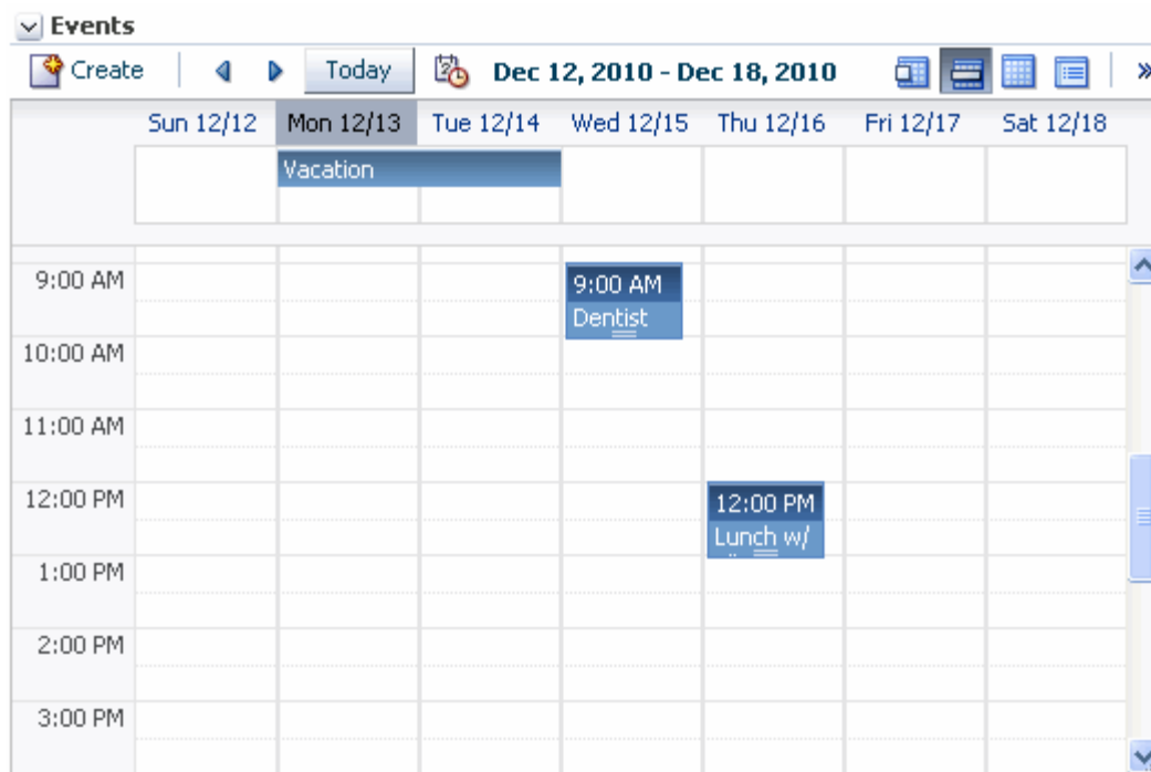
Figure 60–4 Personal Calendar
