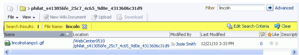
Figure 40–75 Search Results
