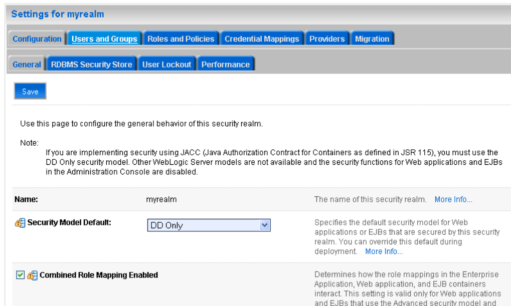
Figure 30-3 Settings Pane
