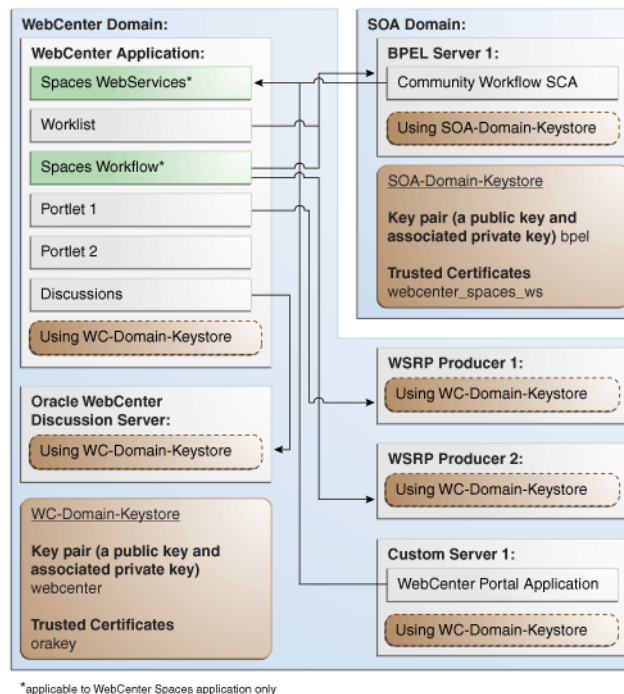
Figure 32-10 WS-Security for a Typical Configuration
