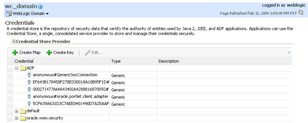
Figure 33–6 Credentials Pane
