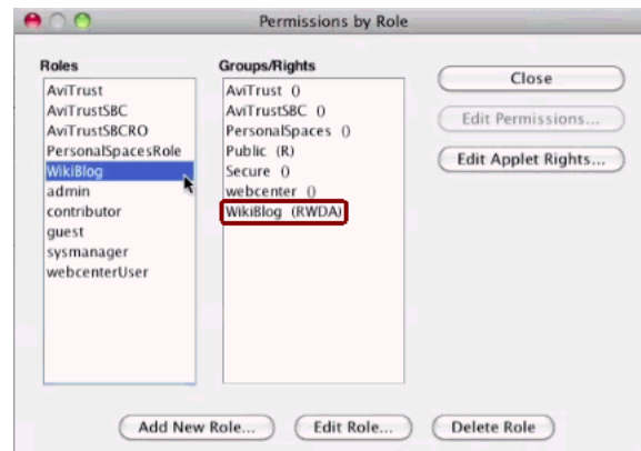
Figure 11–7 RWDA Permissions
