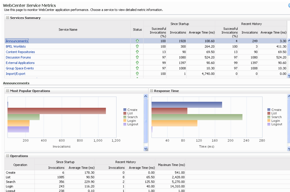
Figure 36–1 Announcement Metrics
