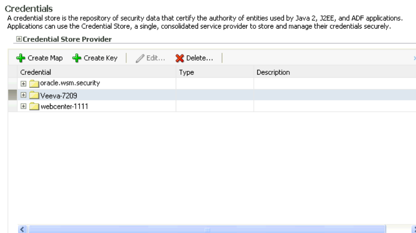
Figure 7-18 Credentials Pane
