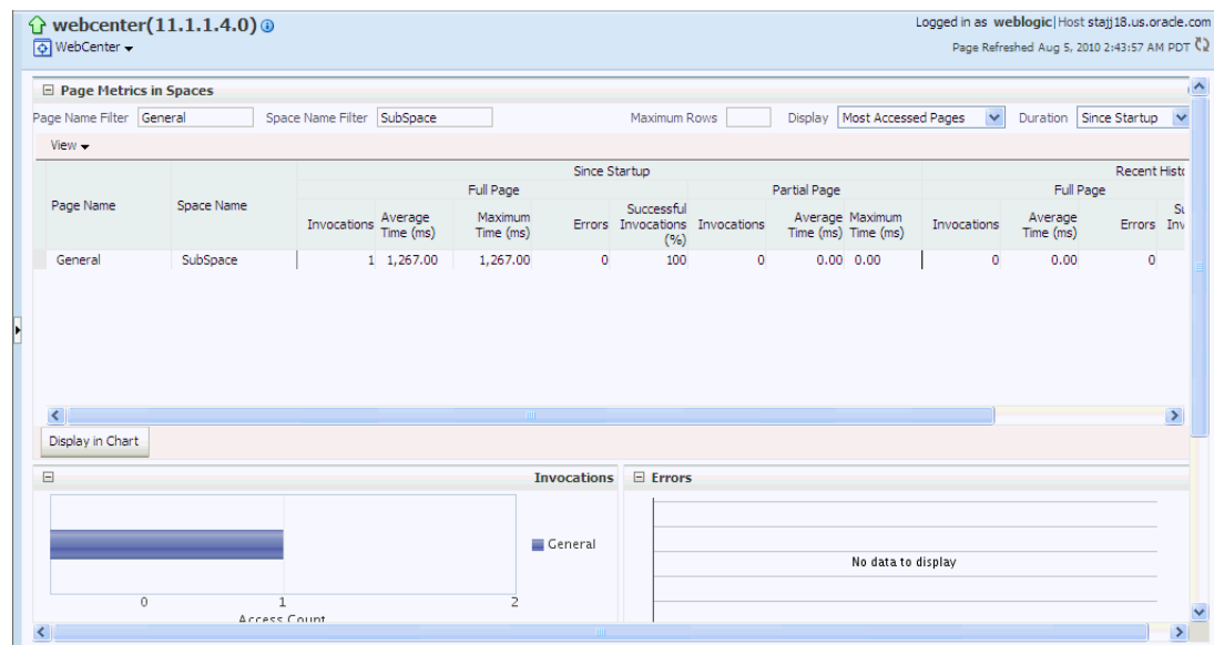
Figure 36–27 Space Metrics
