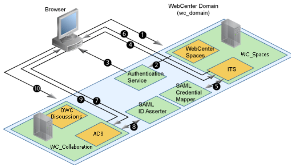
Figure 30–22 SAML Single Sign-on Components and Topology (POST Profile Configured)
