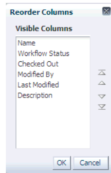
Figure 34-42 Columns - Reorder
