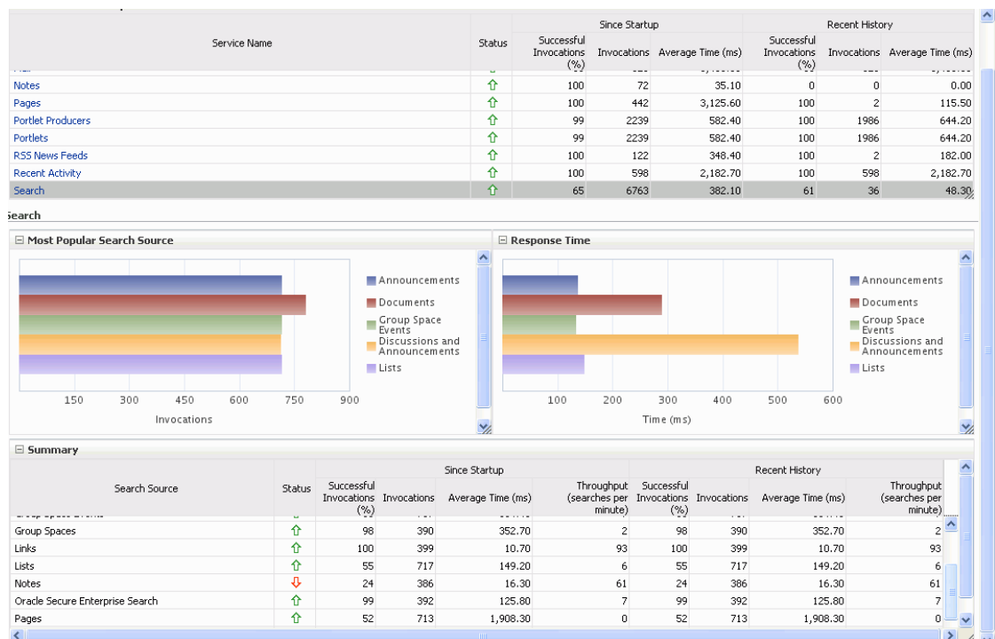
Figure 36–21 Search Metrics
