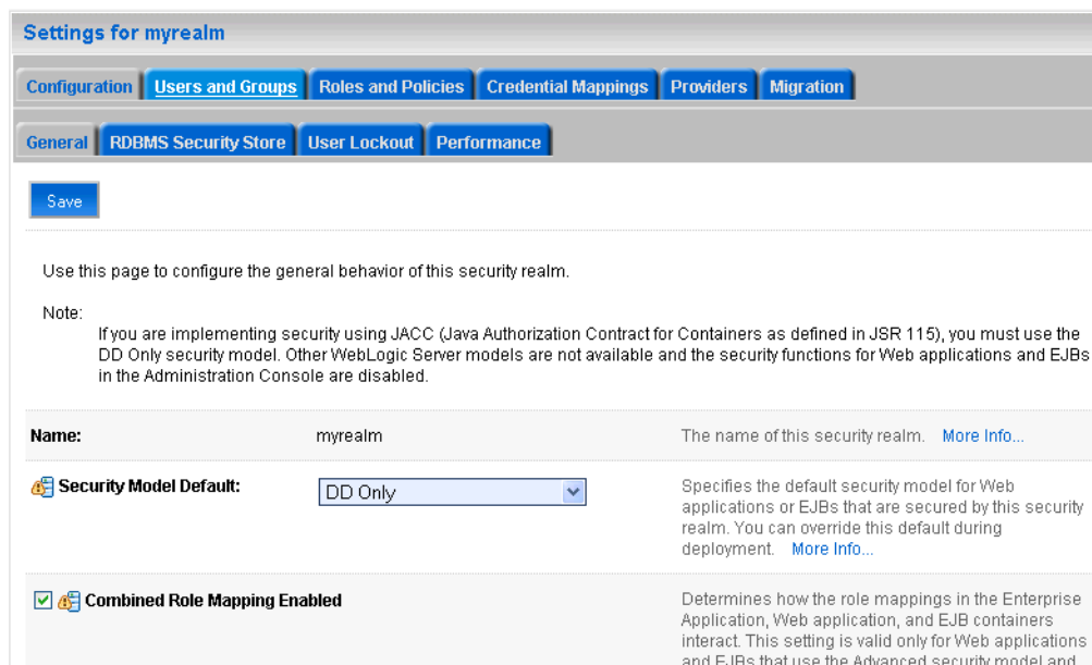
Figure 30–18 Settings Pane
