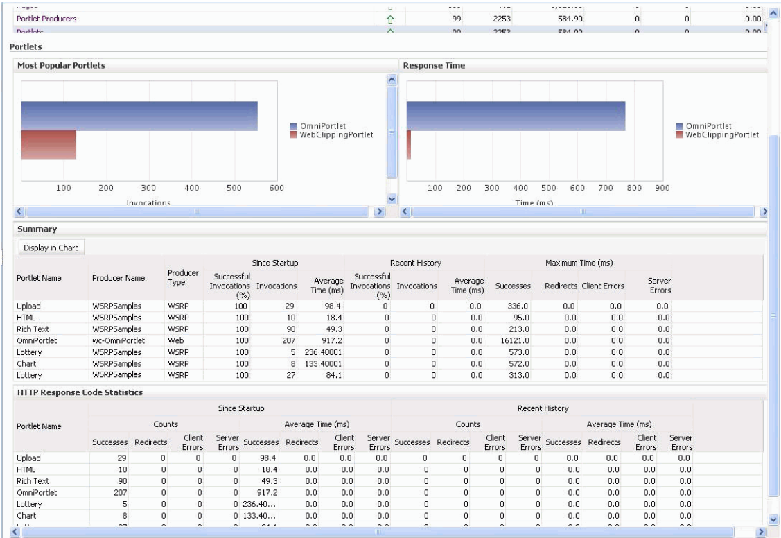
Figure 36–16 Portlet Metrics
