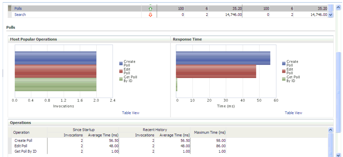
Figure 36–18 Poll Metrics
