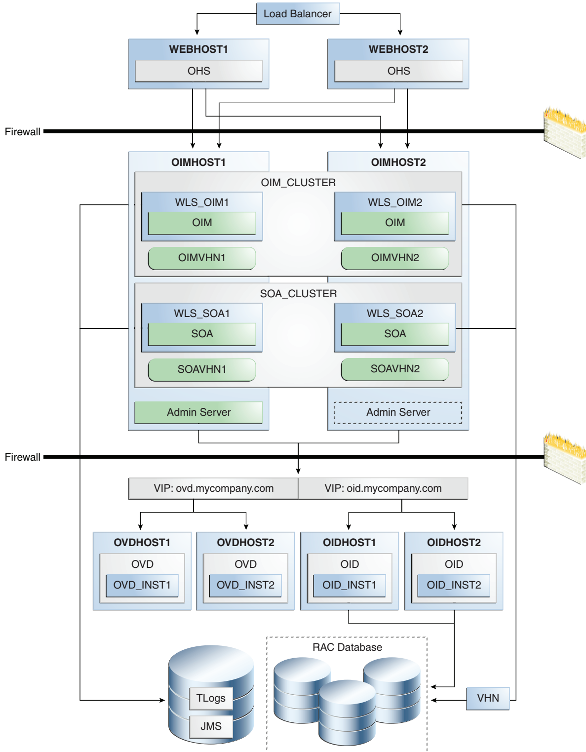
Figure 8–15 Oracle Identity Manager High Availability Architecture
