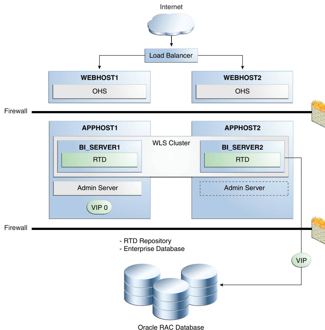
Figure 15-14 Oracle RTD High Availability Architecture
