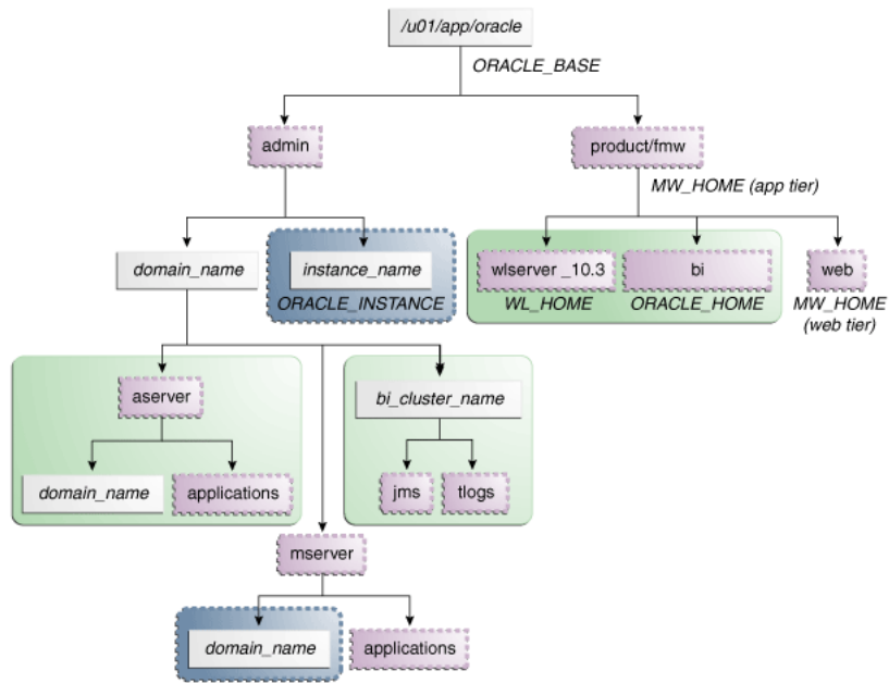
Figure 2–2 EDG Directory Structure for Oracle Business Intelligence
