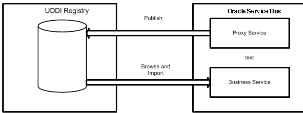
Figure 41–1 Oracle Service Bus integration with UDDI
