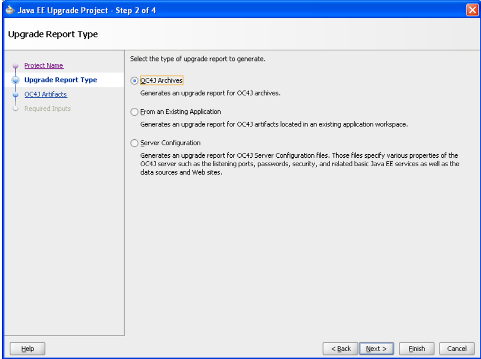
Figure 2-3 Java EE Upgrade Application Wizard - Upgrade Report Type Page
