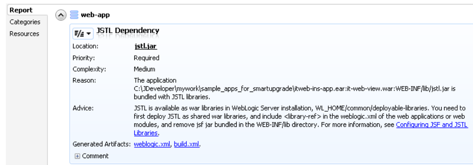
Figure 2–9 Sample Finding in a SmartUpgrade Report
