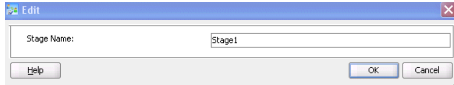
Figure 28–21 Edit Dialog
