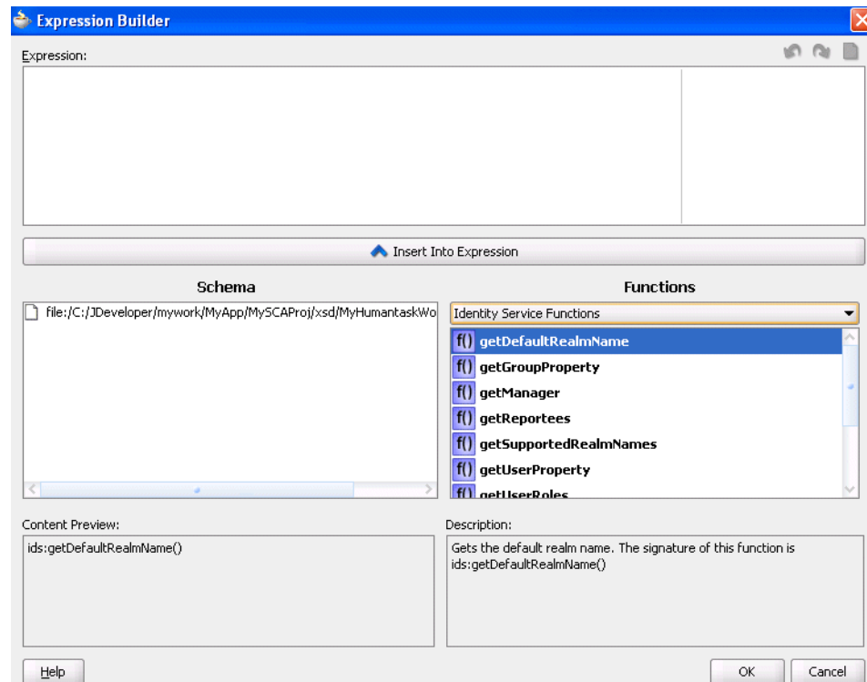
Figure 28–16 Expression Builder
