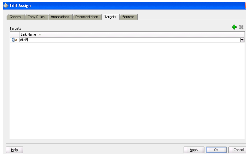
Figure 9-7 Target Activity
