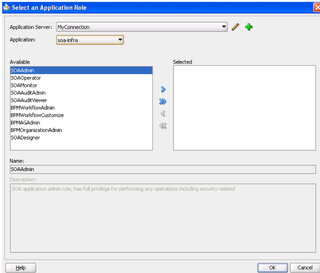
Figure 28–14 Application Role
