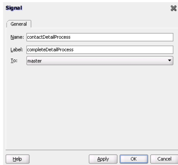
Figure 15–7 Signal Dialog
