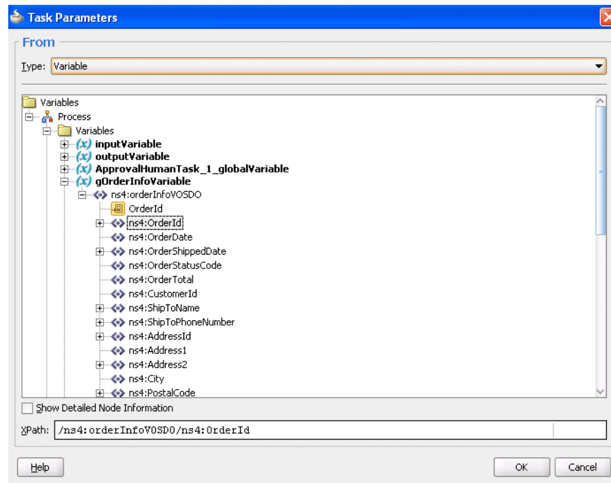
Figure 28–74 Variables Tree
