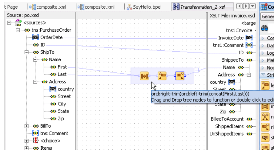
Figure 38–20 Chaining Functions
