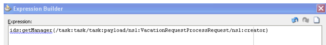
Figure 27–13 XPath Expression
