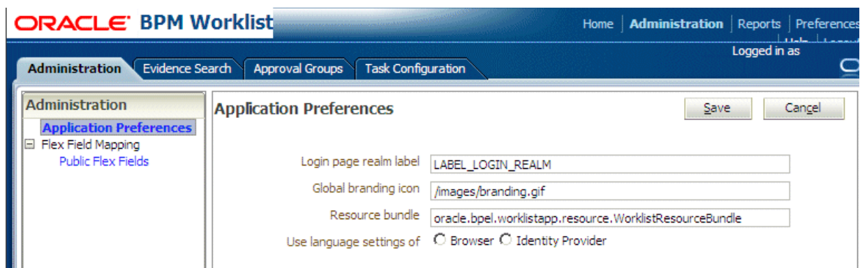
Figure 30–43 Application Preferences
