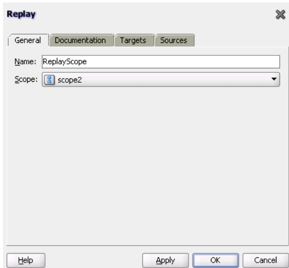
Figure 11–13 Replay Dialog
