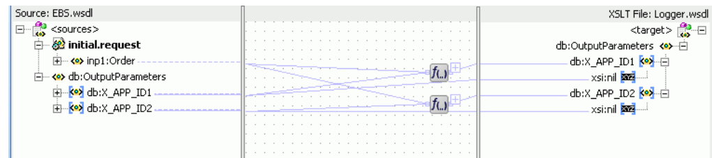
Figure 46–60 EBS_TO_COMMON_INSERT.xsl Transformation
