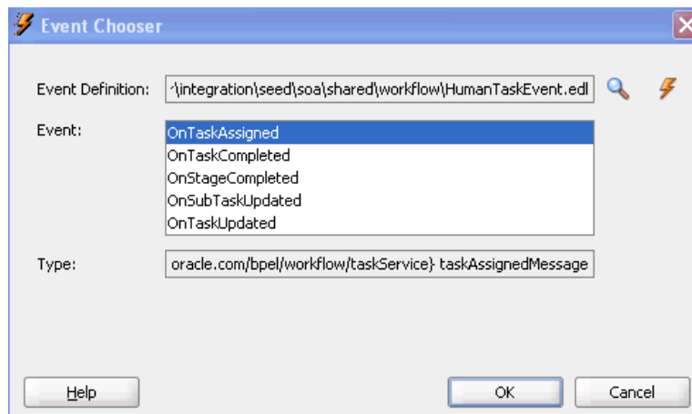
Figure 28–69 Event Callbacks
