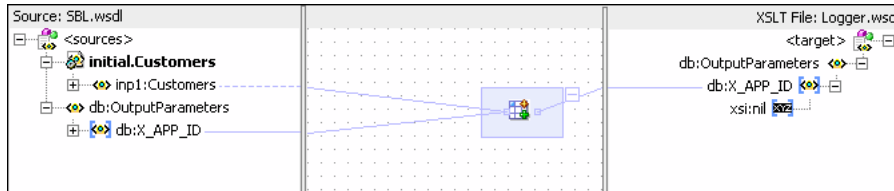
Figure 46–36 SBL_TO_COMMON_INSERT.xml Transformation
