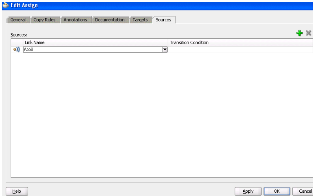
Figure 9–6 Source Activity
