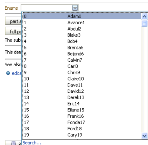
Figure 11-6 InputComboboxListOfValues Displays a List of Employee Names
