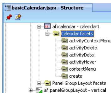
Figure 15–6 Calendar Facets in the Structure Window
