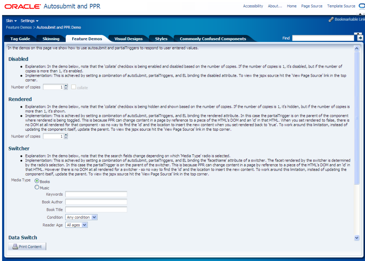
Figure 1–4 Framework Demonstration
