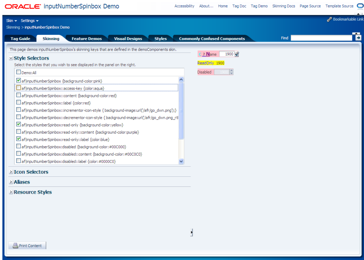
Figure 1–2 Skinning Demonstration
