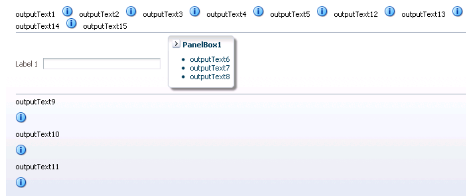
Figure 8–49 panelGroupLayout Arrangements
