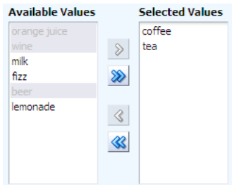
Figure 9–26 selectManyShuttle component
