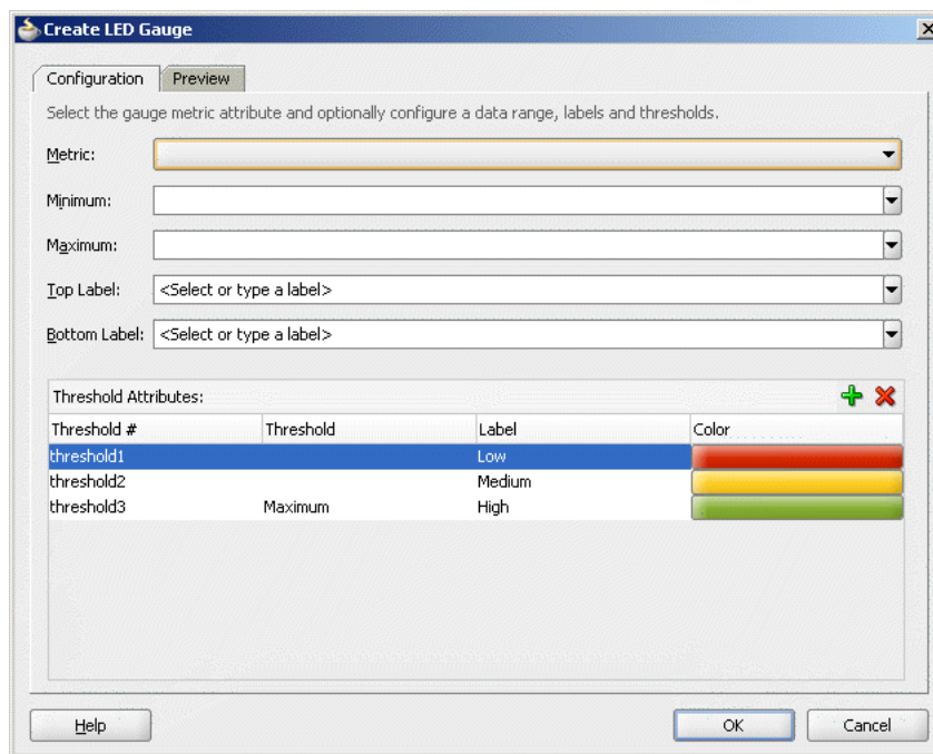
Figure 25–8 Create Gauge Dialog
