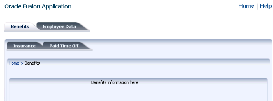
Figure 18–6 First-Level Page
