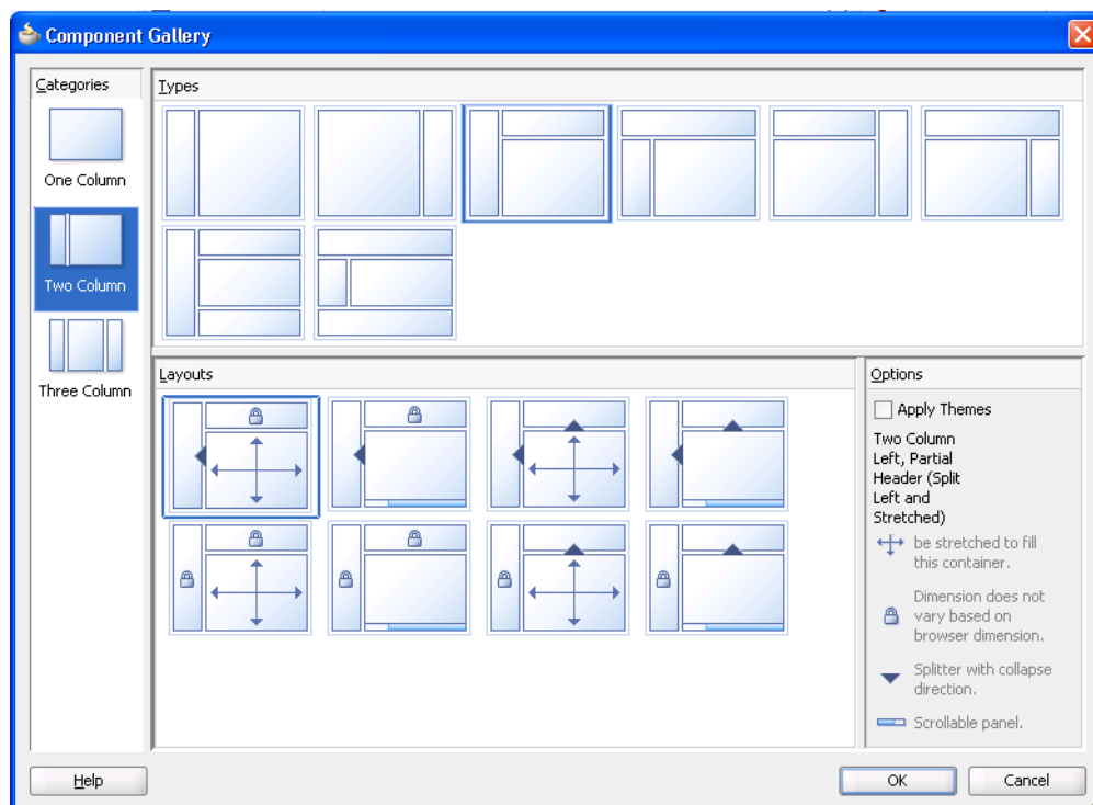
Figure 8-5 Quick Layouts
