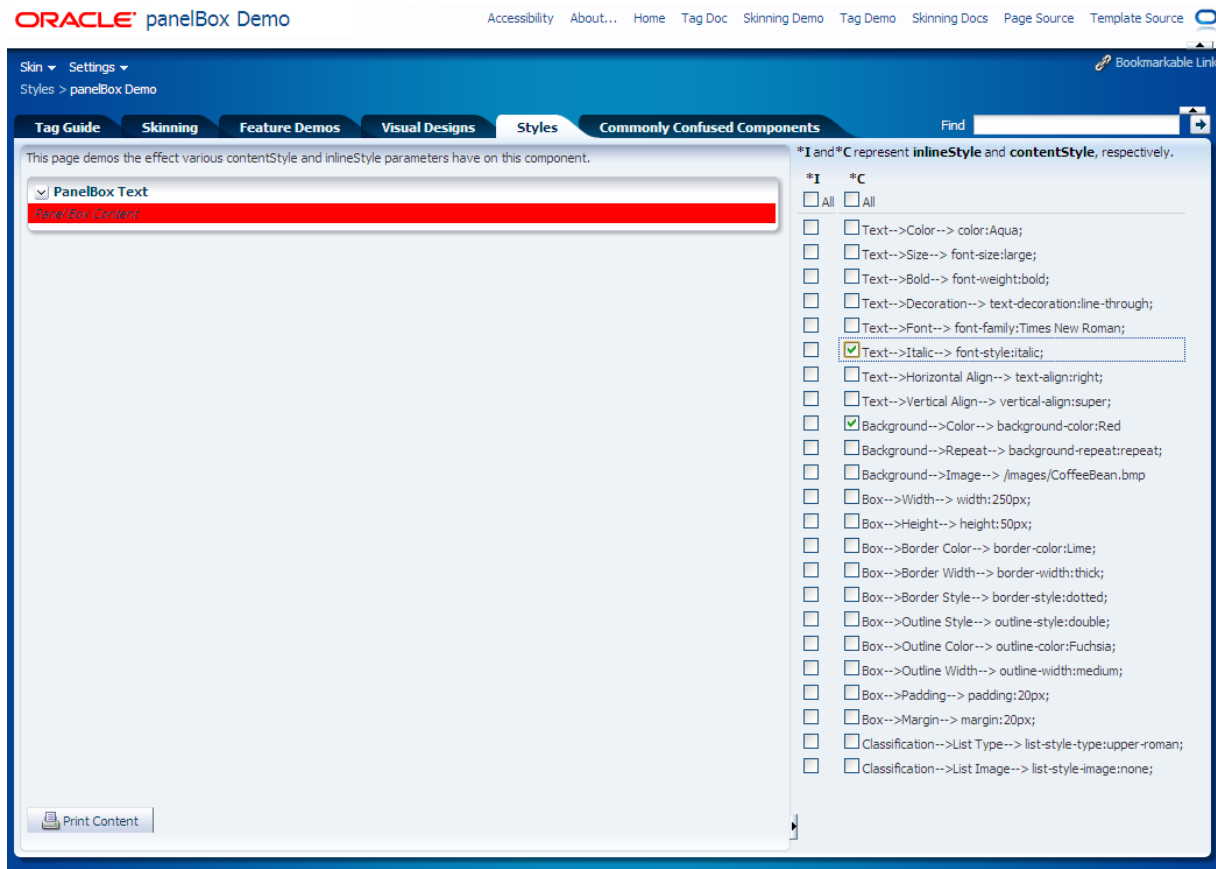
Figure 1–6 Styles Demonstration
