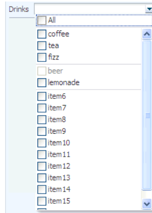
Figure 9–25 selectManyChoice Component
