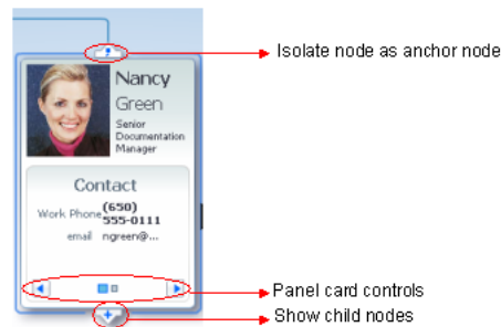
Figure 29–6 Node Controls
