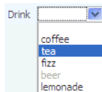
Figure 9–22 selectOneChoice Component
