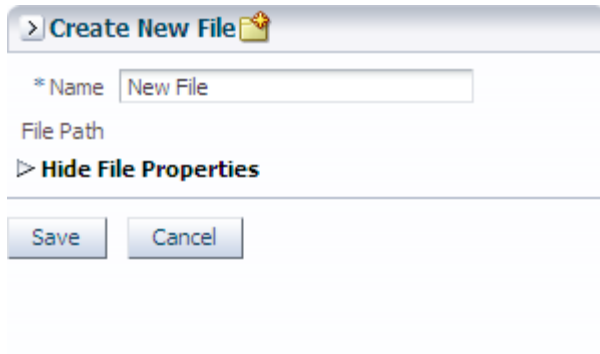
Figure 8–24 Collapsed showDetail
