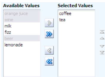
Figure 9–27 selectOrderShuttle Component
