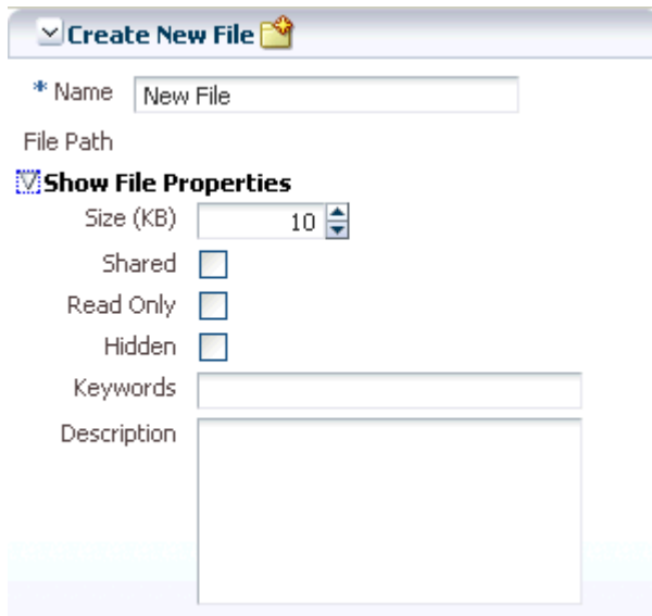
Figure 8–25 Expanded showDetail
