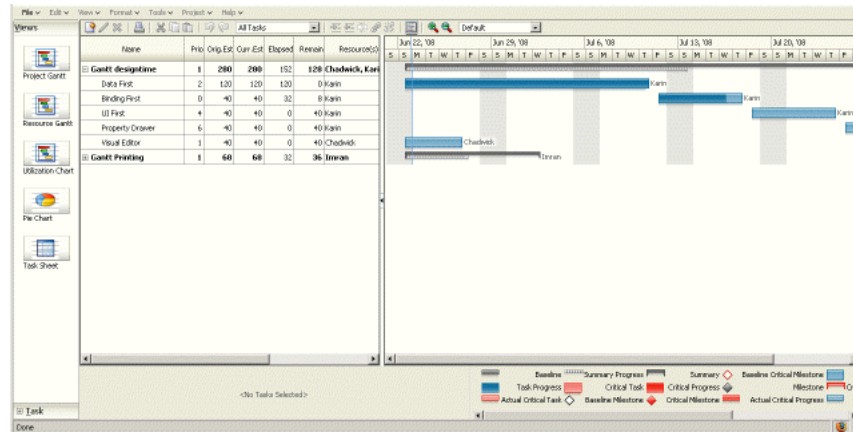
Figure 23–11 Project Gantt
