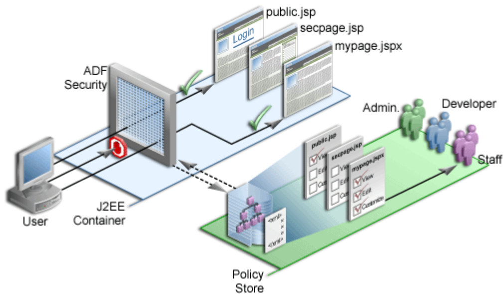
Figure 30–27 ADF Security Authorization
