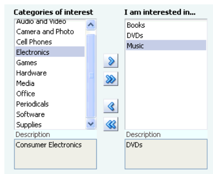
Figure 25–7 SelectManyShuttle Component
