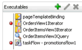
Figure 31–21 ADF Declarative Breakpoints Enabled in the Page Definition Executables
