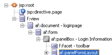
Figure 30–19 Login Page Structure with Panel Form Layout
