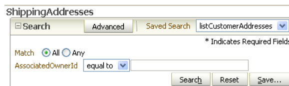
Figure 27–14 Query Search Form with Named Bind Variable
