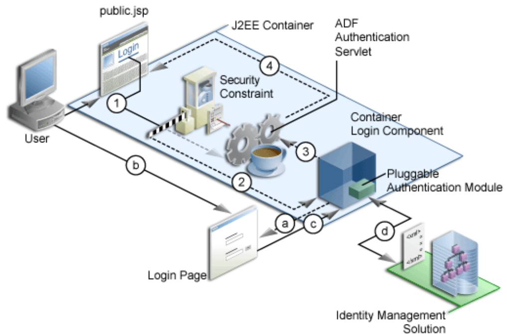
Figure 30–26 ADF Security Explicit Authentication
