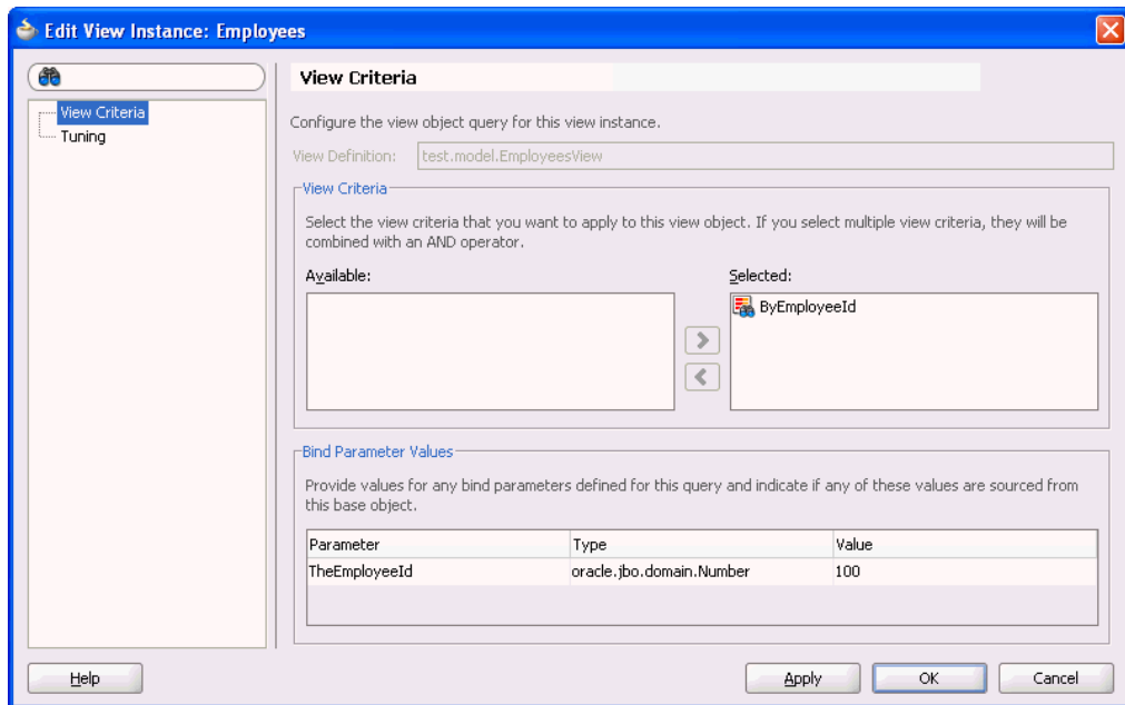
Figure 5–32 View Criteria Filters View Instance
