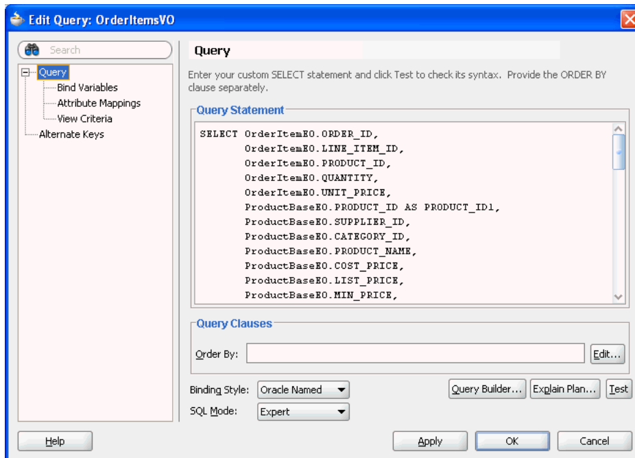
Figure 5–37 OrderItems Expert Mode View Object
