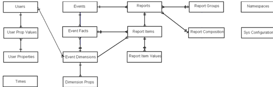
Figure I-1 Analytics Database Model
