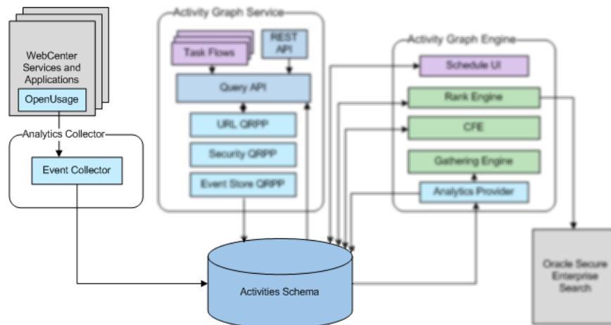
Figure 45–2 Data Collection by Oracle WebCenter Analytics
