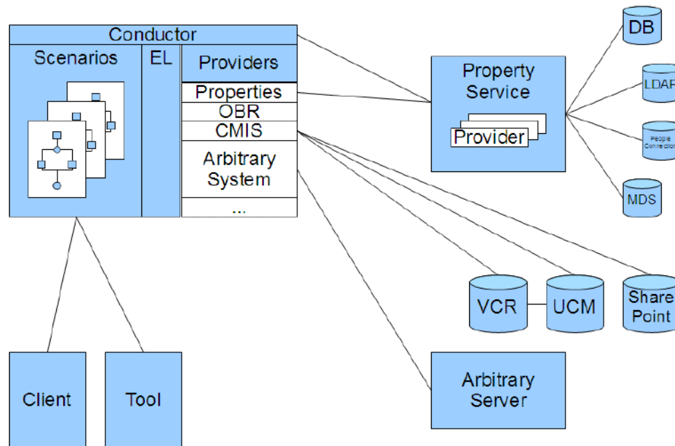
Figure 66–1 WebCenter Personalization Services Architecture
