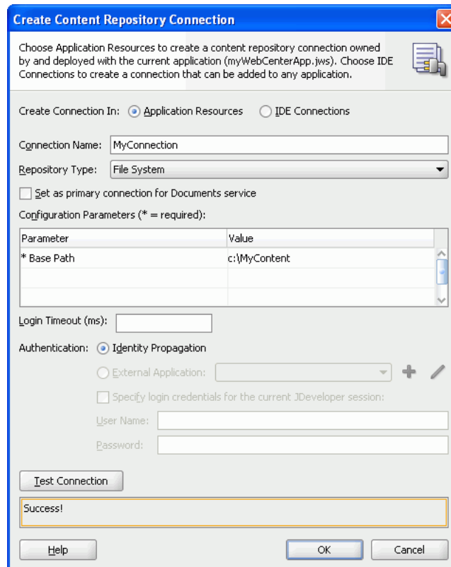
Figure 26–8 File System Connection
