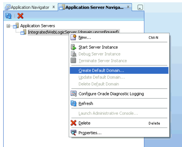
Figure 66–17 Application Server Navigator - Creating the Default Domain
