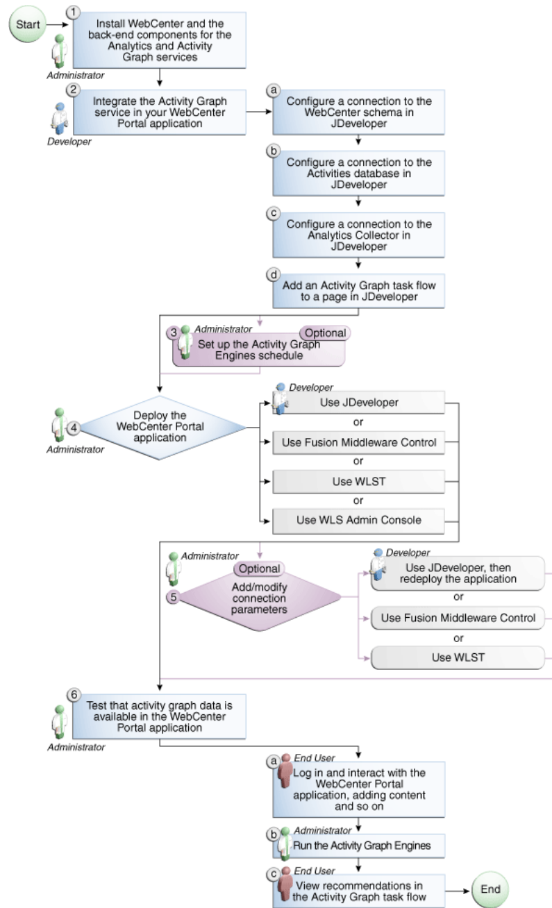
Figure 45–5 Configuring the Activity Graph Service for WebCenter Portal Applications
