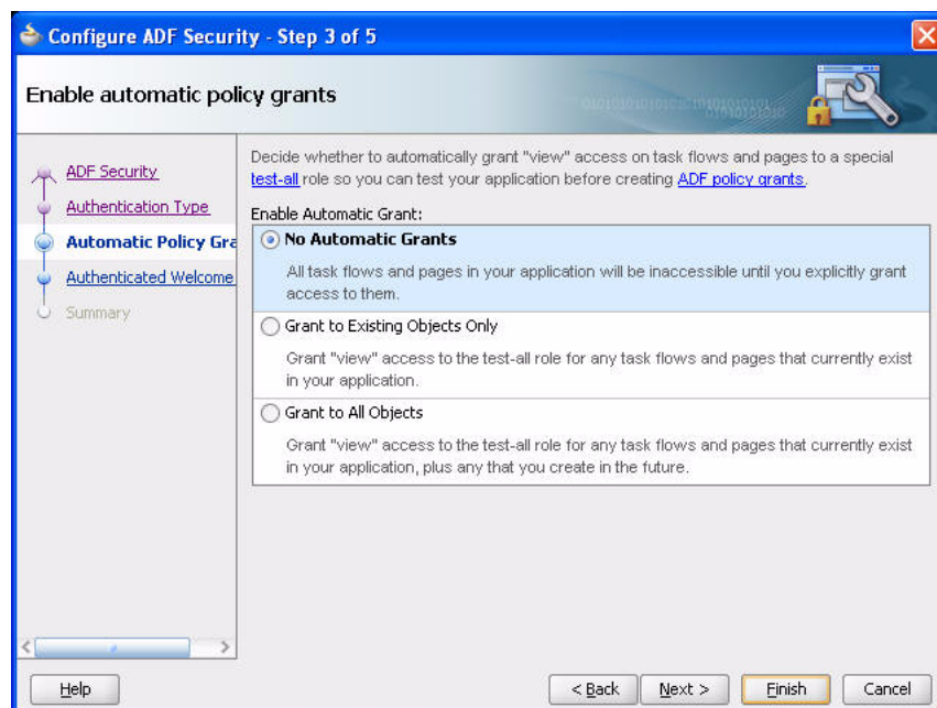
Figure 67–3 Automatic Policy Grants Page
