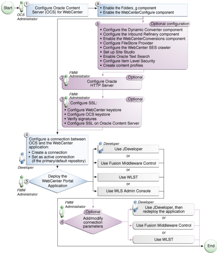
Figure 26-1 Configuring Oracle Content Server for WebCenter Portal Applications
