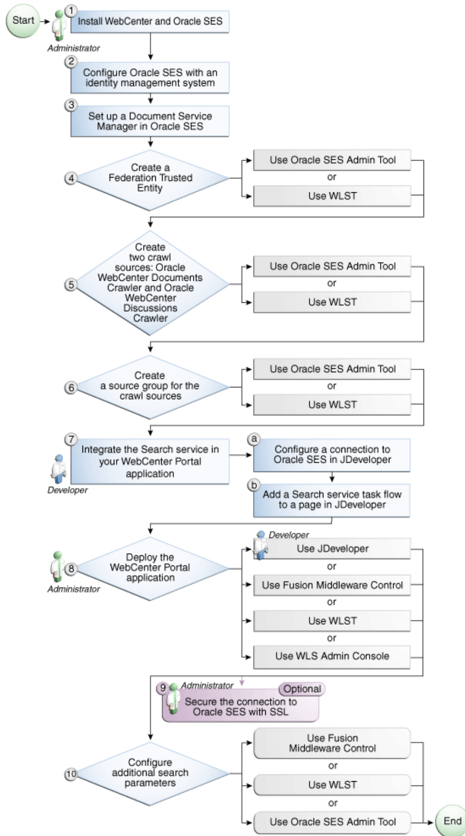
Figure 44–1 Configuring Oracle SES for WebCenter Portal Applications
