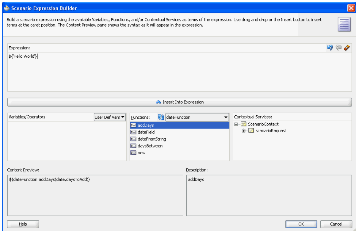
Figure 66-24 Scenario Expression Builder
