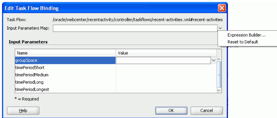
Figure 49–4 Example of the Edit Task Flow Binding Dialog for the Recent Activities Service
