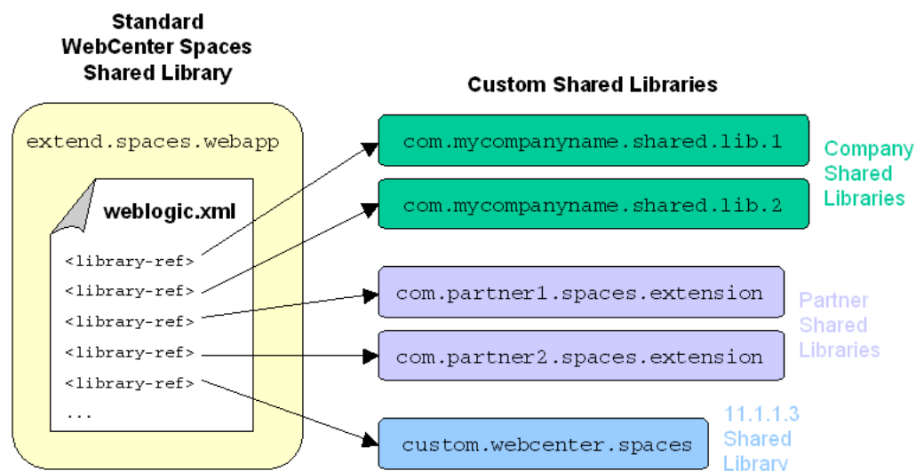
Figure 53-1 Referencing Custom Shared Libraries in extend.spaces.webapp.war
