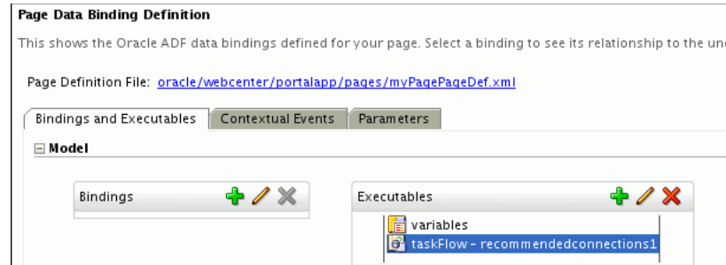
Figure 45–6 Recommended Connections in the Page Data Binding Definition
