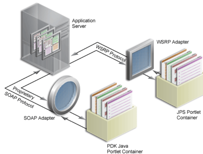
Figure 59–2 Oracle WebCenter Portlet Architecture
