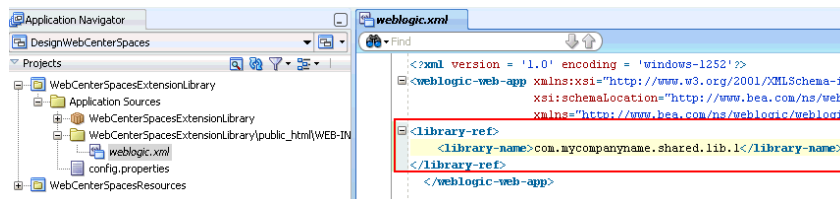
Figure 53–5 weblogic.xml - Single Shared Library Reference
