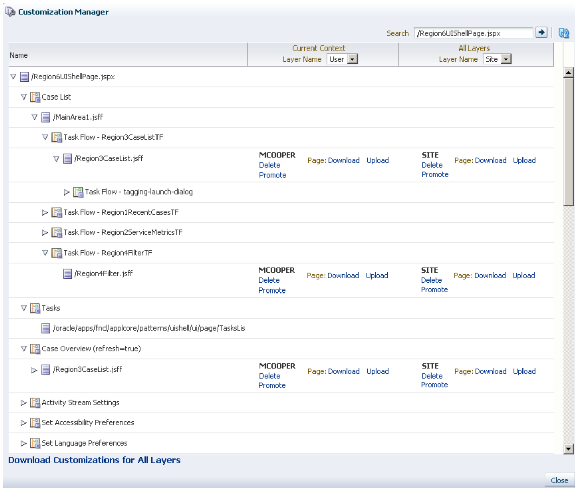
Figure 17-43 Customization Manager Dialog
