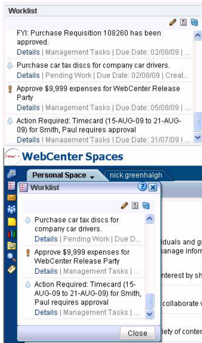
Figure 50–1 Worklist Service at Runtime
