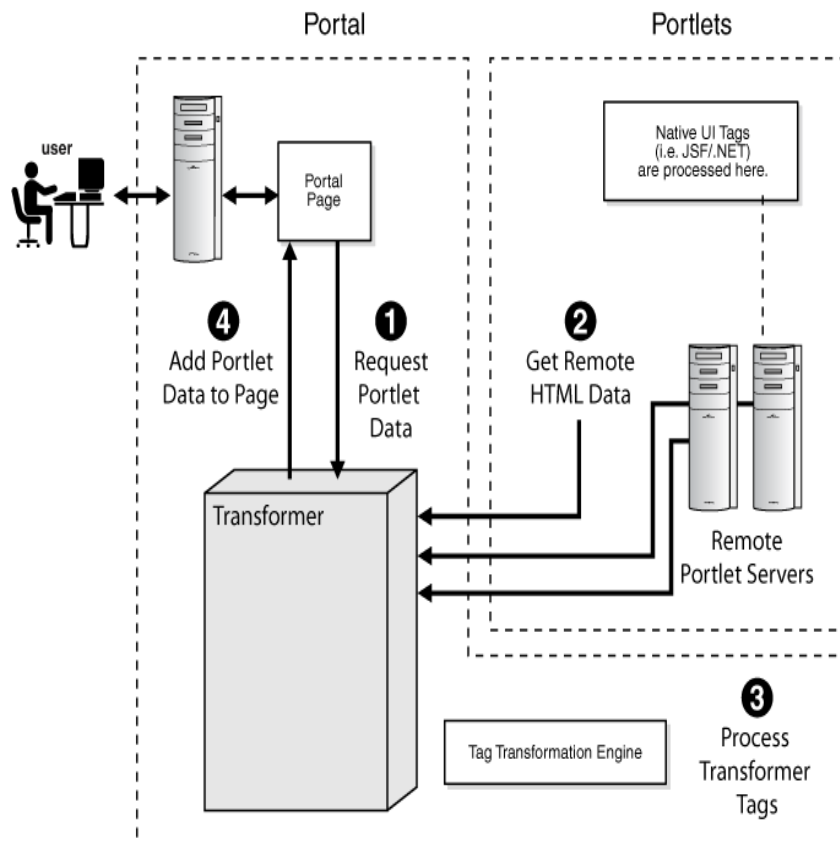
Figure 62-4 Tag Control Flow
