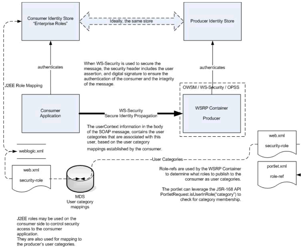
Figure 67–18 WSRP Portlet Security Architecture
