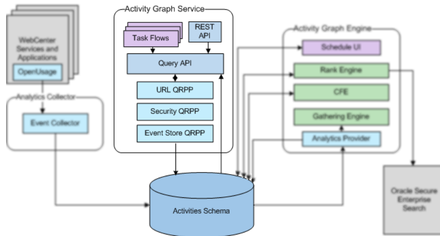
Figure 45–4 Recommendations Calculation by the Activity Graph Service
