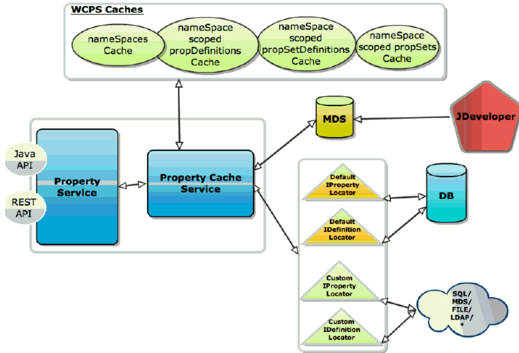
Figure 66–2 Property Service Architecture
