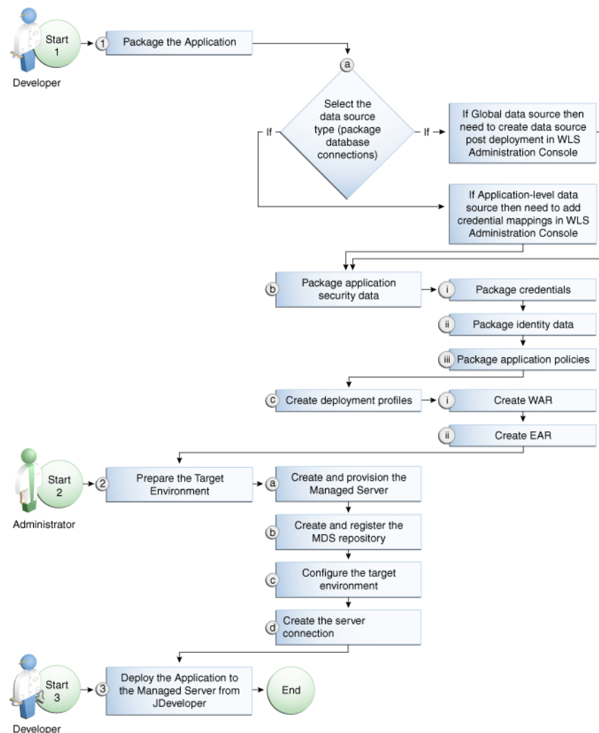
Figure 68–4 Deploying a WebCenter Portal Application to a Managed Server
