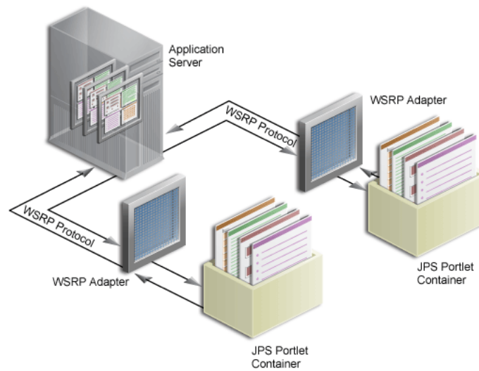
Figure 59–1 WSRP Specification Architecture
