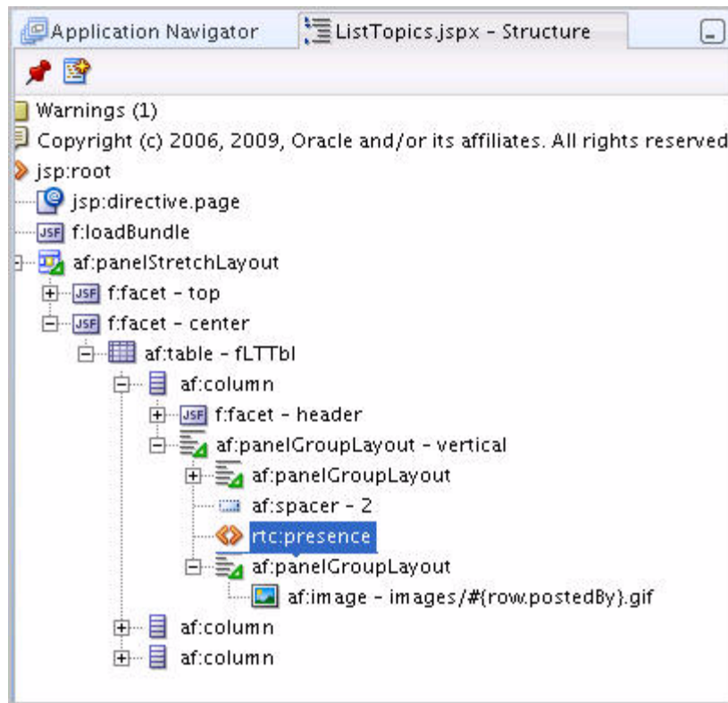
Figure 24–12 rtc:presence Tag in the Structure Window
