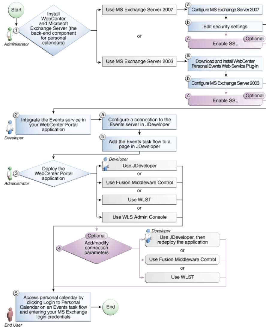
Figure 51–2 Configuring the Events Service for WebCenter Portal Applications
