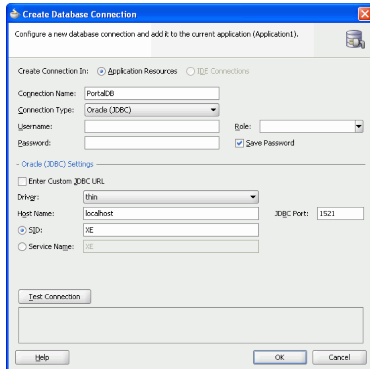
Figure 26–4 Create Database Connection
