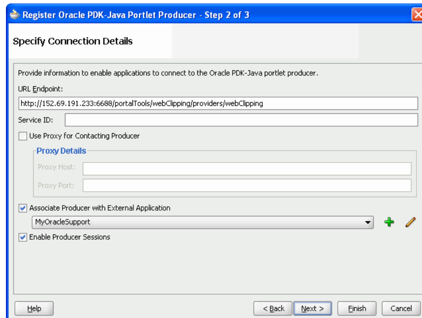
Figure 65–1 Associating a Web Clipping Producer with an External Application
