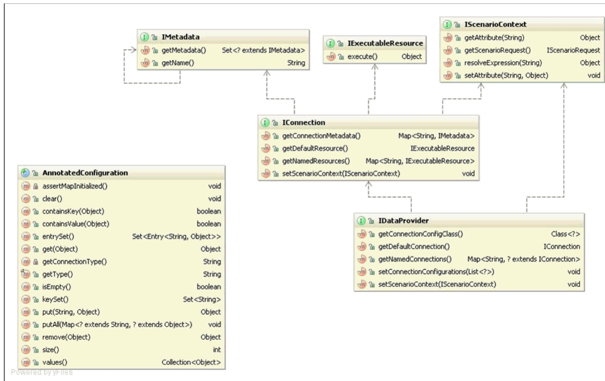
Figure 66–14 Class Interaction for Data Providers
