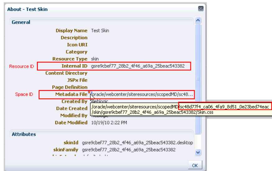
Figure 53–11 Checking Resource IDs in WebCenter Spaces
