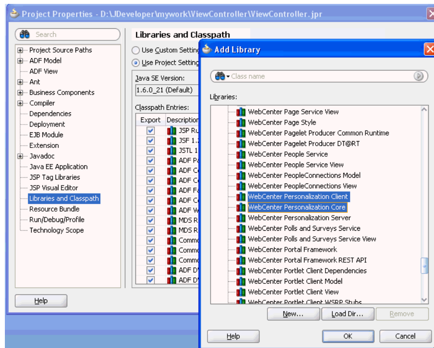
Figure 66–26 Project Properties Dialog - Adding the Extension Libraries
