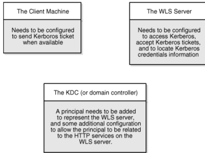
Figure 30–29 Configuring SSO with Microsoft Clients
