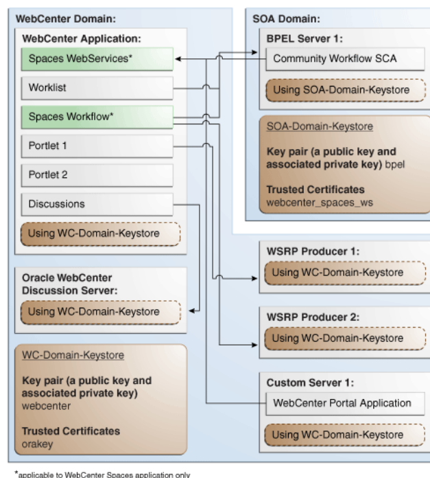
Figure 32-11 WS-Security for a Typical Configuration
