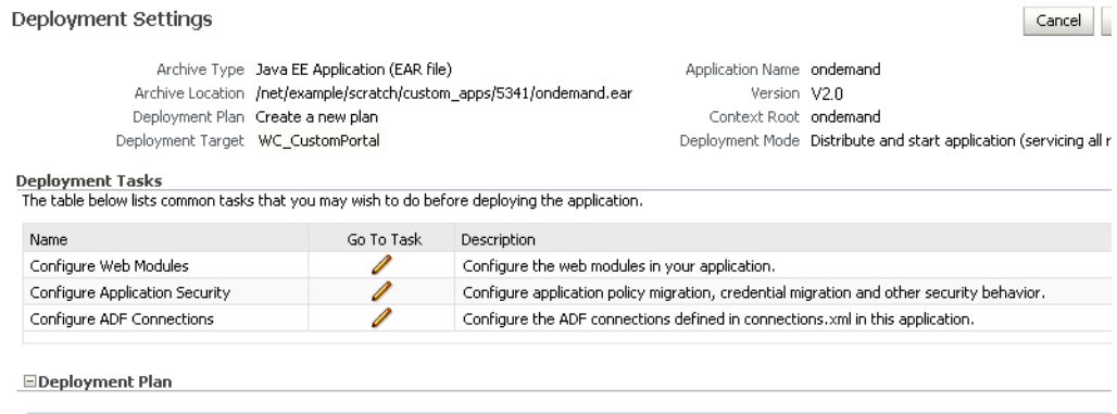
Figure 7–23 Deployment Settings Page
