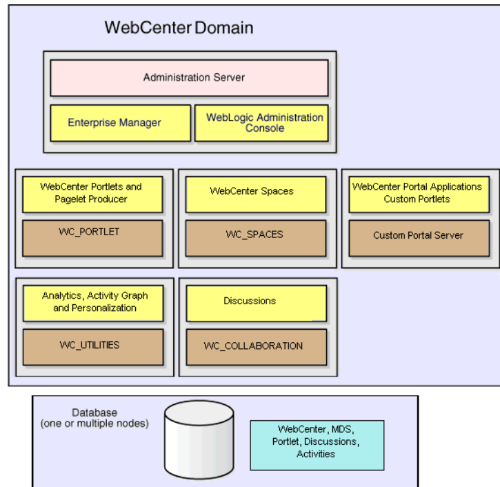
Figure 1–3 Oracle WebCenter Topology Out-of-the-Box
