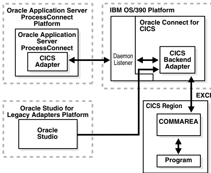
Figure 1-1 Architecture of the Oracle Application Server Integration Adapter for CICS
