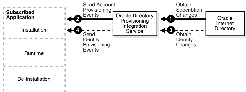
Figure 34–2 How an Application Receives Provisioning Information by Using the Oracle Directory Provisioning Integration Service
