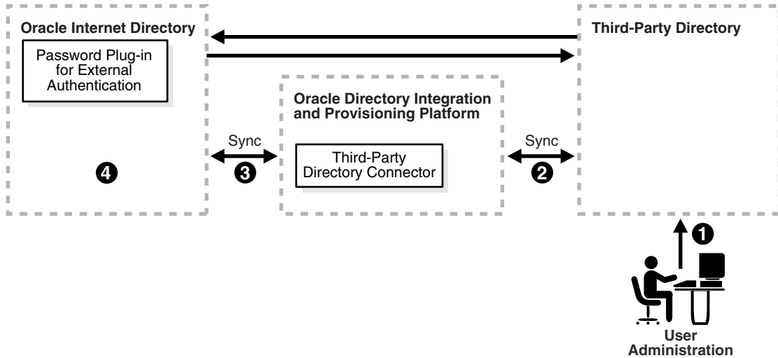
Figure 41–2 Interaction of Components with a Third-Party Directory as the Central Directory
