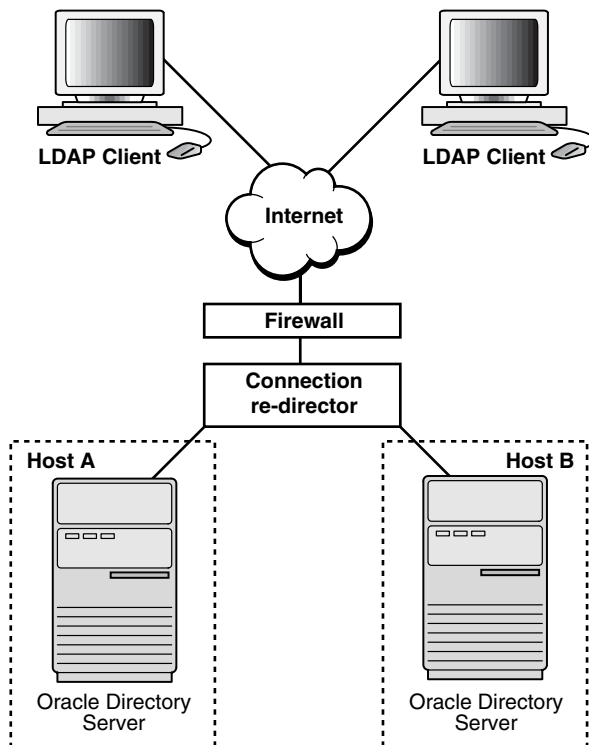
Figure 26–2 Network-Level Failover
