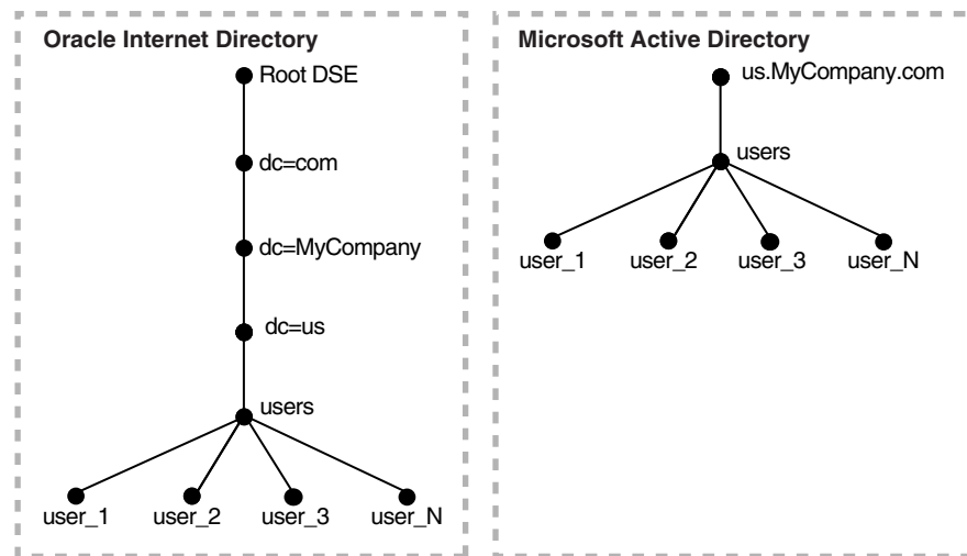
Figure 43–1 Default DIT Structures in Oracle Internet Directory and Microsoft Active Directory when Both Directory Hosts are Under the Domain us.MyCompany.com
