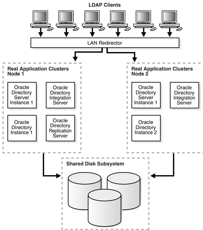
Figure 29-1 Oracle Internet Directory with Basic High Availability Configuration
