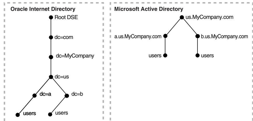
Figure 43-2 Integration of Oracle Internet Directory with Multiple Domains in Microsoft Active Directory
