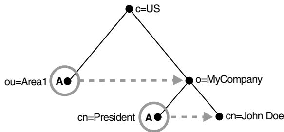
Figure 5-3 Resulting Tree when Creating the My_file.Idif
