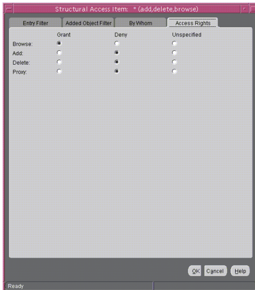
Figure 14-3 Example: Structural Access Item: Access Rights Tab Page
