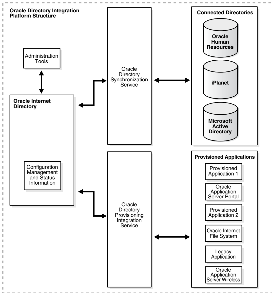
Figure 32-1 Example of an Oracle Directory Integration and Provisioning Platform Environment
