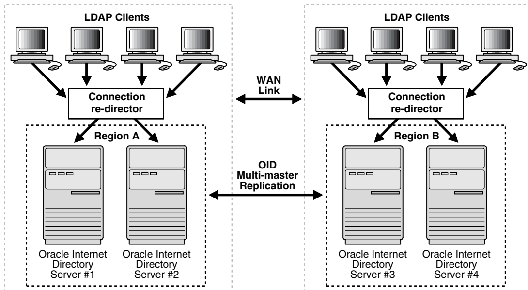
Figure 26-4 Deployment Example 2
