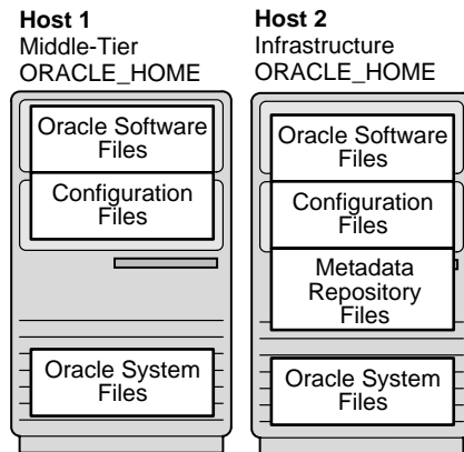
Figure 11-1 Types of Files for Oracle Application Server Backup and Recovery
