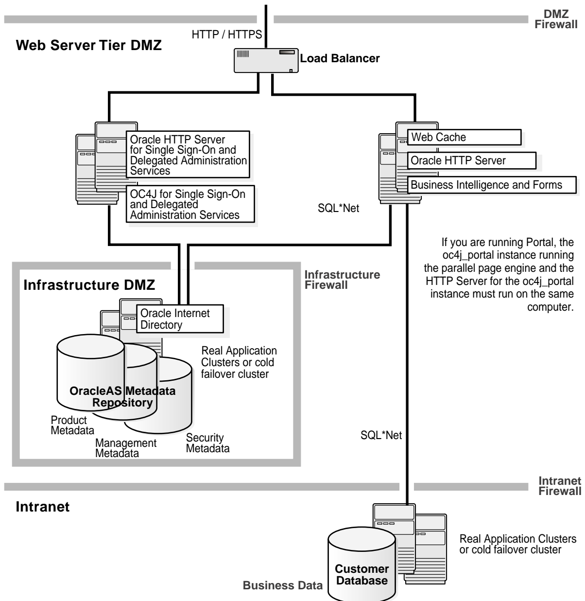
Figure 10–6 Enterprise Data Center Topology for Portal, Wireless, Business Intelligence, and Forms
