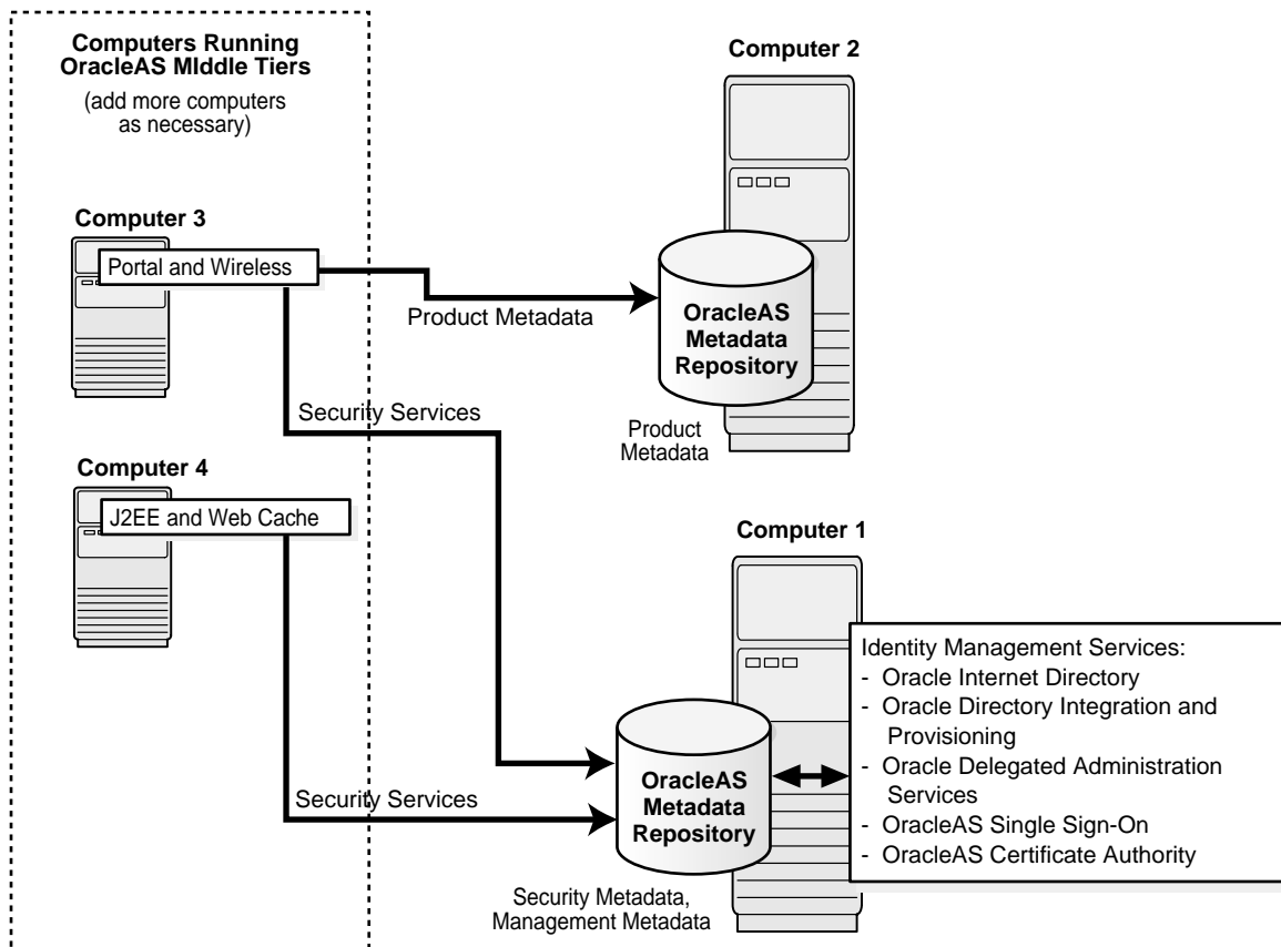
Figure 10-7 Departmental Topology
