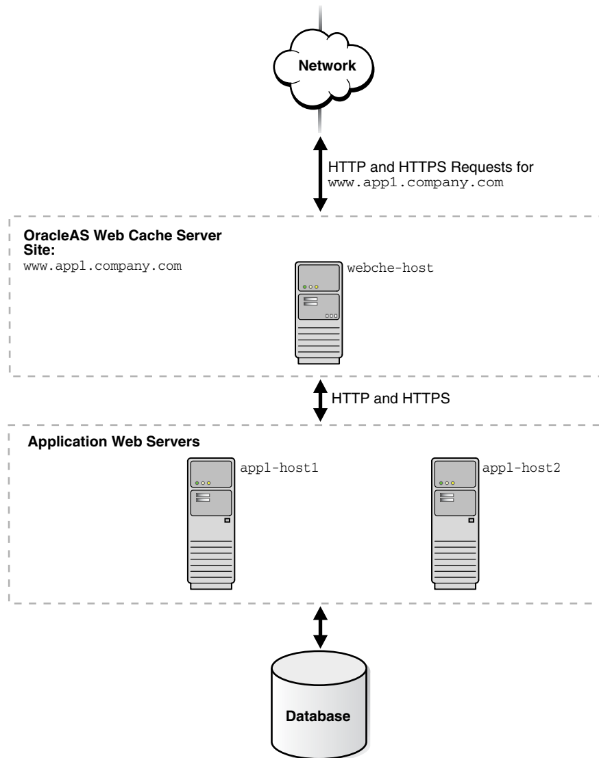
Figure 8–6 Deploying OracleAS Web Cache as a Load Balancer
