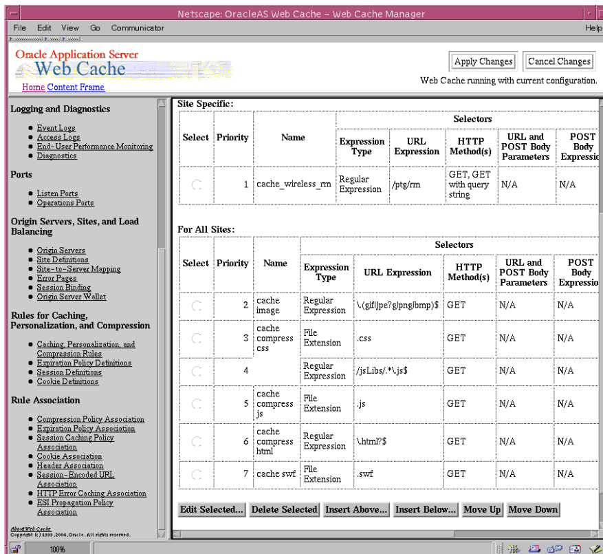
Figure 6–7 Caching, Personalization, and Compression Rules Page
