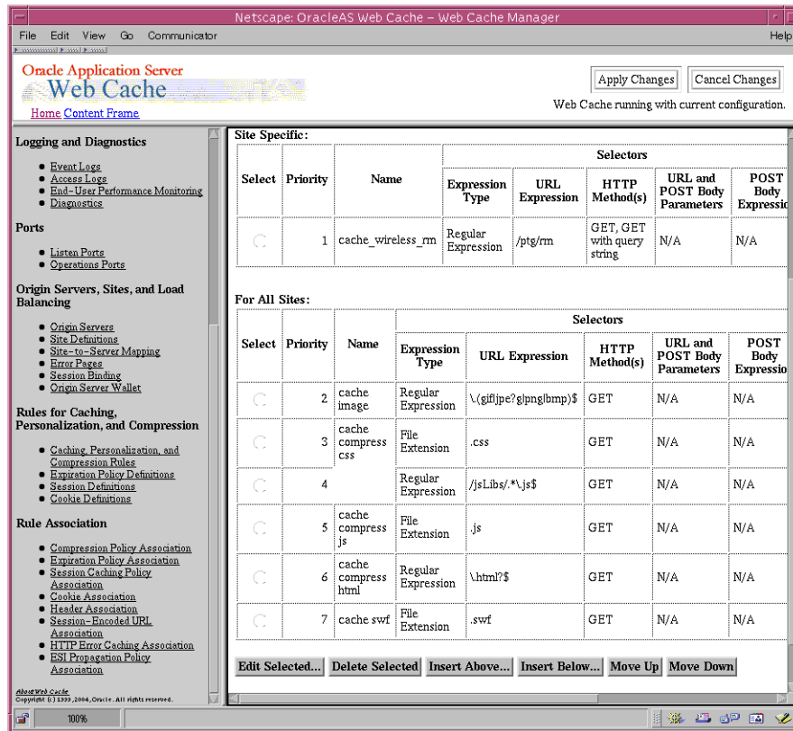
Figure 12–2 Default Caching Rules in OracleAS Web Cache Manager
