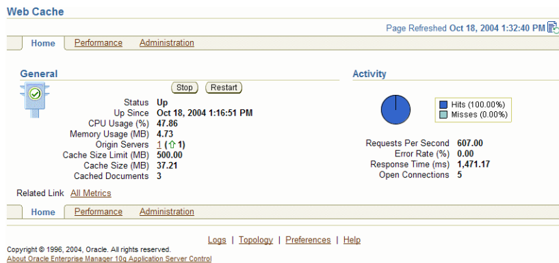
Figure 6–1 Application Server Control Console: Web Cache Home Page
