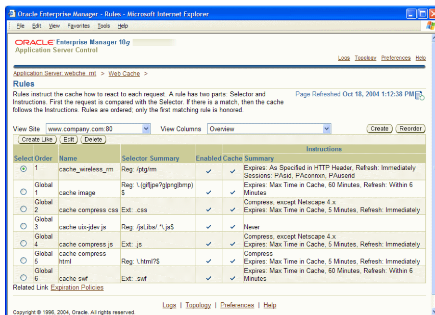
Figure 12–1 Default Caching Rules in Application Server Control Console
