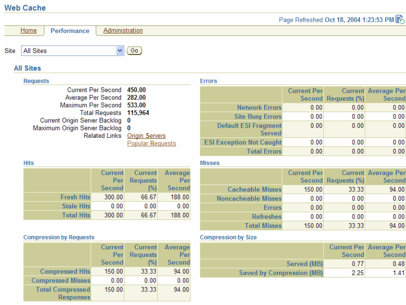
Figure 6–2 Application Server Control Console: Web Cache Performance Page
