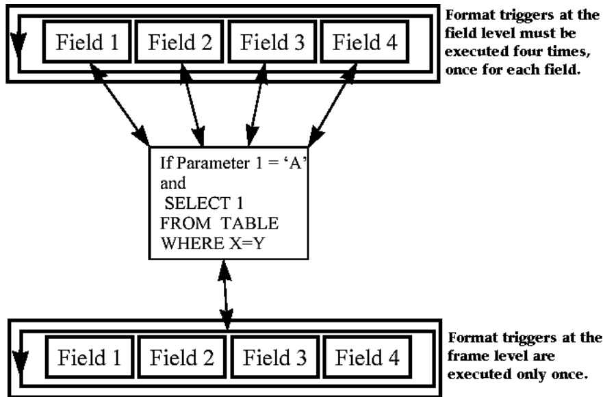
Figure 20–2 Format Triggers
