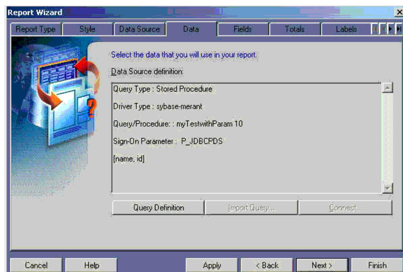
Figure 8-4 Query Description
