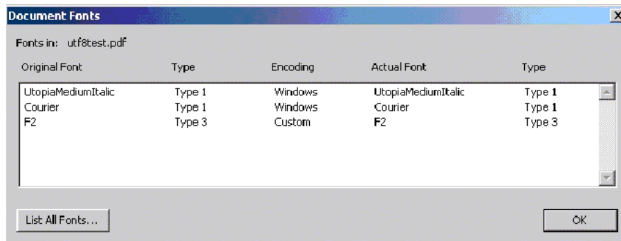
Figure 6–2 Font Subsetting
