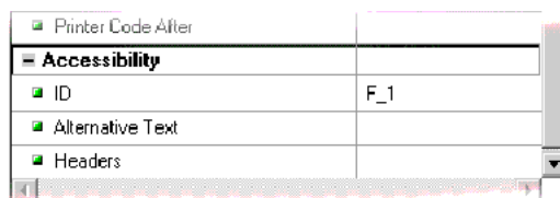
Figure 6–4 Accessibility
