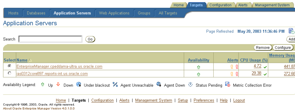
Figure 19–2 Grid Control Console, Targets, Application Servers Tab
