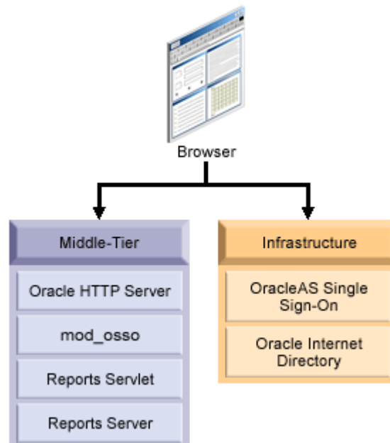
Figure 9-2 SSO Architecture
