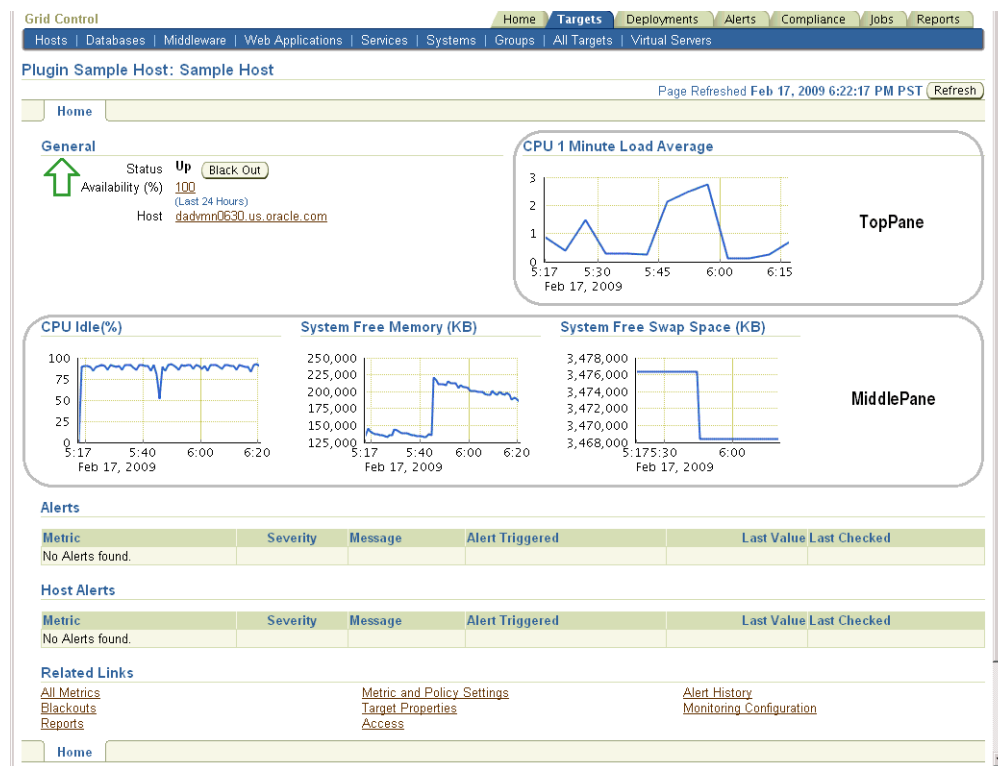
Figure 3-3 TopPane and MiddlePane Locations within the Target Home Page
