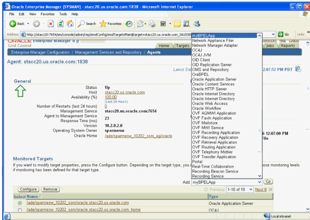
Figure 6-4 Selecting a JMX Target Type
