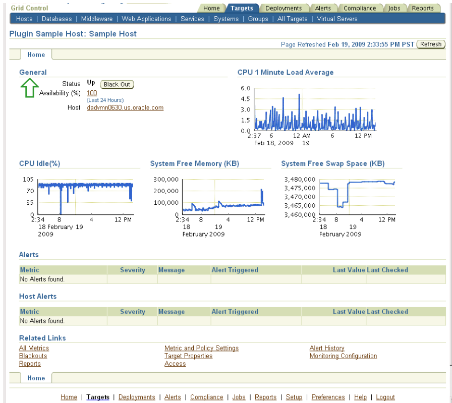
Figure 3–2 Default Target Home Page with Charts
