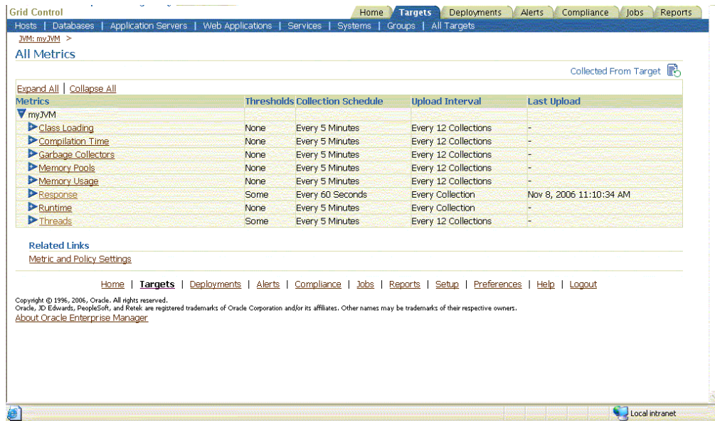
Figure 6–8 Metrics Collected from the JVM
