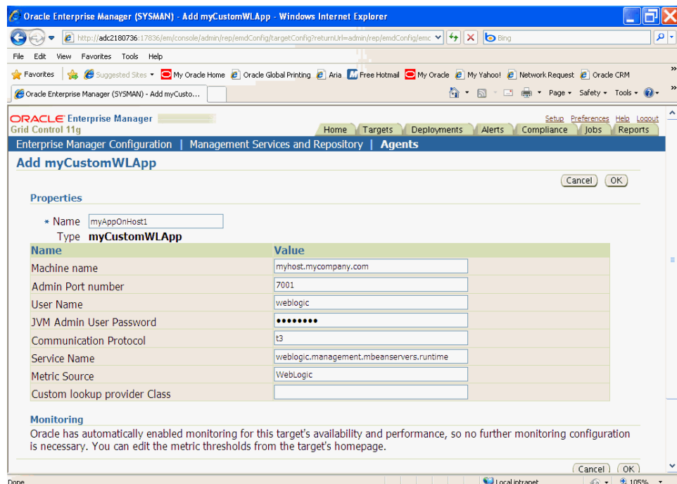
Figure 6–11 Specifying Target Properties
