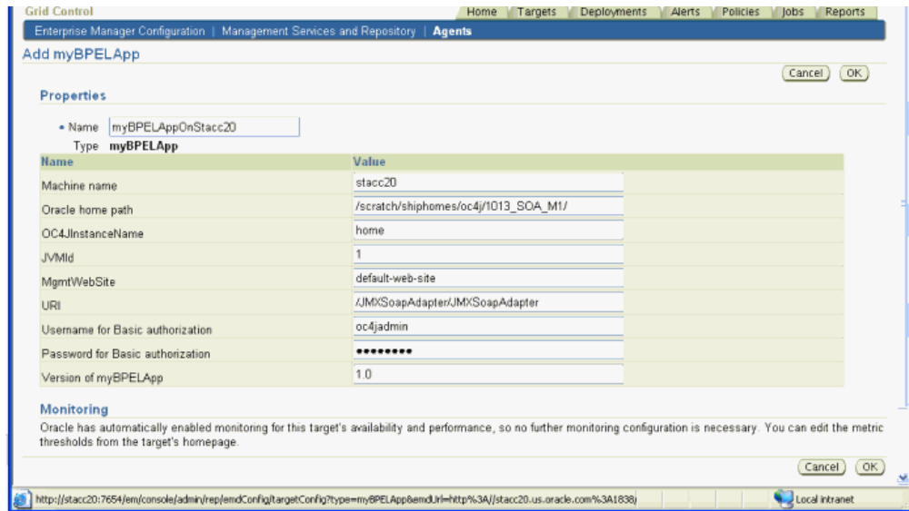
Figure 6-5 Specifying JMX Target Properties
