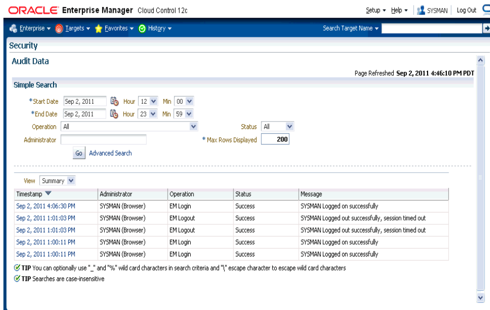
Figure 13–10 Audit Data Search Page
