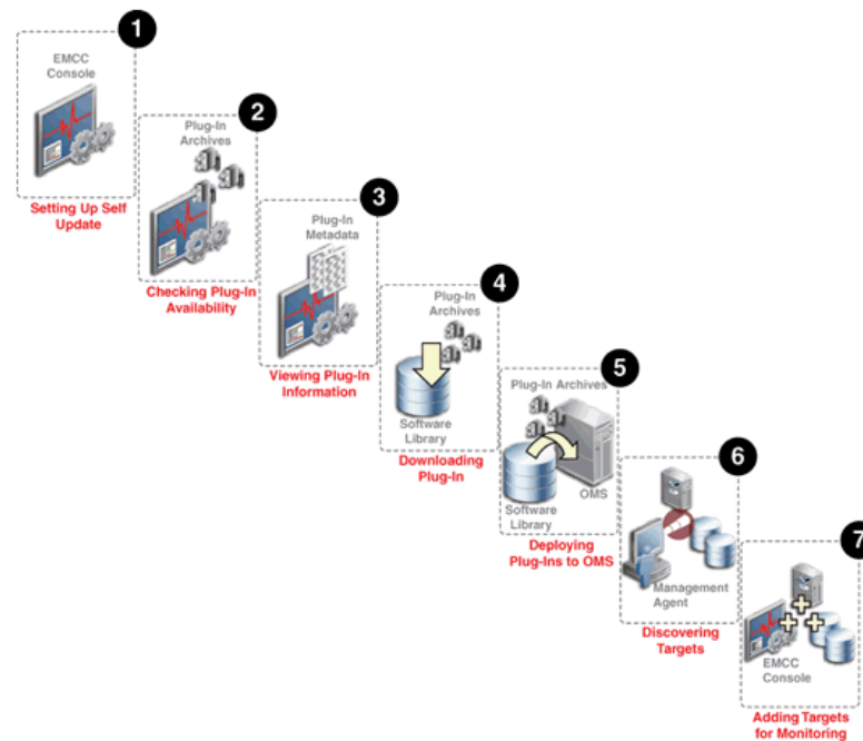
Figure 22–1 Plug-In Deployment Workflow
