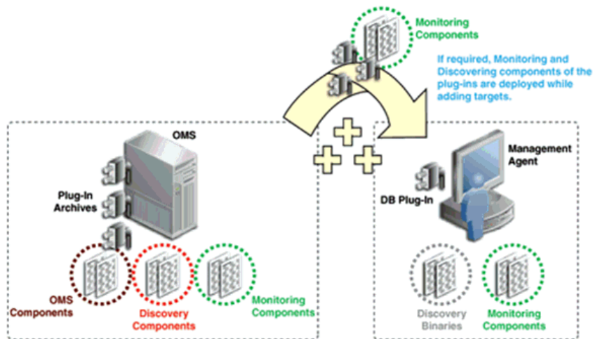
Figure 22–4 Adding Targets
