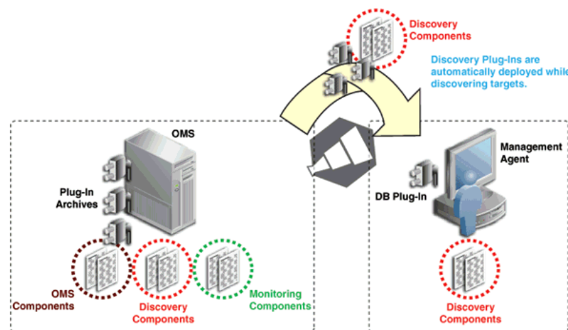
Figure 22–3 Discovering Targets
