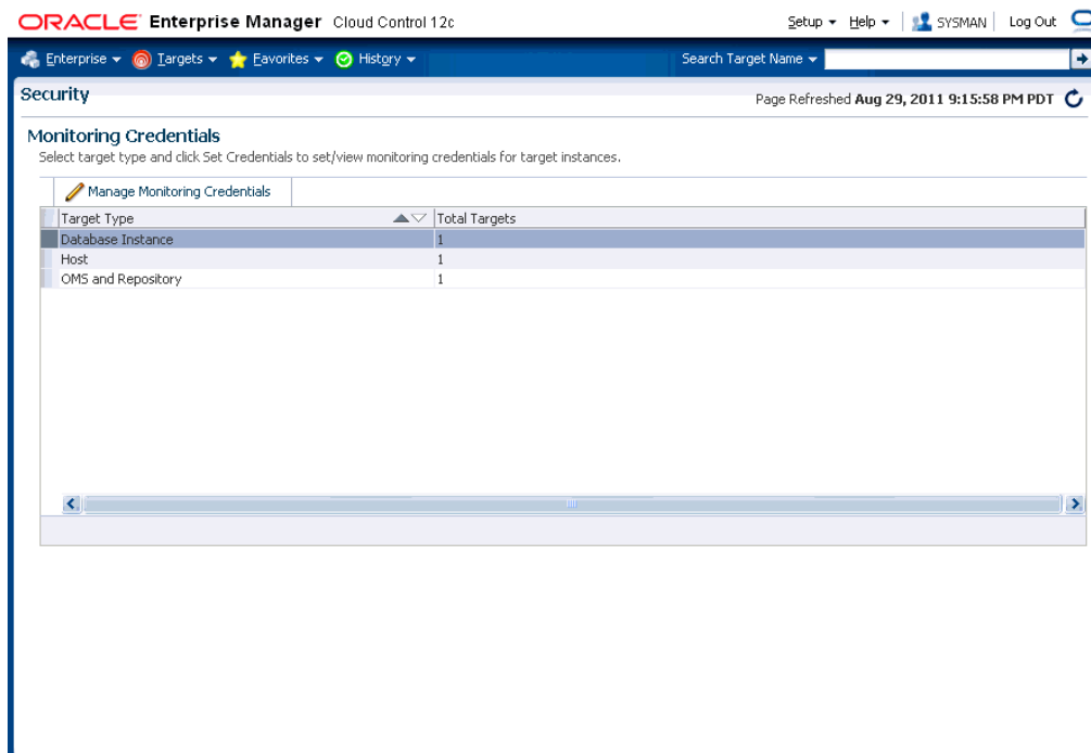
Figure 13–5 Monitoring Credentials
