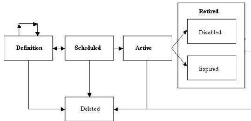
Figure 10–8 SLA Lifecycle
