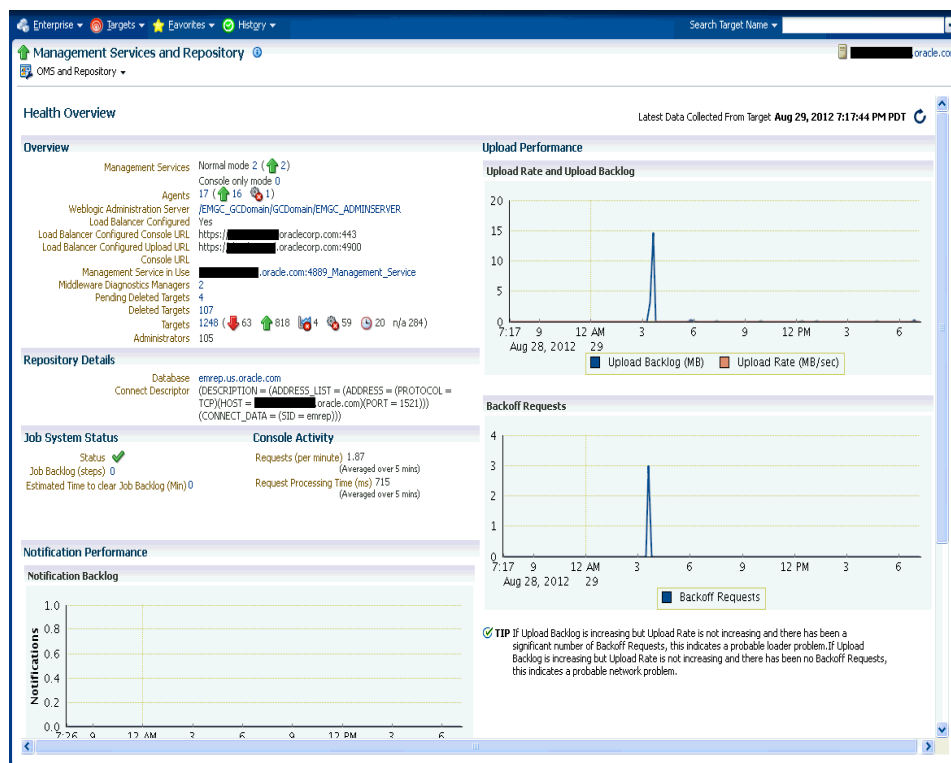
Figure 19–1 Health Overview Page
