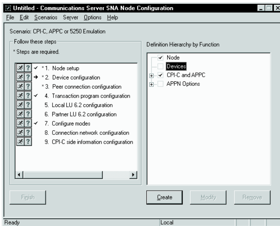
Figure 7-4 Creating Devices
