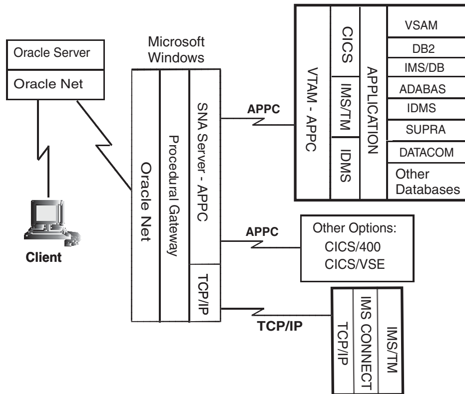
Figure 1–2 Gateway Architecture Featuring SNA or TCP/IP Protocol
