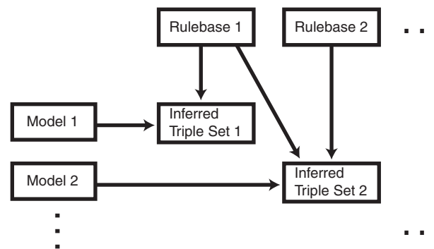
Figure 1–2 Inferencing
