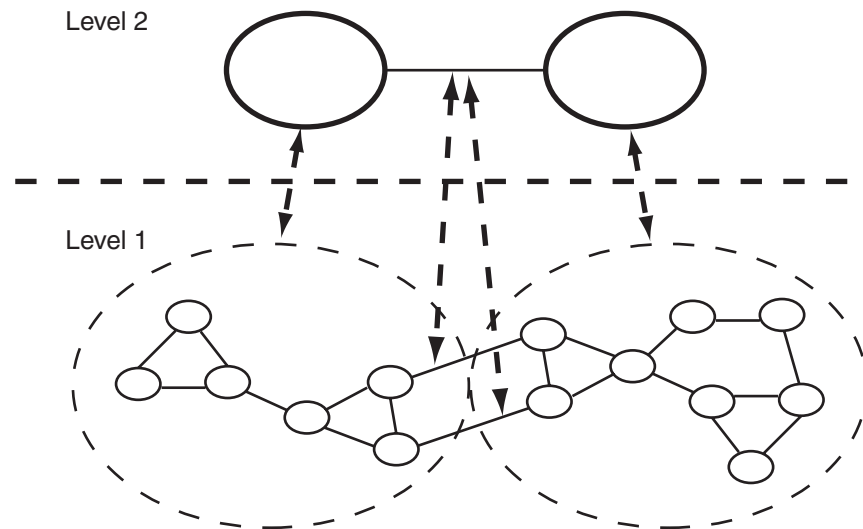
Figure 5–3 Network Hierarchy
