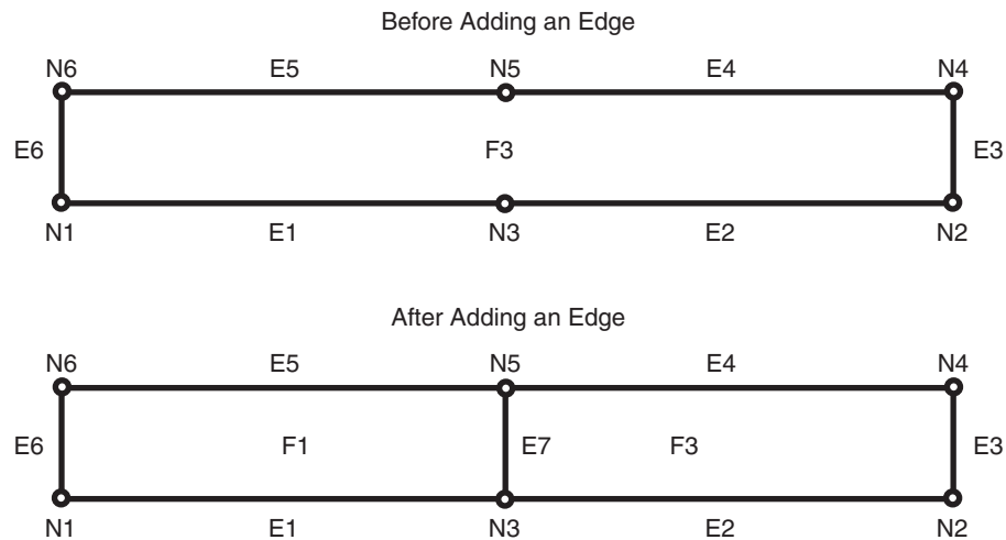
Figure 2–11 Adding a Non-Isolated Edge
