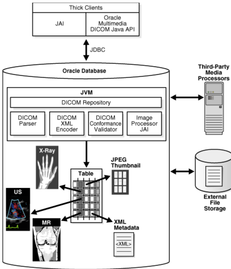
Figure 2–1 Oracle Multimedia DICOM Architecture
