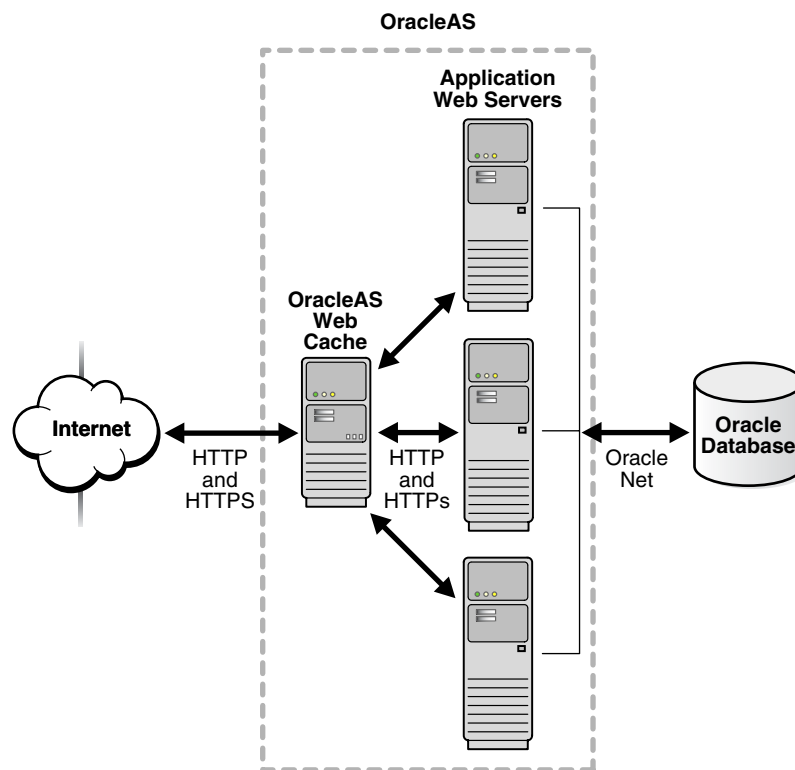
Figure 12–1 Middle-Tier Caching
