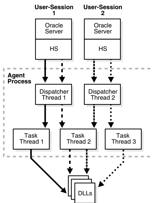
Figure A-1 Multithreaded extproc Agent Architecture
