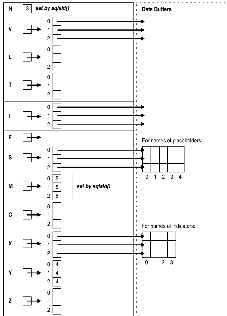
Figure 15-3 Initialized Bind Descriptor
