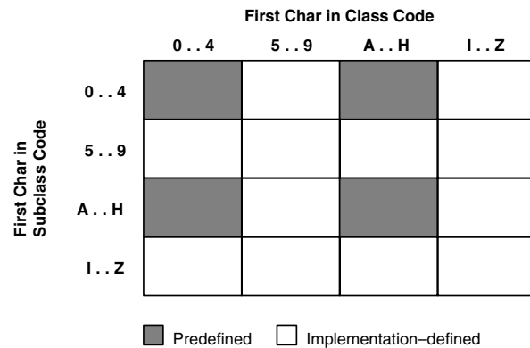
Figure 9–1 SQLSTATE Coding Scheme
