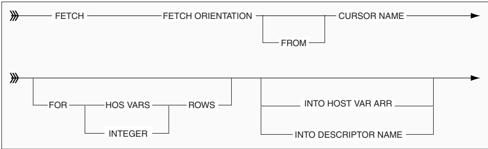
Figure 7-2 Additional Fetch Syntax
