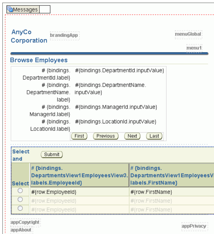
Figure 7–13 Master-Detail View in Visual Editor
