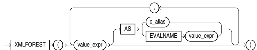
Figure 18-3 XMLFOREST Syntax
