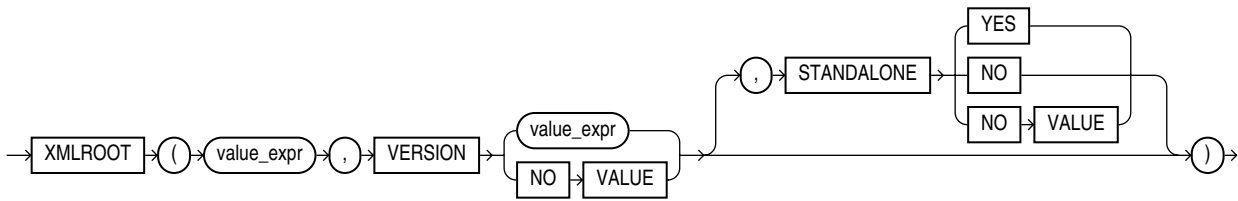
Figure 18–10 XMLRoot Syntax
