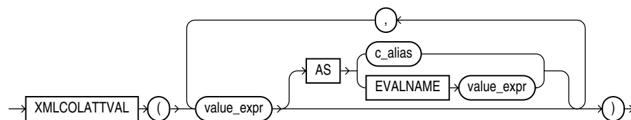
Figure 18–11 XMLCOLATTVAL Syntax
