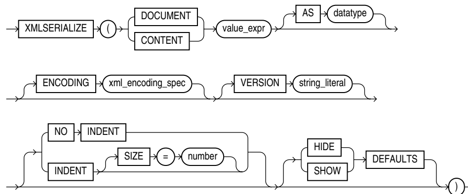
Figure 18-8 XMLSerialize Syntax
