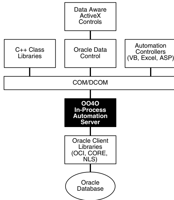
Figure 13–2 Software Layers
