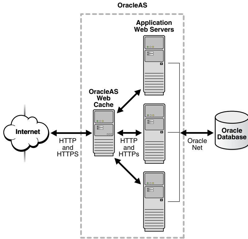
Figure 11-1 Middle-Tier Caching
