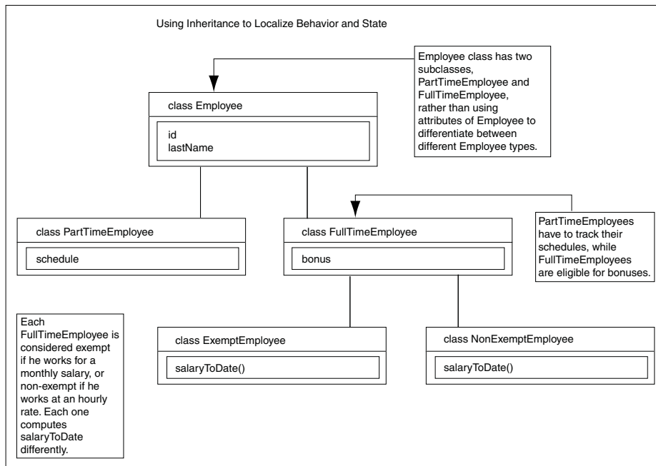
Figure 1–4 Class Hierarchy
