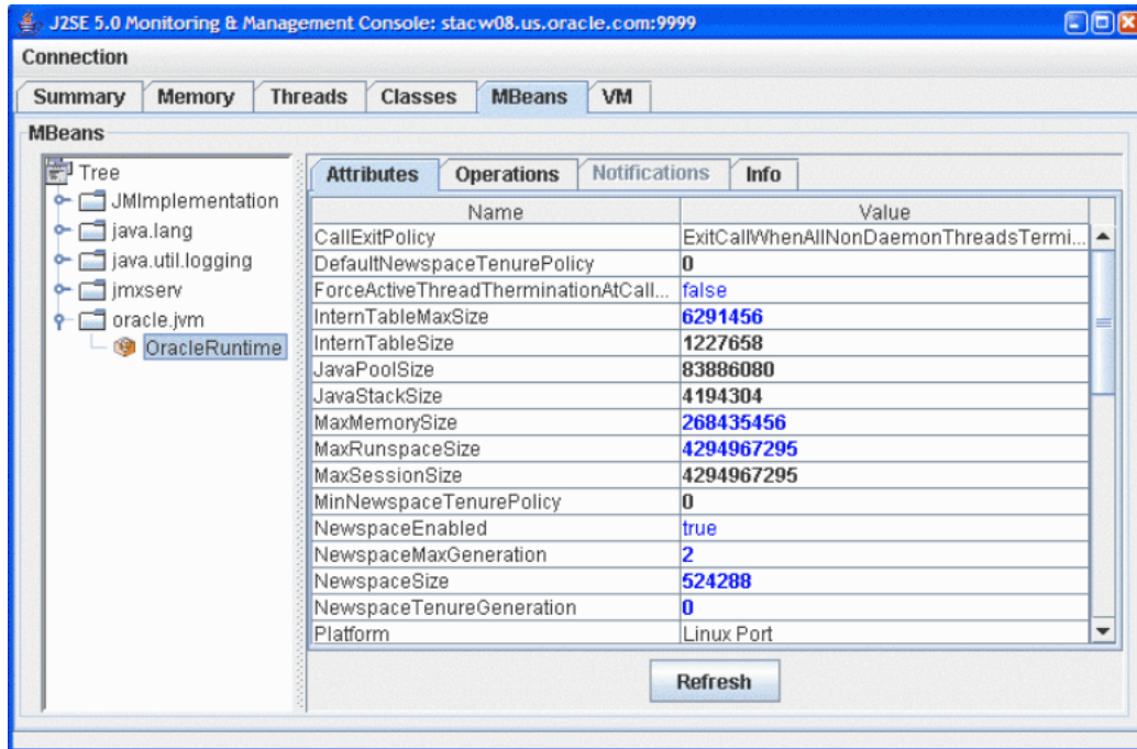
Figure 2–15 Attributes Tab of the OracleRuntime MBean
