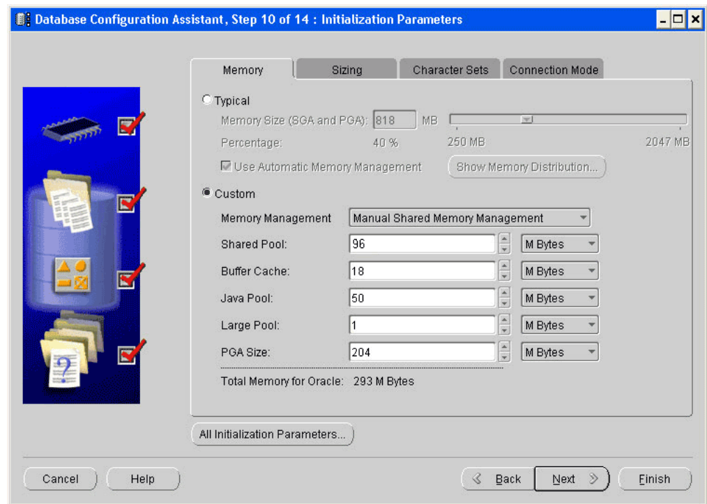
Figure 9–1 Configuring Oracle JVM Memory Parameters
