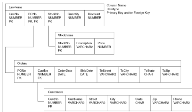
Figure 8–3 Schema Plan for Purchase Order Application
