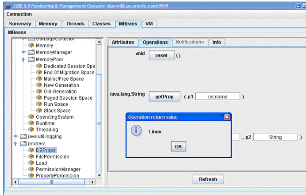
Figure 2–13 Operations Tab of the MBeans Tab of the JConsole Interface
