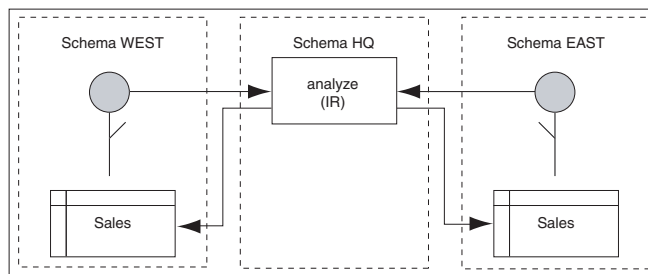
Figure 2-4 Invoker's rights Solution
