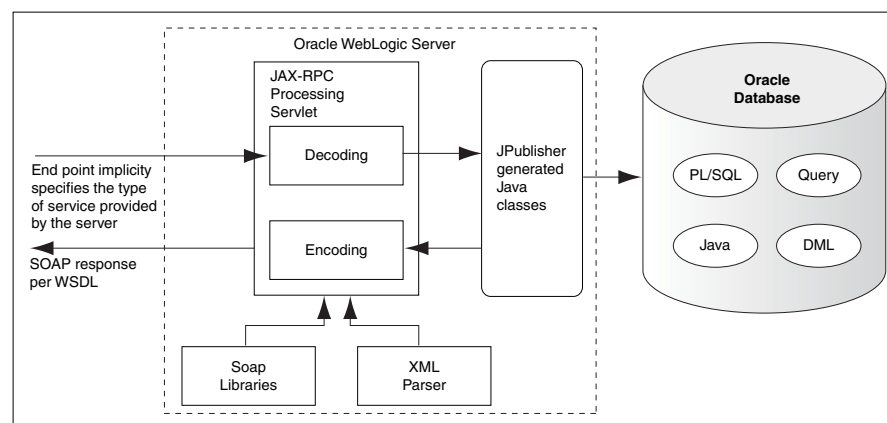
Figure 3–1 Client-Side Stub Interface
