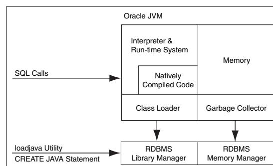
Figure 1–8 Main Components of an Oracle JVM
