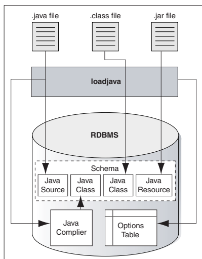
Figure 2–2 Loading Java into Oracle Database
