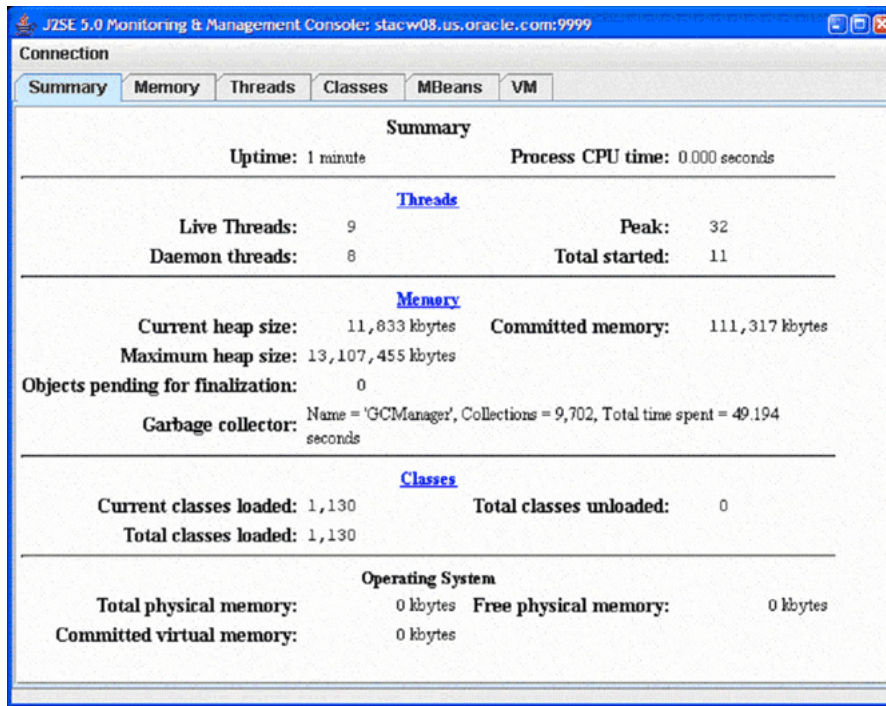
Figure 2–6 The Summary Tab of the JConsole Interface
