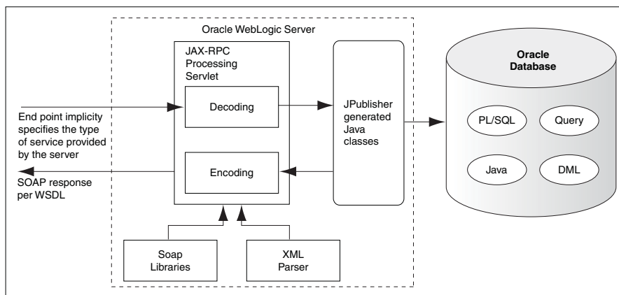
Figure 12-1 Web Services Call-In to the Database
