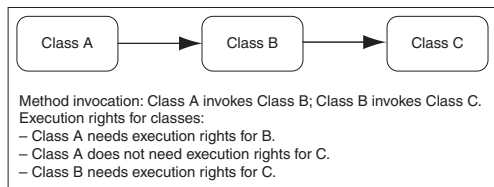
Figure 2–3 Rights to Run Classes
