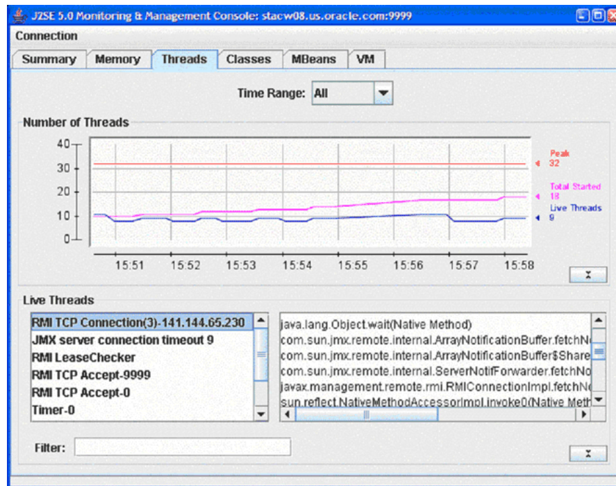
Figure 2–8 The Threads Tab of the JConsole Interface
