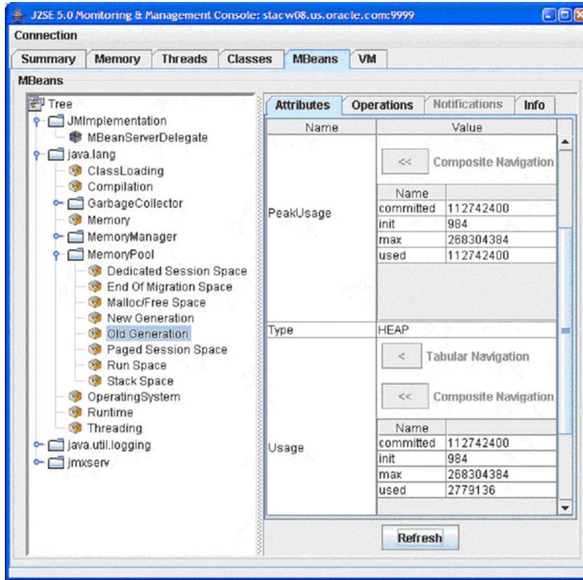
Figure 2-12 Displaying Details of a Complex Attribute in the MBeans Tab
