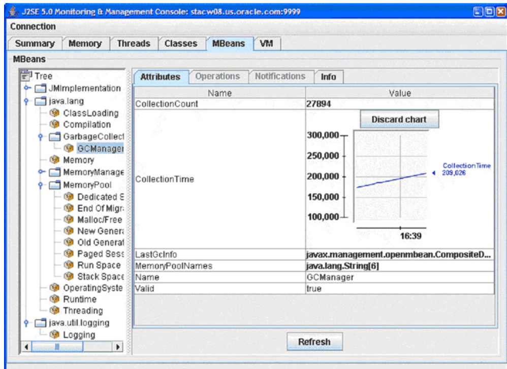
Figure 2–11 Displaying a Chart of the Values of an Attribute
