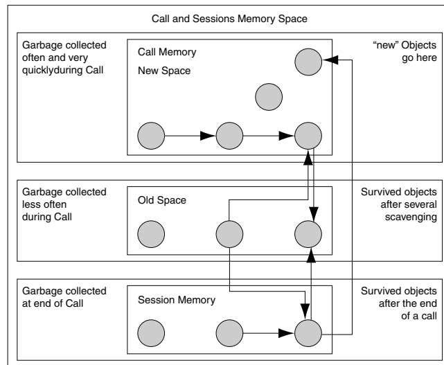
Figure 1–6 Garbage Collection
