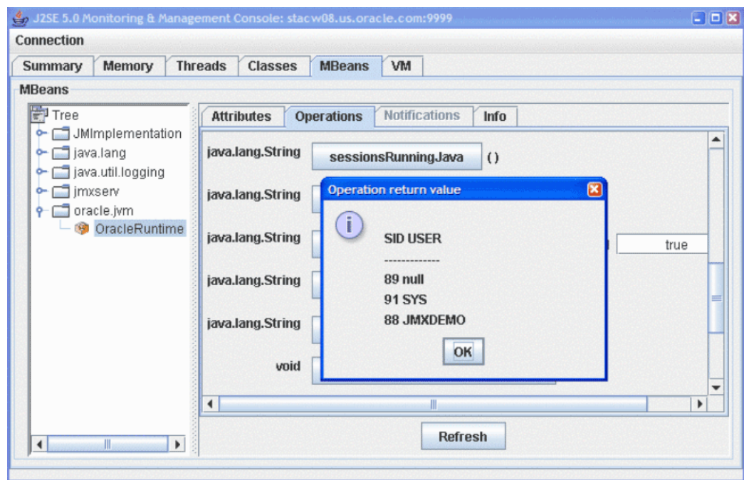
Figure 2–17 Operation sessionsRunningJava
