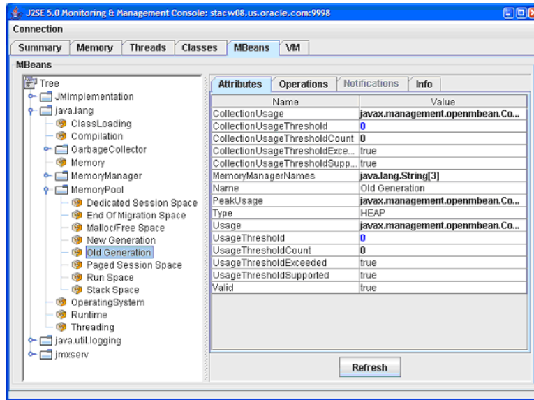
Figure 2–10 Displaying the Attributes of an MBean
