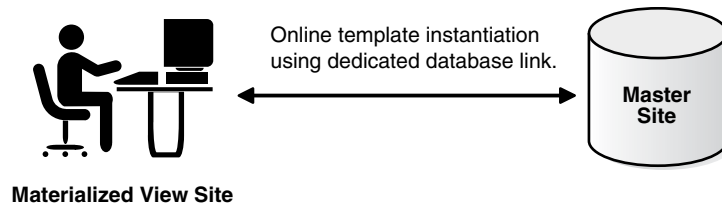
Figure 4–3 Online Instantiation
