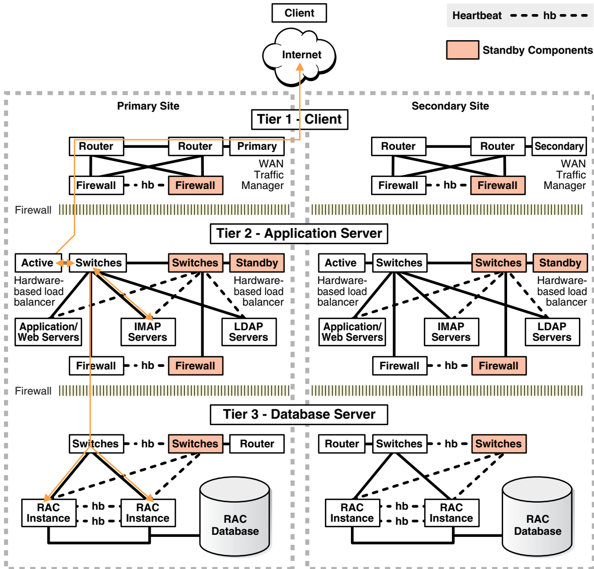
Figure 13–1 Network Routes Before Site Failover
