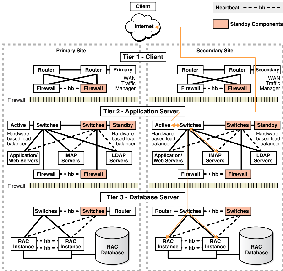
Figure 13–2 Network Routes After Site Failover
