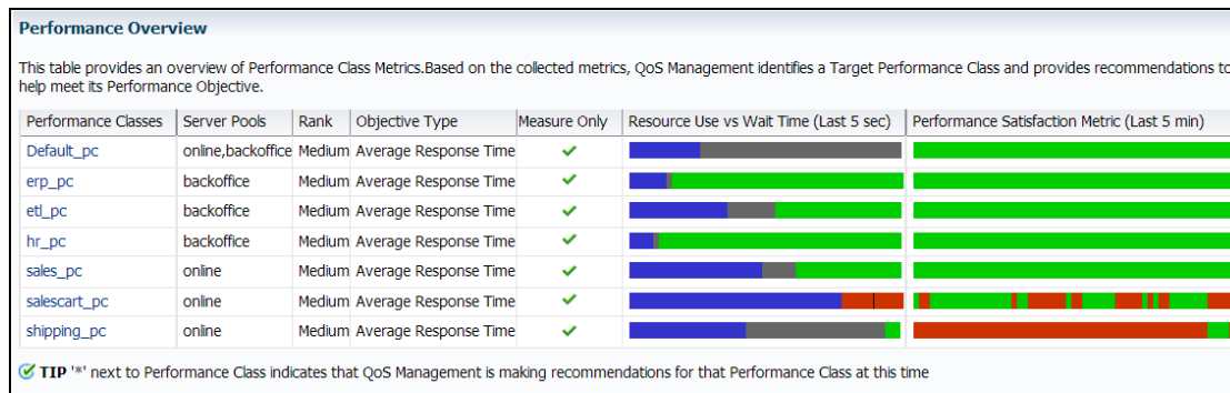
Figure 4-1 Performance Satisfaction Metrics for Measure-Only Performance Classes
