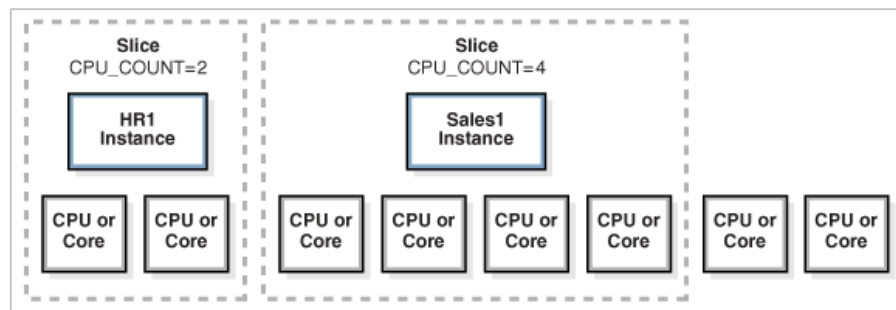
Figure 1–1 Instance Caging and CPU Slices
