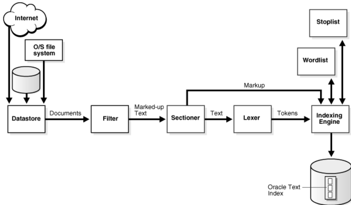
Figure 1 Oracle Text Indexing Process
