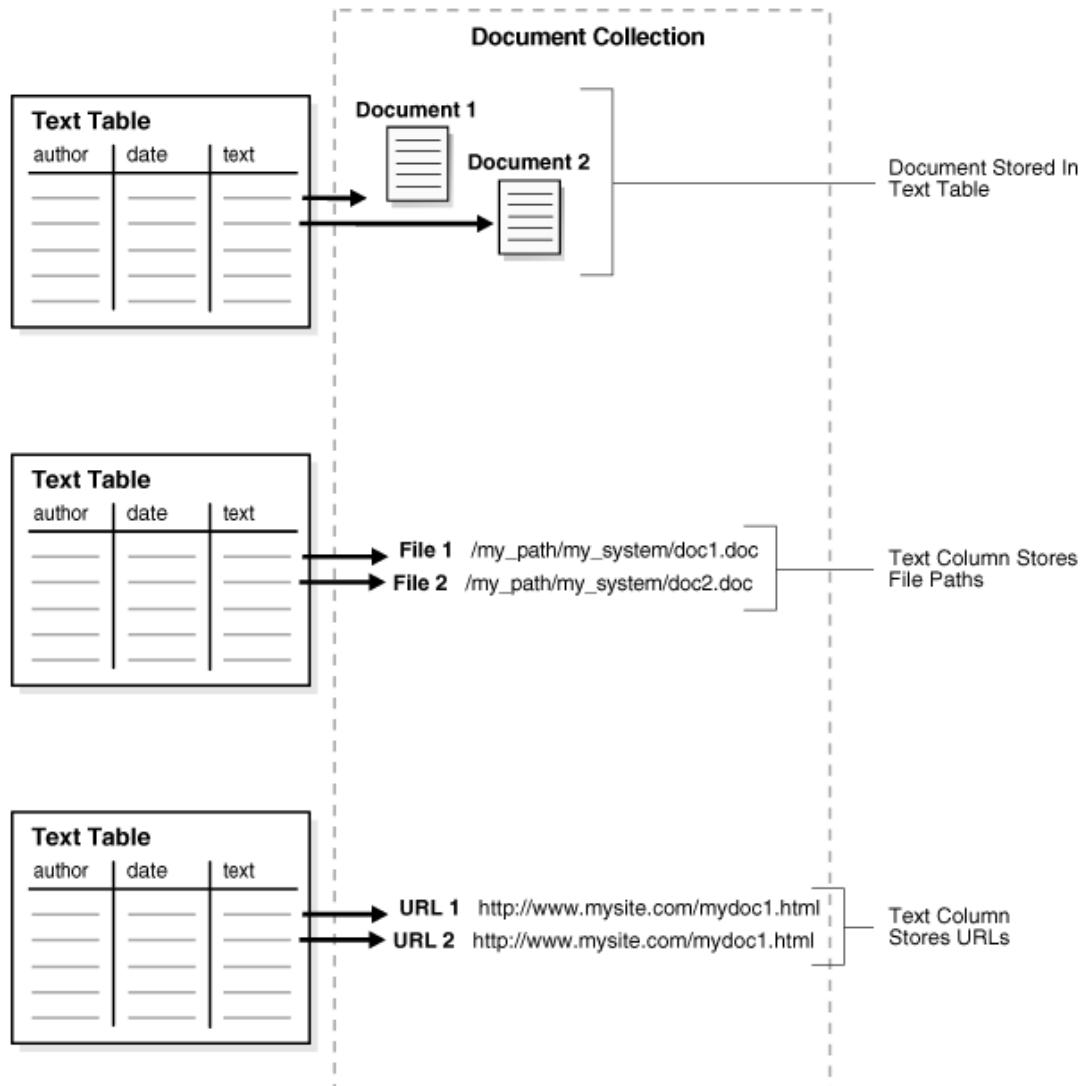
Figure 2 Different Ways of Storing Text
