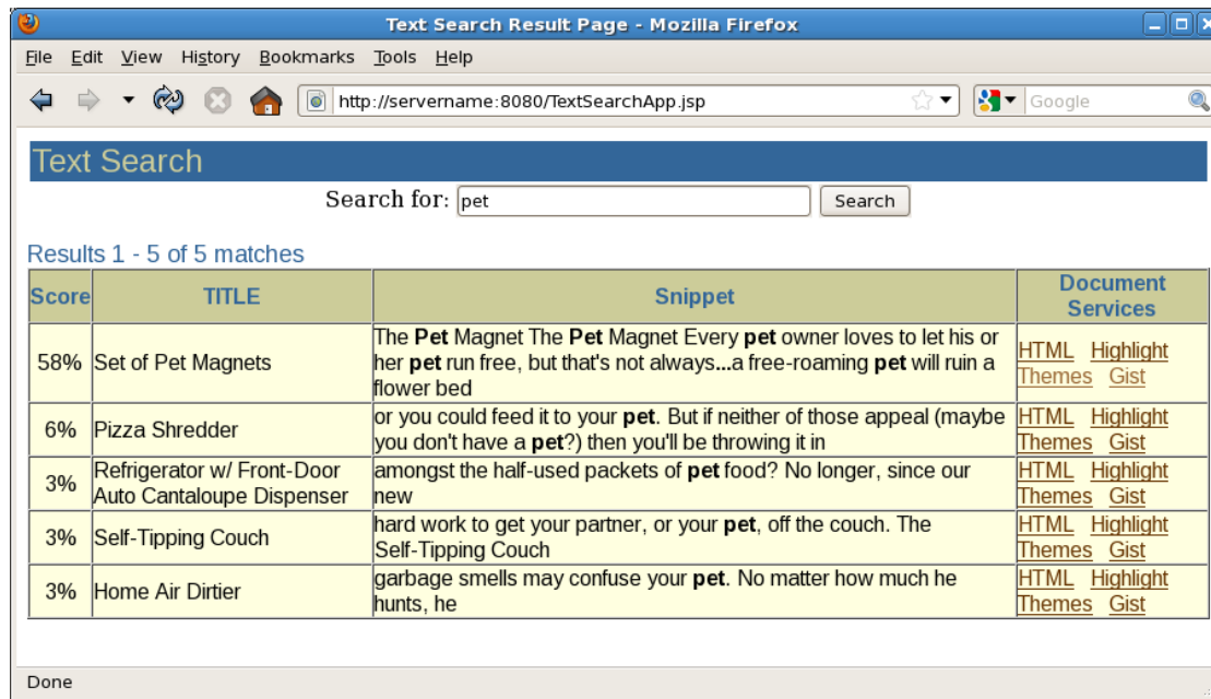
Figure 2 The Text Query Application with Results
