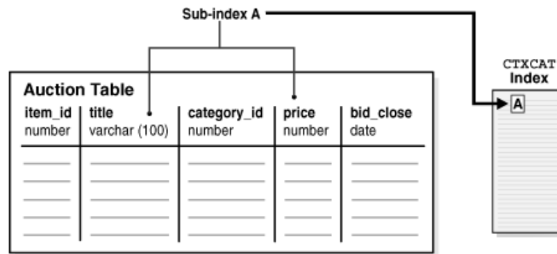
Figure 1 Auction table schema and CTXCAT index
