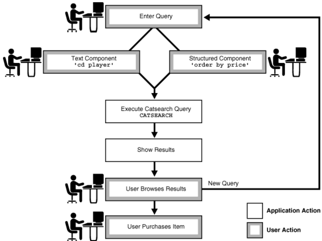
Figure 4 Flowchart of a Catalog Query Application
