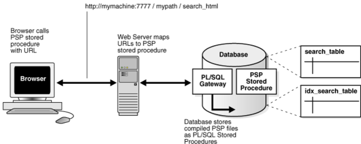
Figure 3 The PSP Web Application
