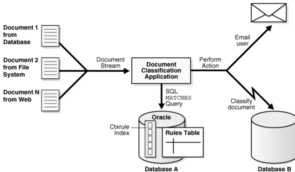
Figure 1 Overview of a Document Classification Application
