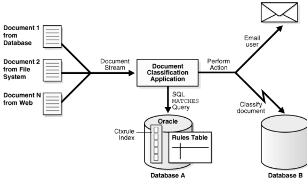
Figure 2 Overview of a Document Classification Application
