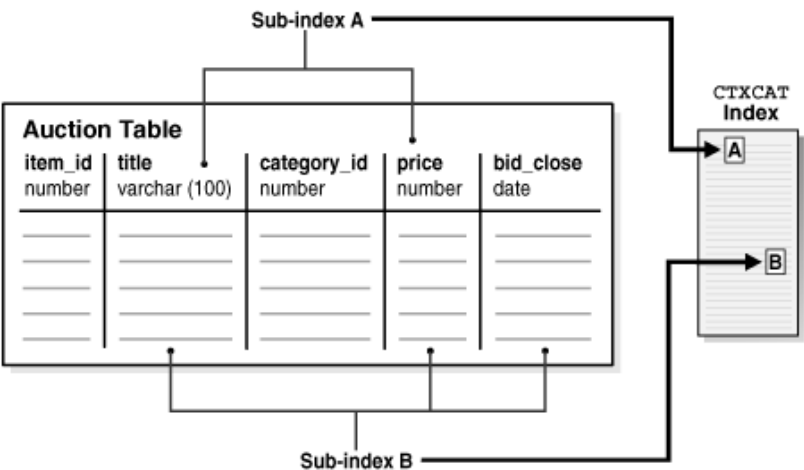
Figure 3 Auction Table Schema and CTXCAT Index
