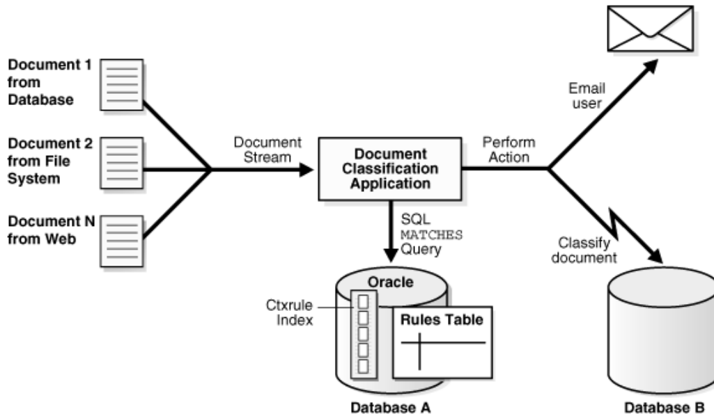
Figure 5 Overview of a Document Classification Application
