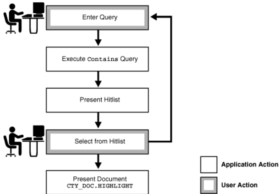
Figure 2 Flowchart of a query application
