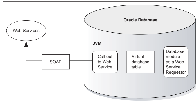
Figure 13–3 Storing Results from Request in a Virtual Table
