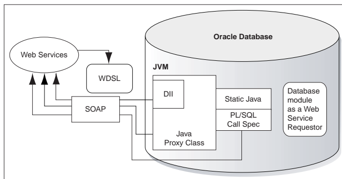
Figure 13–2 Calling Web Services From Within the Database
