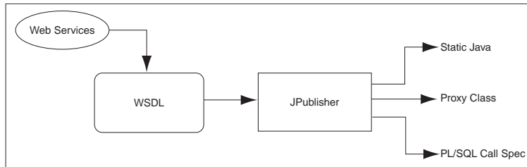
Figure 13-4 Creating Web Services Call-Out Stubs
