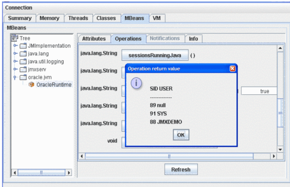
Figure 2–17 Operation sessionsRunningJava
