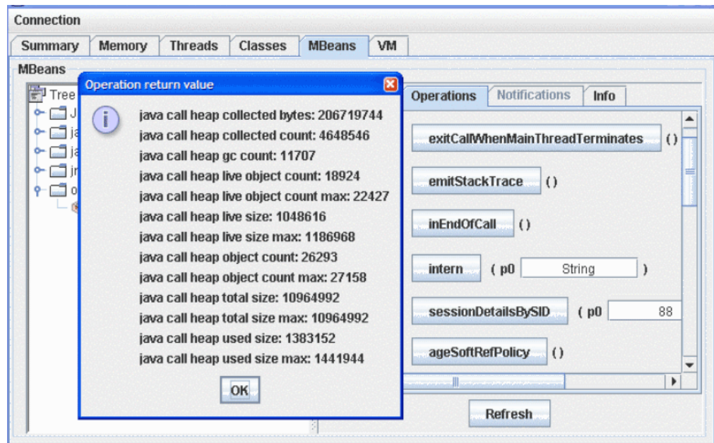
Figure 2–18 Operation sessionDetailsBySID
