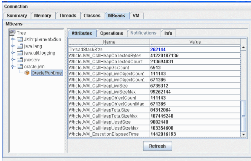
Figure 2–16 OracleRuntime MBean
