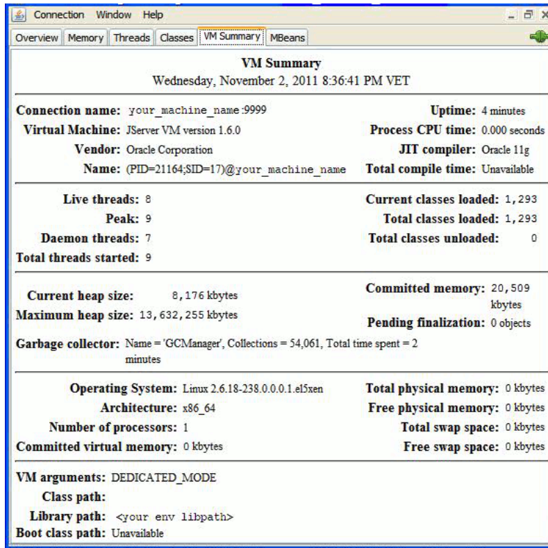
Figure 2–14 The VM Tab of the JConsole Interface
