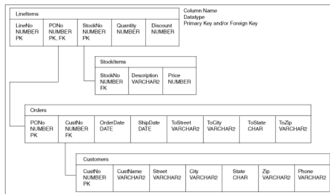
Figure 8-1 Schema Plan for Purchase Order Application
