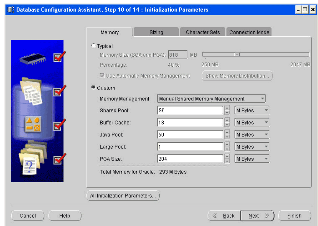
Figure 9-1 Configuring Oracle JVM Memory Parameters
