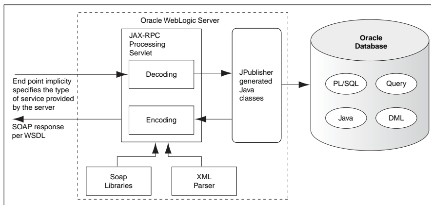
Figure 13-1 Web Services Call-In to the Database
