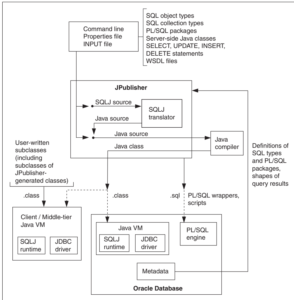
Figure 1–7 Translating and Using JPublisher-Generated Code
