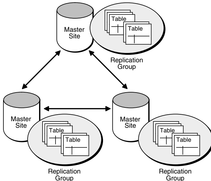
Figure 2-1 Multimaster Replication
