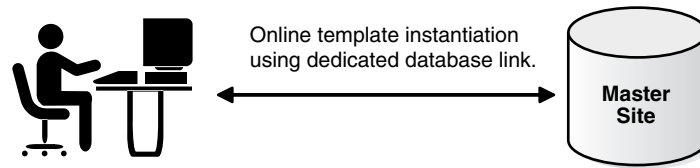
Figure 4–3 Online Instantiation
