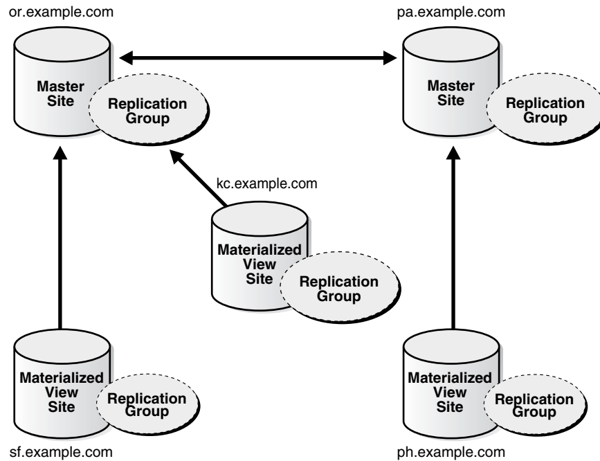
Figure 1–4 Hybrid Configuration
