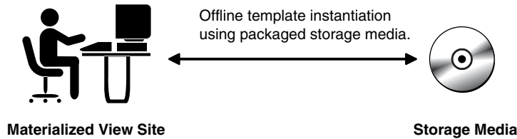
Figure 4–4 Offline Instantiation
