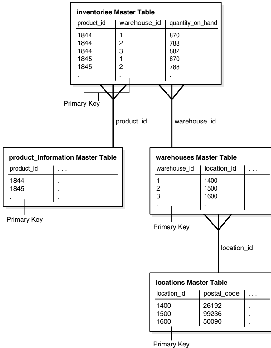
Figure 4–7 Product/Warehouse Relationship
