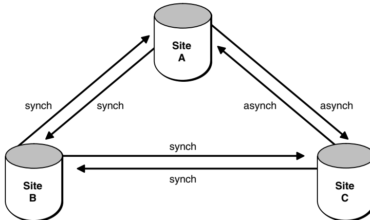
Figure 2–10 Ordering Considerations
