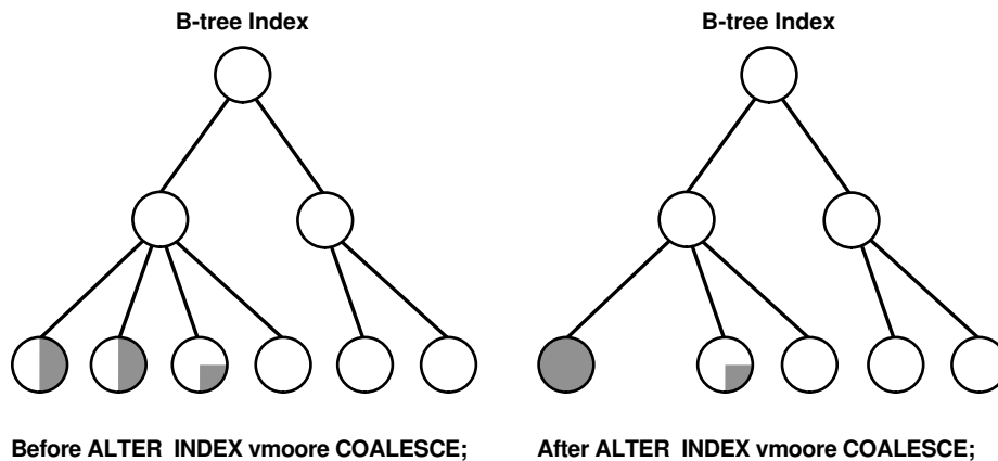
Figure 21-1 Coalescing Indexes
