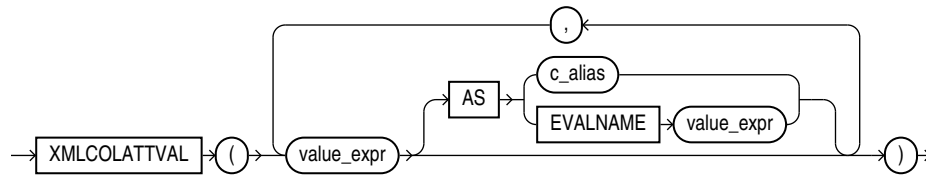
Figure 8-10 XMLCOLATTVAL Syntax
