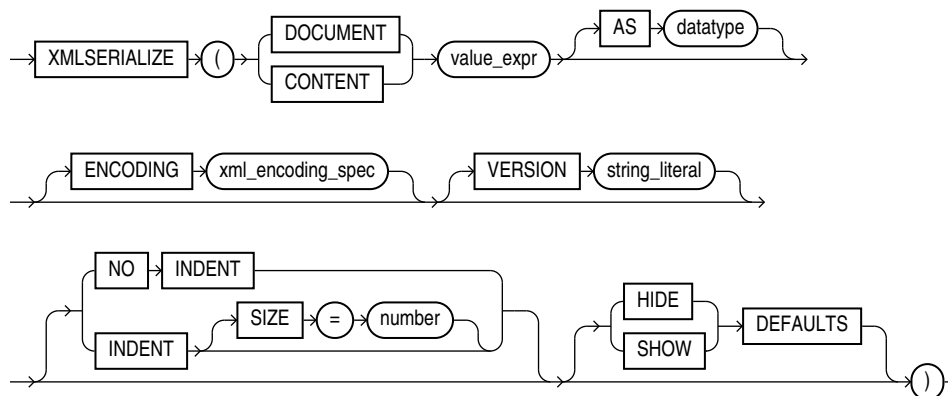
Figure 8-8 XMLSerialize Syntax
