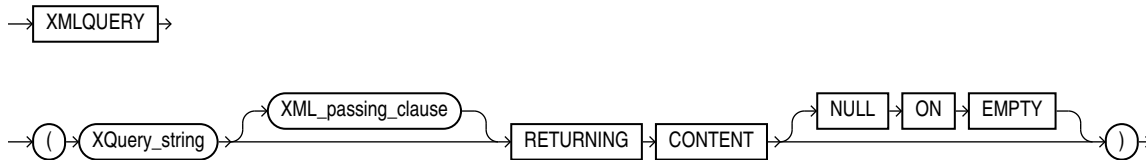
Figure 4-1 XMLQUERY Syntax
