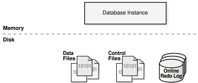
Figure 11-1 Database Instance and Database Files
