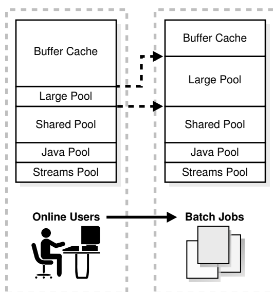
Figure 18-6 Automatic Memory Management
