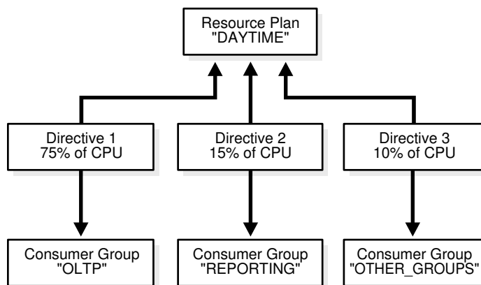
Figure 18-7 Simple Resource Plan
