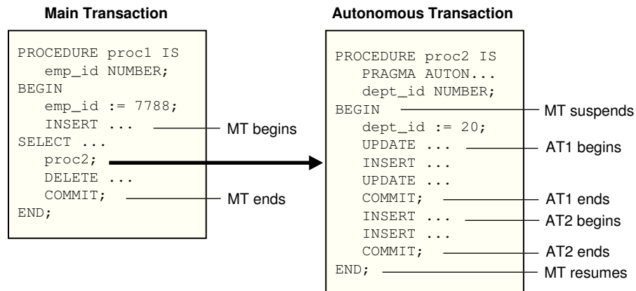
Figure 10-4 Transaction Control Flow
