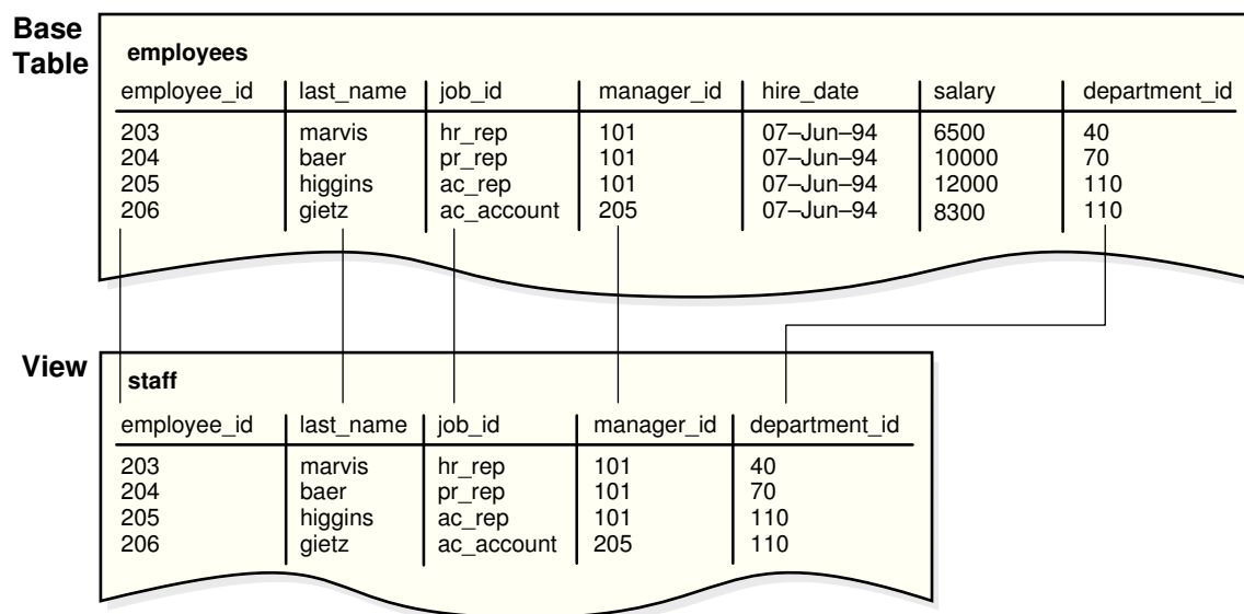
Figure 4-9 View
