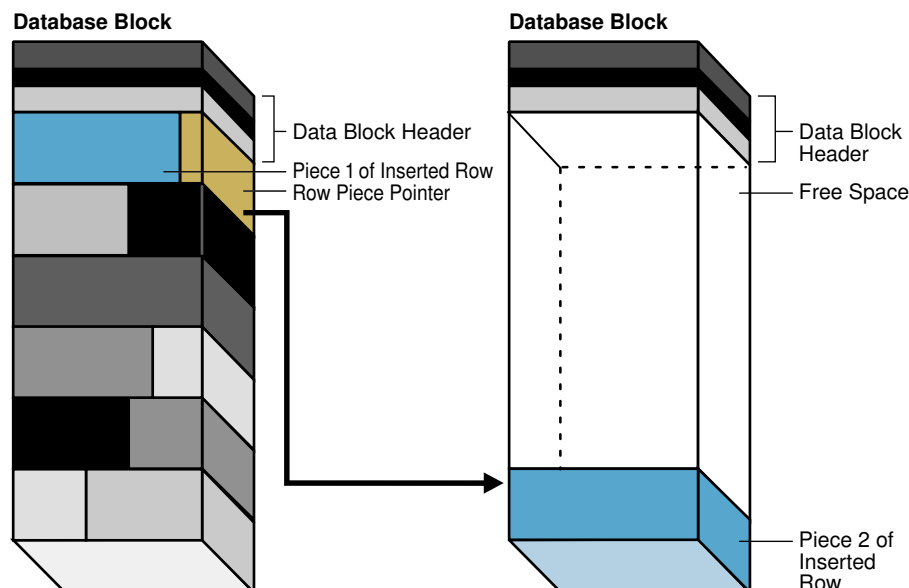
Figure 12-13 Row Chaining
