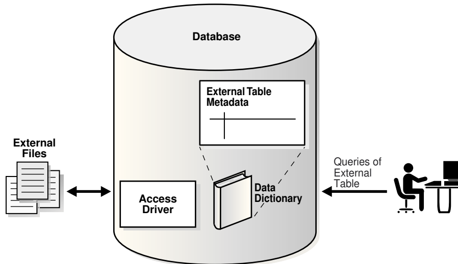
Figure 2-8 External Tables
