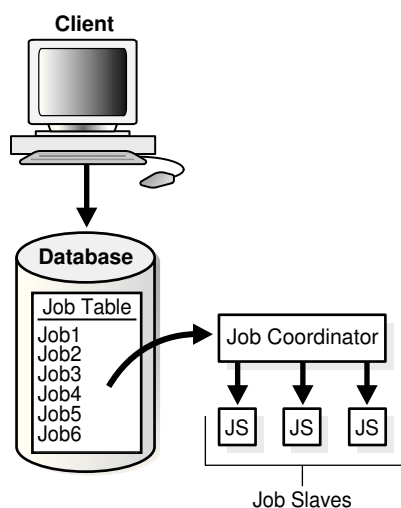
Figure 18-8 Scheduler Components
