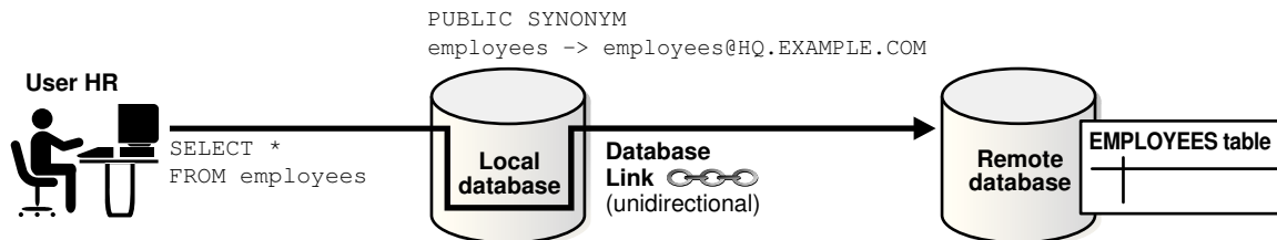
Figure 17-6 Database Link
