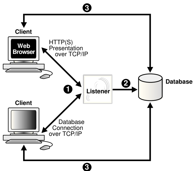
Figure 16-5 Listener Architecture
