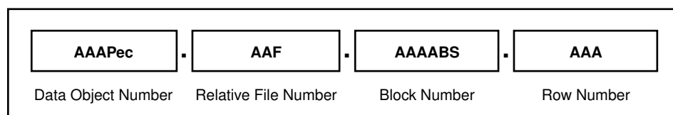
Figure 12-9 ROWID Format
