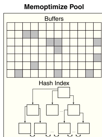
Figure 14-12 Memoptimize Pool
