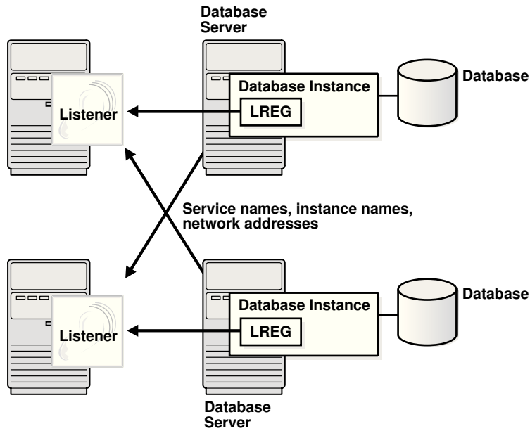
Figure 16-4 Two Listeners
