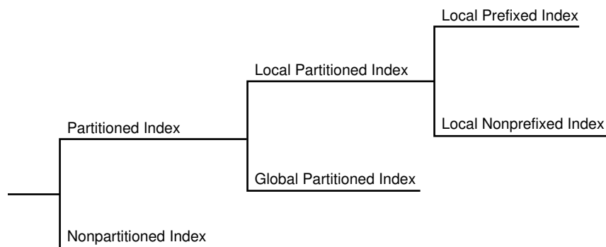
Figure 4-5 Index Partitioning Options
