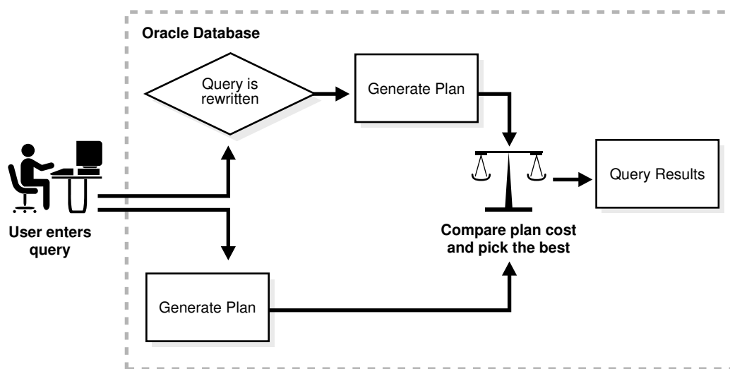
Figure 4-11 Query Rewrite
