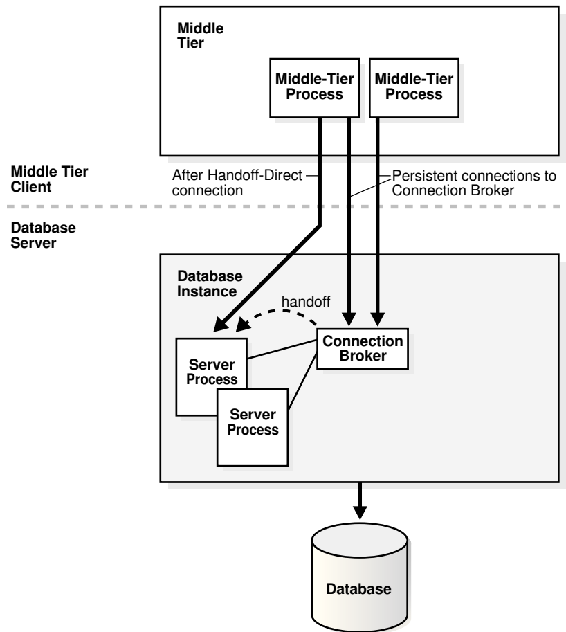
Figure 16-9 DRCP
