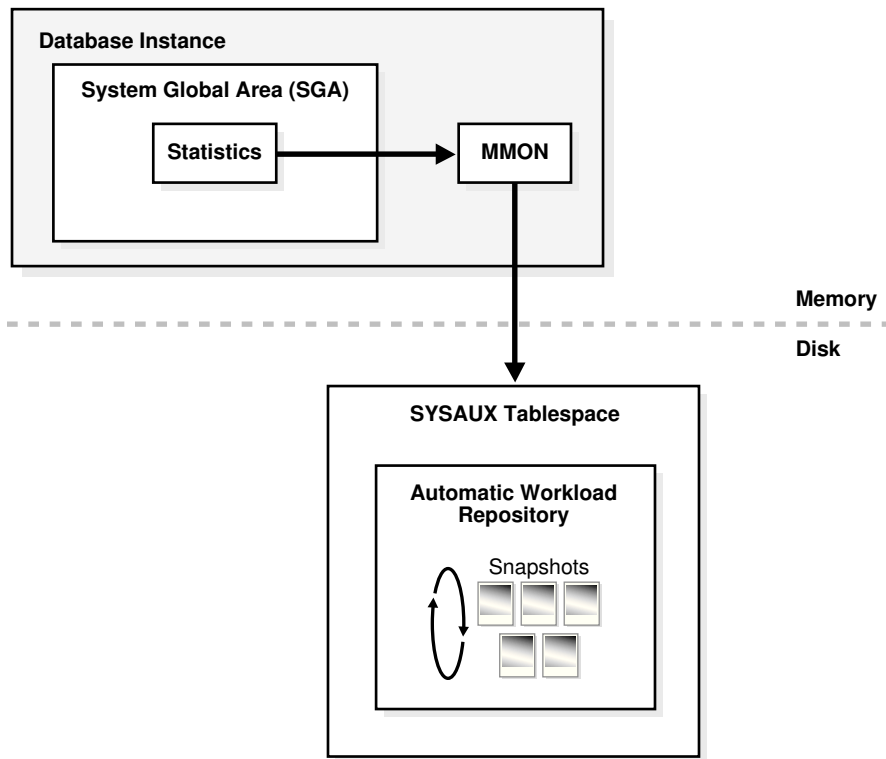
Figure 18-9 Automatic Workload Repository (AWR)
