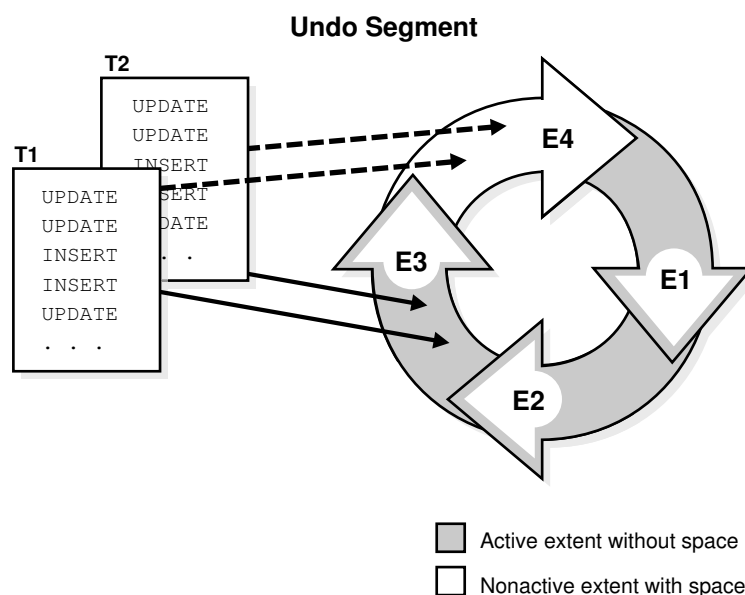
Figure 12-21 Ring of Allocated Extents in an Undo Segment
