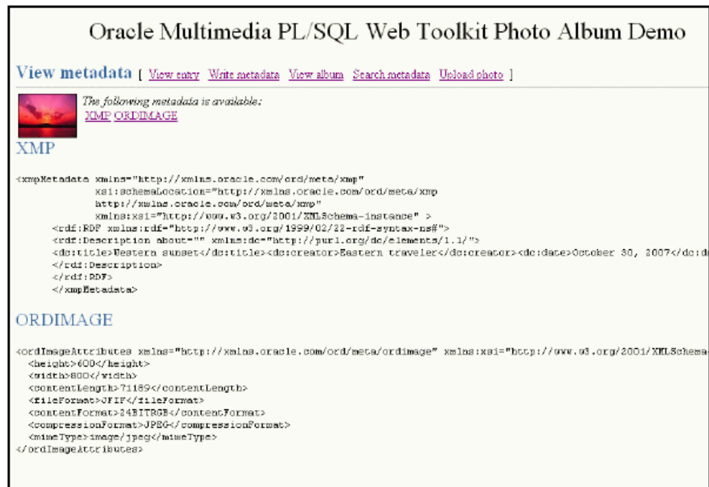
Figure 3-5 View metadata Page with Metadata for an Uploaded Image
