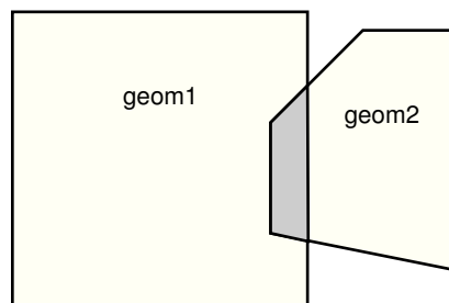
Figure 26-3 SDO_GEOM.SDO_INTERSECTION
