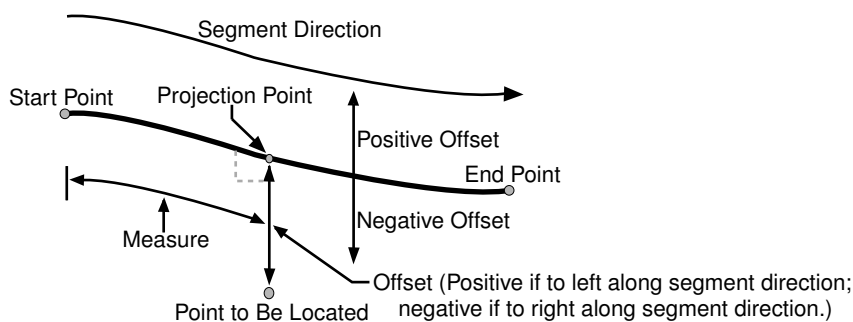
Figure 7-15 Locating a Point Along a Segment with a Measure and an Offset
