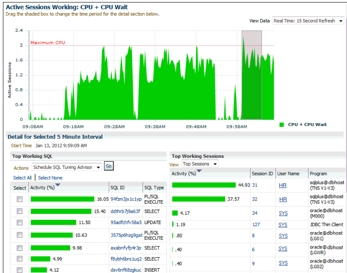
Figure 4-2 Active Sessions Working Page
