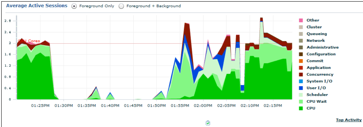
Figure 4-1 Average Active Sessions Chart
