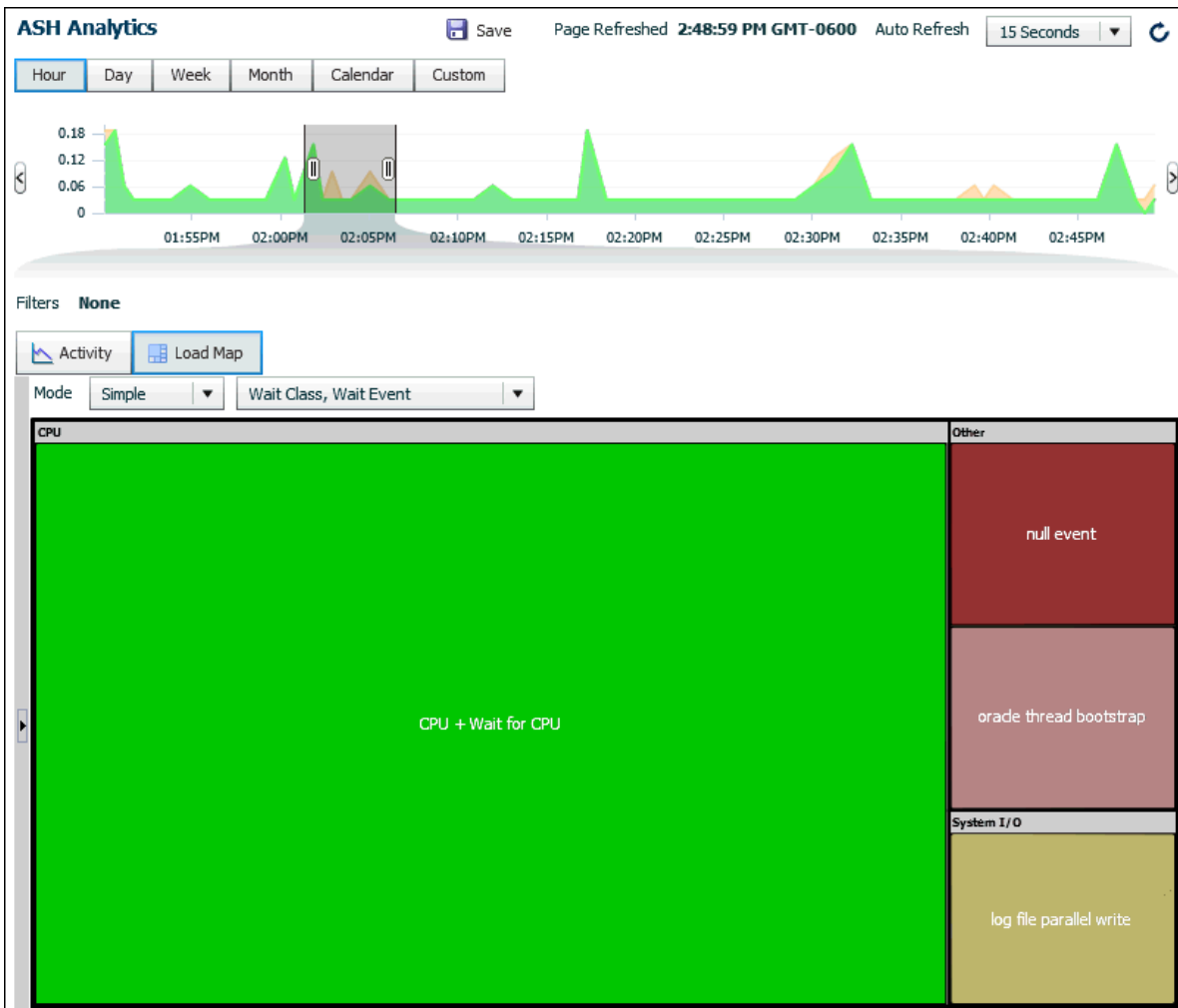
Figure 4-19 Load Map on the ASH Analytics Page
