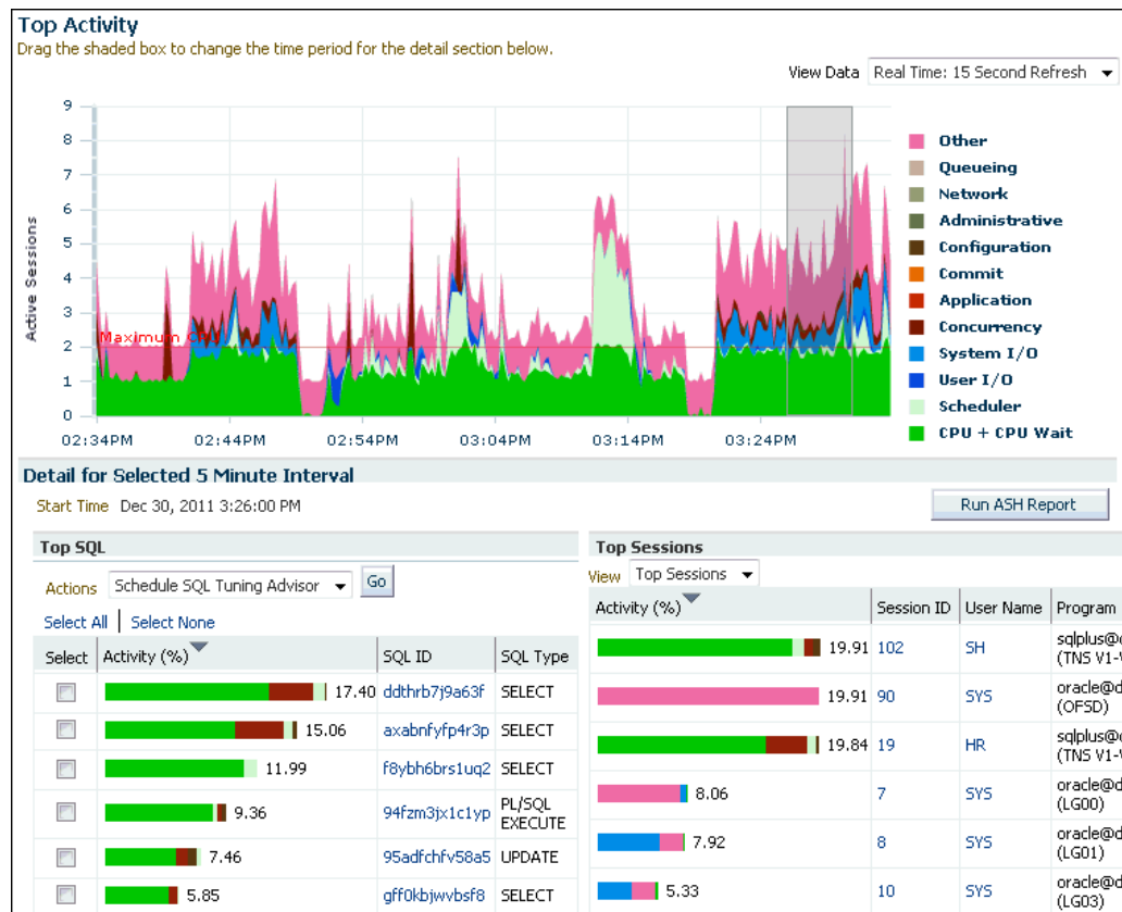
Figure 11-1 Top Activity Page
