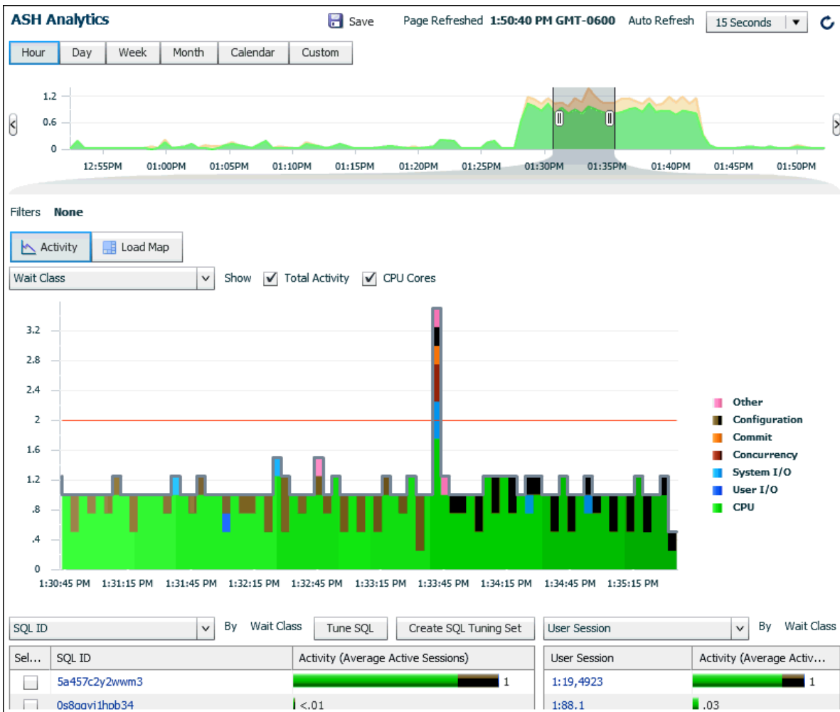
Figure 4-17 ASH Analytics Page
