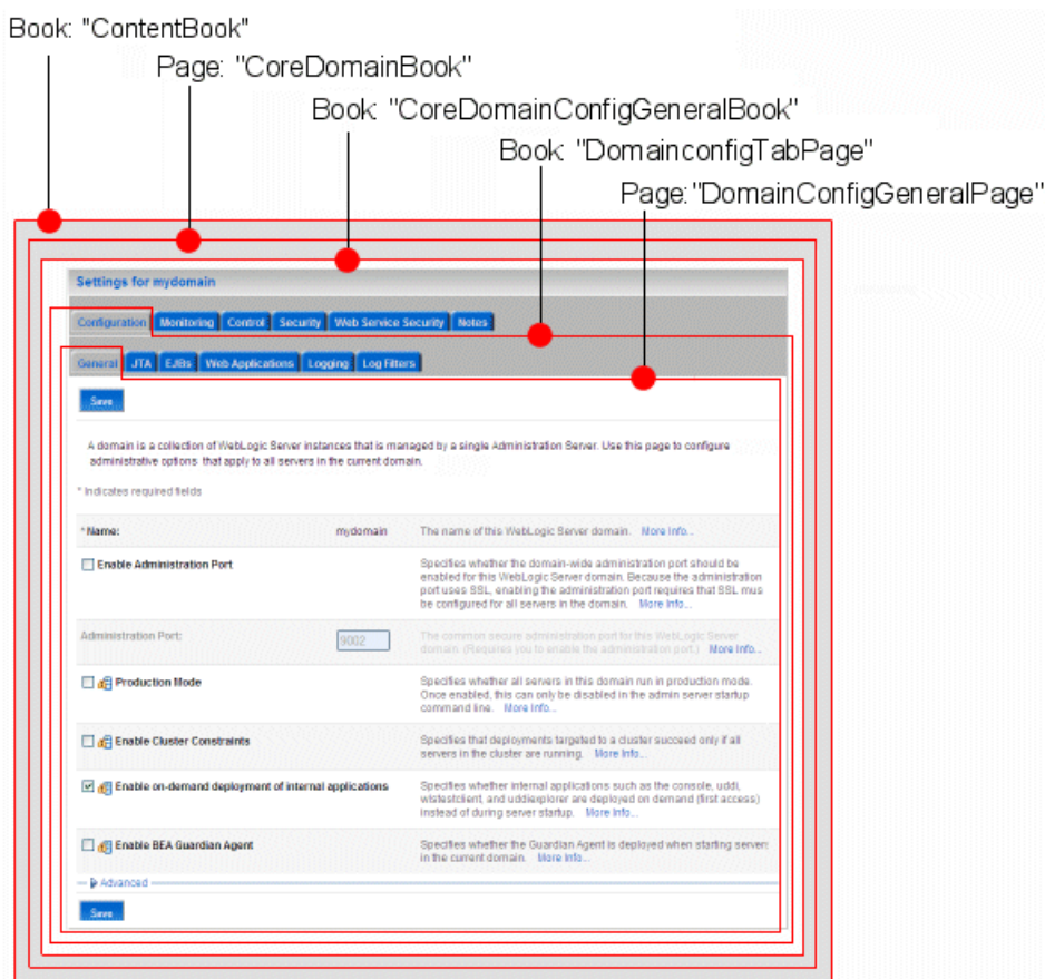
Figure 2-4 The ContentBook
