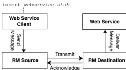
Figure 3-1 Web Service Reliable Message Exchange
