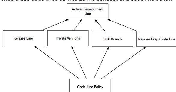
Figure 2: Code Line Patterns
