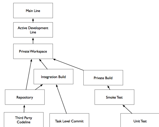
Figure 1: Workspace Patterns
